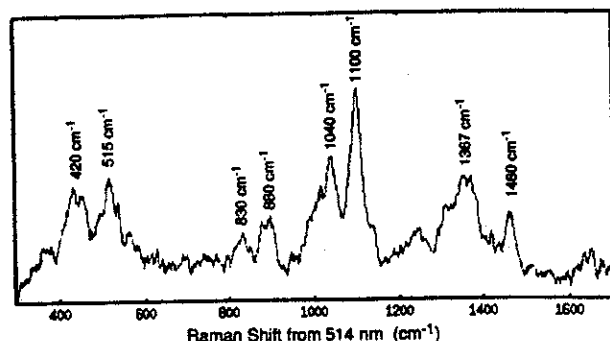
Fig. 5 Typical Raman spectrum for aqueous glucose. The Stokes Raman spectrum is shown as vibrational intensity vs shift in wave numbers from 514 nm excitation wavelength. The water background has been subtracted.
