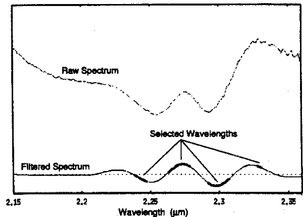
Fig. 8 Wavelength selection for NIR spectra. After Fourier filtering of the raw NIR absorption spectrum, an iterative wavelength selection algorithm determines wavelengths which are most useful for prediction. Adapted from Ref. 88.
