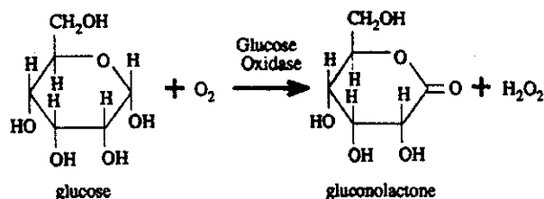
Fig. 6 The oxidation of glucose by glucose oxidase. Glucose and diatomic oxygen are consumed to form a gluconolactone and hydrogen peroxide.
