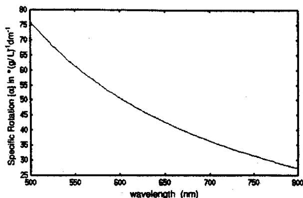
Fig. 2 Optical rotatory dispersion (ORD) curve for glucose. The specific rotation in ^\circ(\text{g/L})^{-1} \text{dm}^{-1} is shown vs wavelength in nm. Adapted from Ref. 39.
