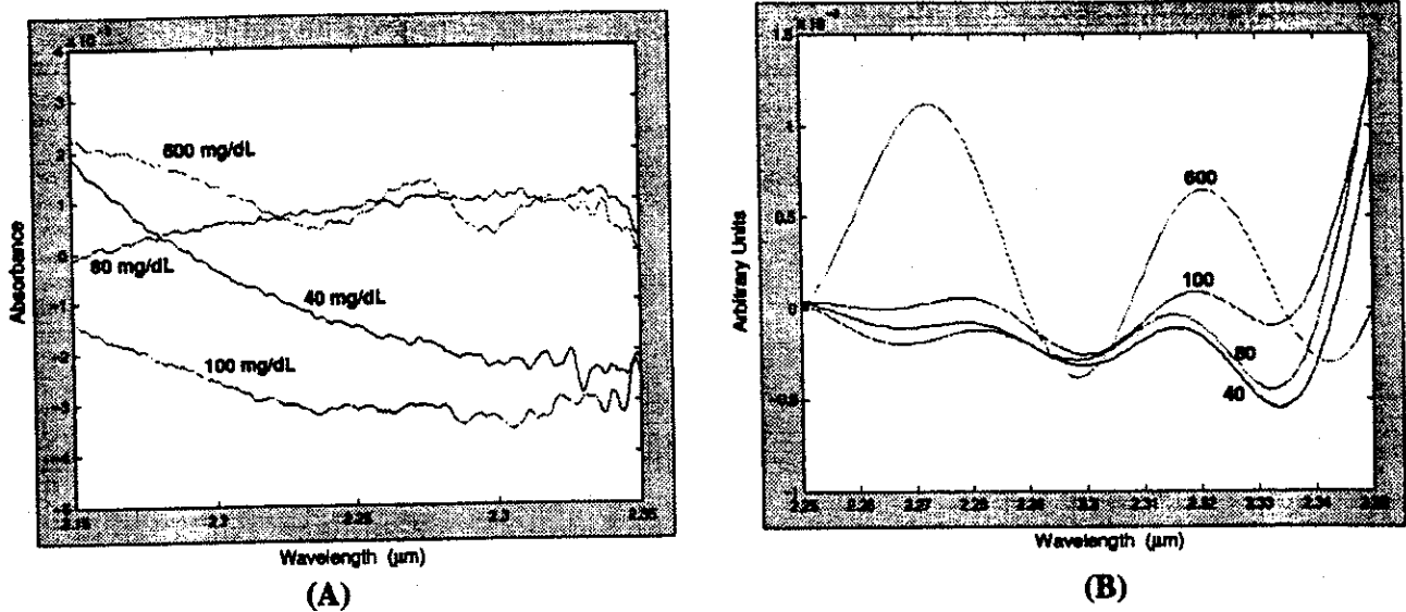
Fig. 7 NIR spectra of aqueous glucose solutions before (a) and after (b) application of Fourier filtering. The filter has the effect of enhancing glucose specific information by removing baseline offsets and high frequency noise. Adapted from Ref. 96.
