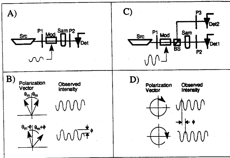
Fig. 3 Amplitude and phase based polarimetry measurements. (a) In the amplitude approach light from a monochromatic source (Src) is passed through a linear polarizer (P1), a polarization modulator (Mod), a sample (Sam), and a second linear polarizer perpendicular to the first (P2) before being recorded by a detector (Det). (b) The resulting polarization vector and observed intensity are symmetric when no optically active sample is present and asymmetric if the sample is optically active with net rotation \phi . (c) In the phase approach, polarization modulated sample and reference beams are split by a beam splitter (BS), passed through crossed linear polarizers (P2, P3), and recorded by separate detectors (Det1, Det2). (d) A rotation of polarization by the sample causes a phase shift between the intensity signals recorded by the two detectors.
