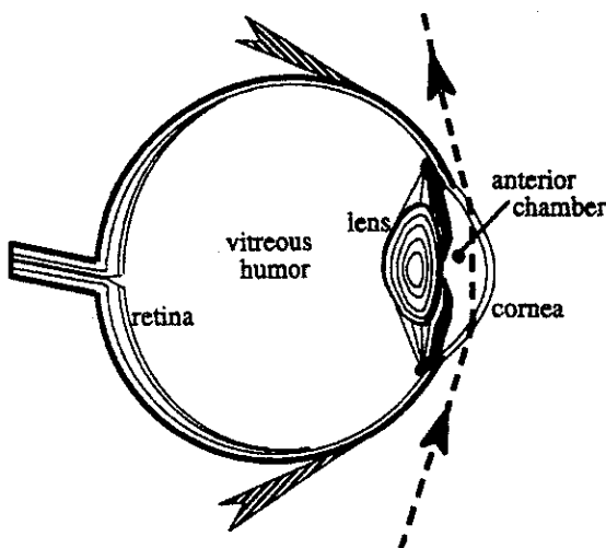
Fig. 4 Optical sensing in the anterior chamber of the eye. Light passing through the anterior chamber of the eye interacts with the aqueous humor. A commonly proposed beam path is shown.
