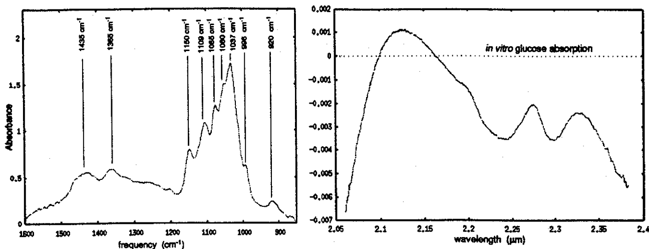
Fig. 1 Optical absorption spectra for glucose. (a) Midinfrared region extending from 1600 to 900 \text{cm}^{-1} or 6.25 to 11 \mu\text{m} and showing absorption peak assignments. (b) Near-infrared region extending from 2.0 to 2.5 \mu\text{m} or 5000 to 4000 \text{cm}^{-1} . Note that the magnitude of the three absorbance peaks in the NIR region is much smaller.
