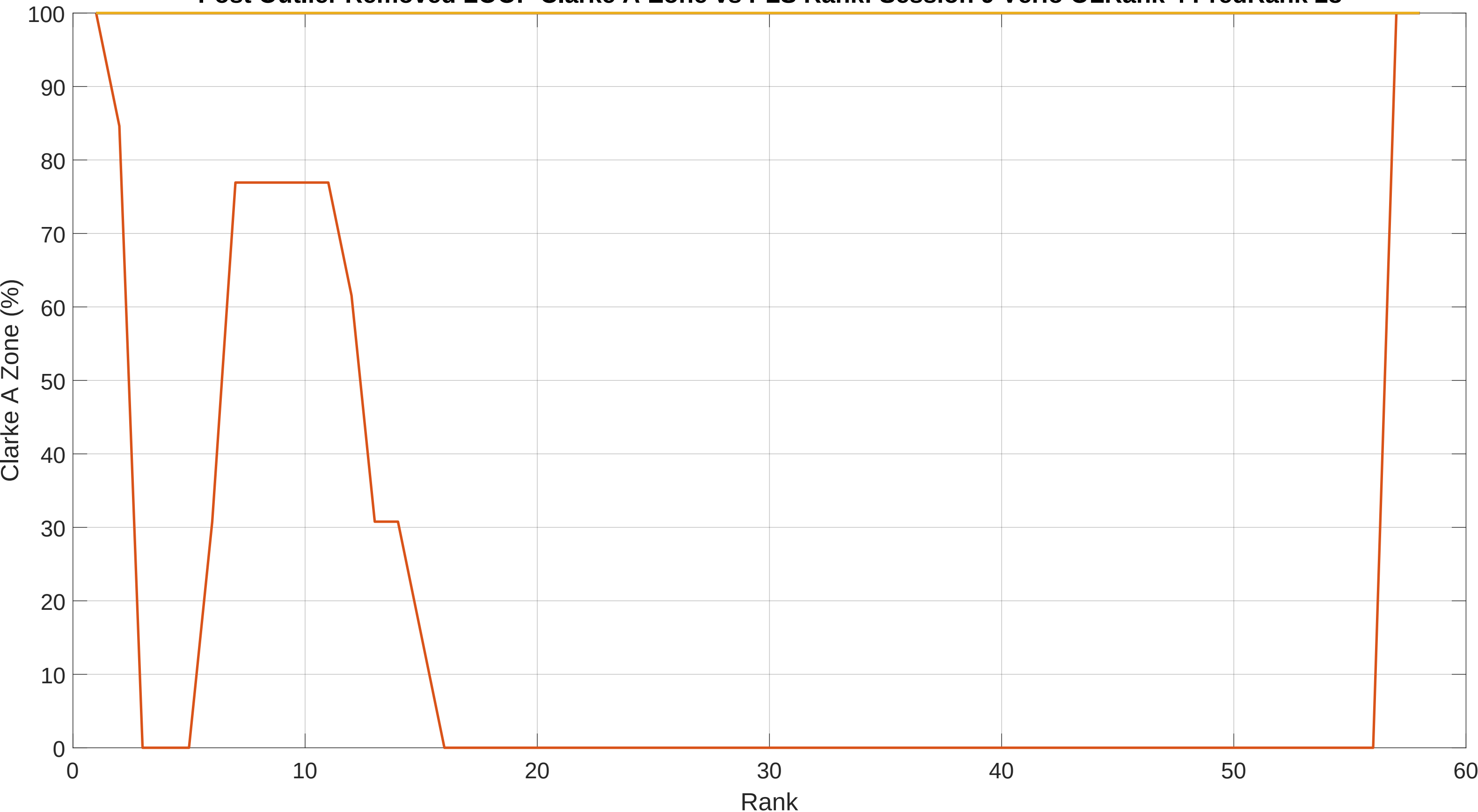
Post Outlier Removed LOOP Clarke A-Zone vs PLS Rank: Session 9 Verio OLRank 4 PredRank 28
