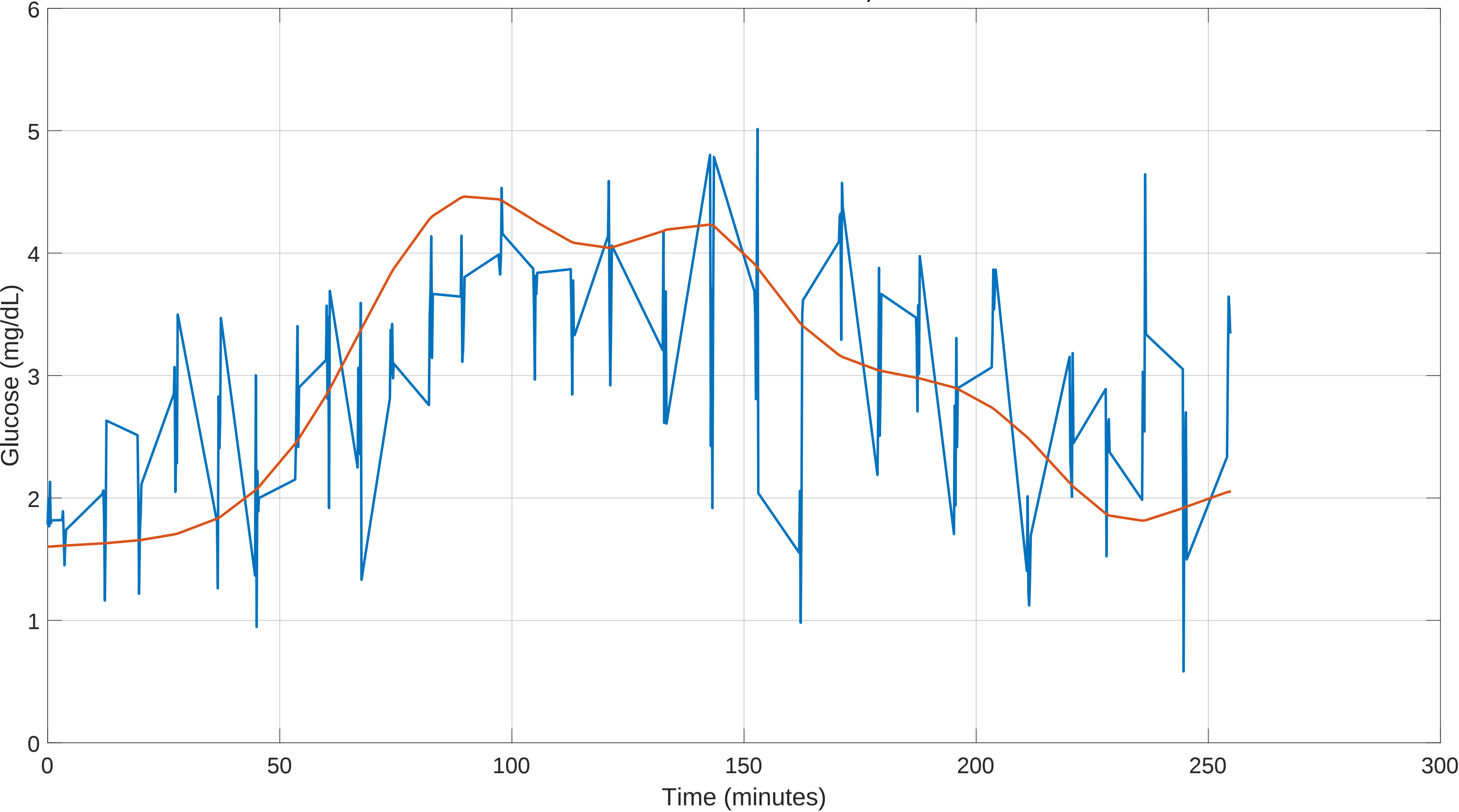
Post Outlier Removed LOOP vs Time: Outliers in Predictions, Session 6 Ultra OLRank 8 PredRank 28
