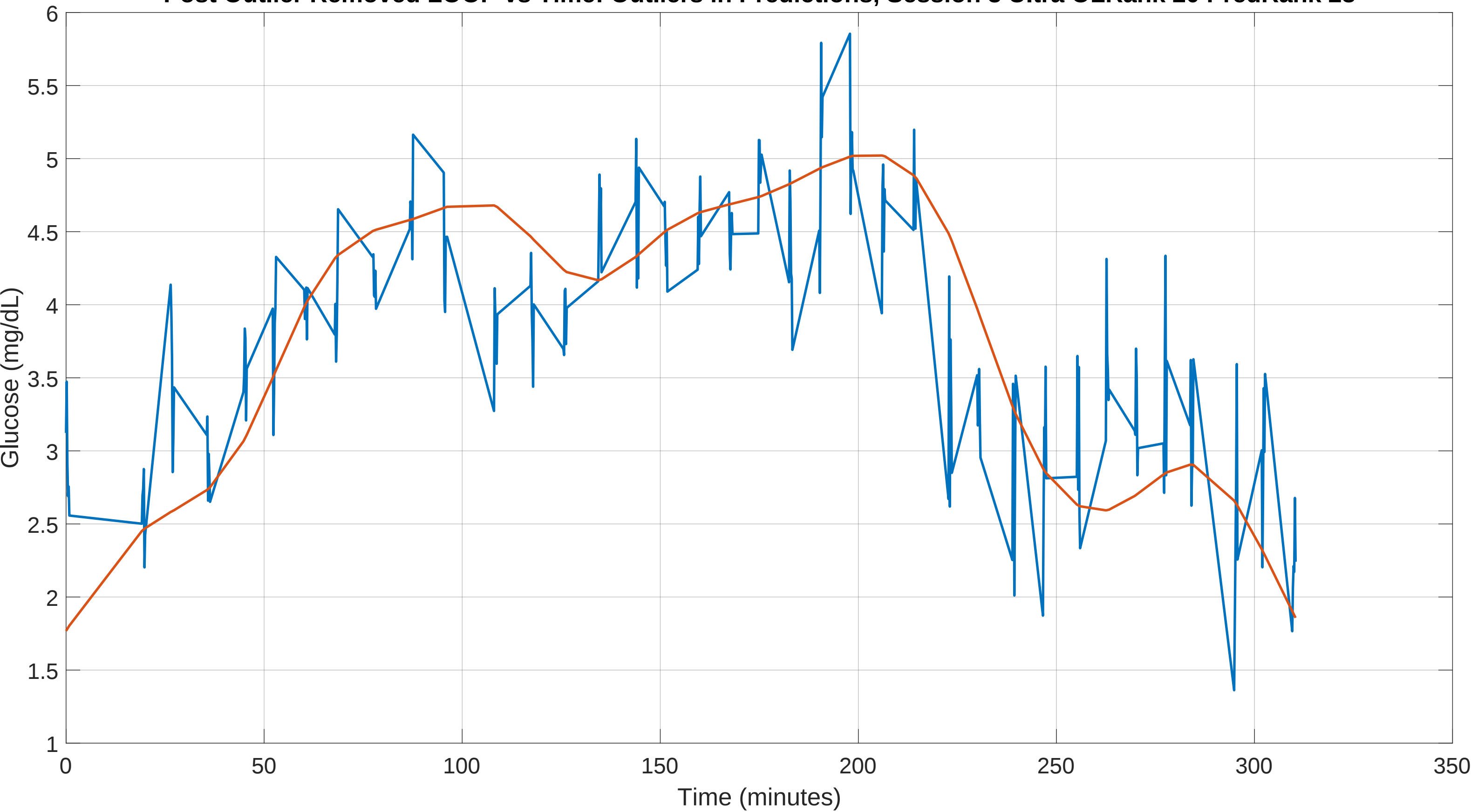
Post Outlier Removed LOOP vs Time: Outliers in Predictions, Session 3 Ultra OLRank 20 PredRank 28
