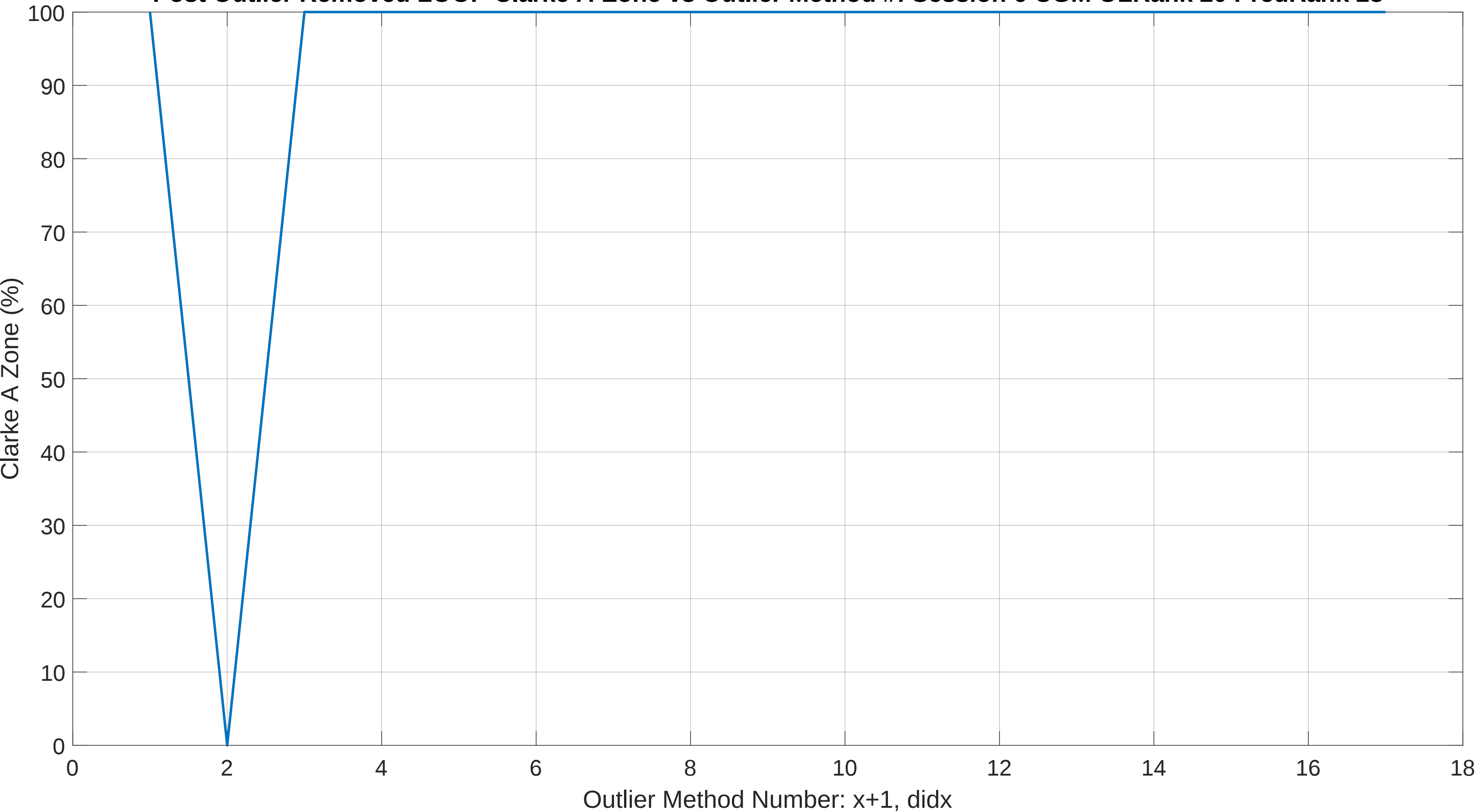
Post Outlier Removed LOOP Clarke A-Zone vs Outlier Method #: Session 6 CGM OLRank 20 PredRank 28
