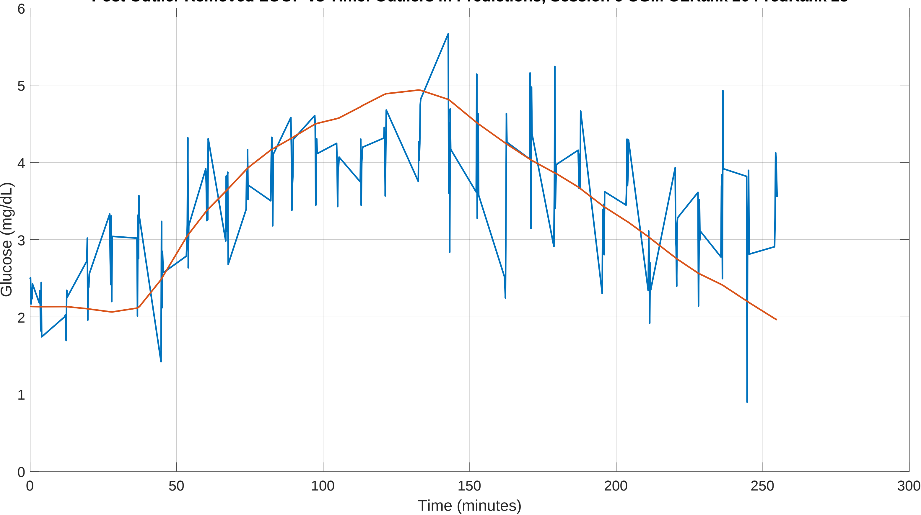
Post Outlier Removed LOOP vs Time: Outliers in Predictions, Session 6 CGM OLRank 20 PredRank 28
