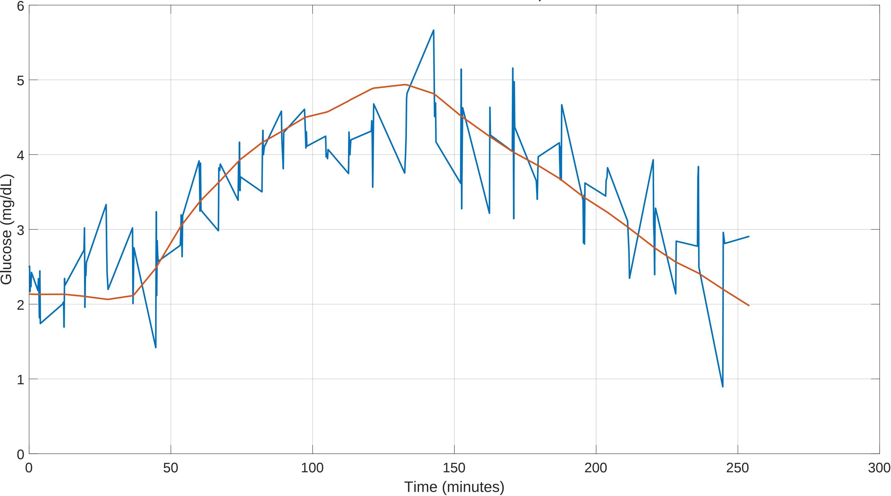
Post Outlier Removed LOOP vs Time: Outliers not in Predictions, Session 6 CGM OLRank 20 PredRank 28
