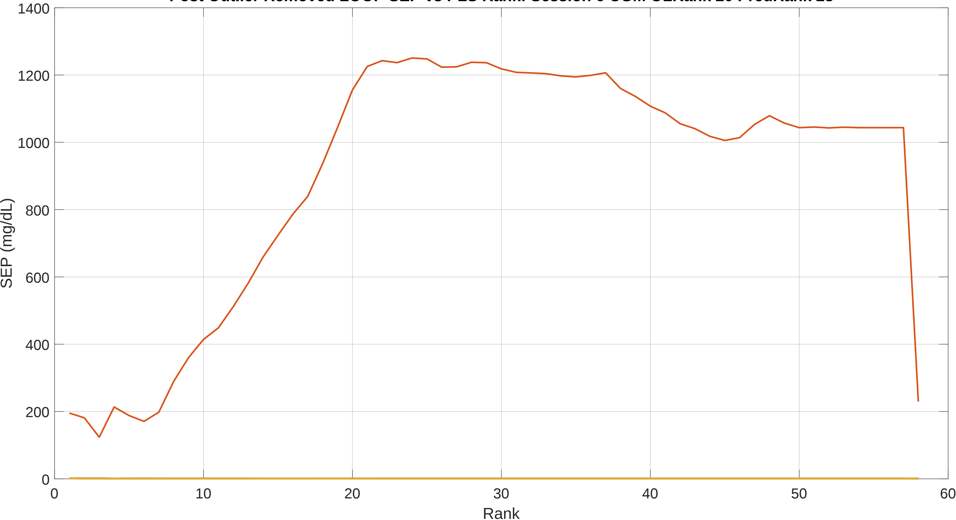
Post Outlier Removed LOOP SEP vs PLS Rank: Session 6 CGM OLRank 20 PredRank 28
