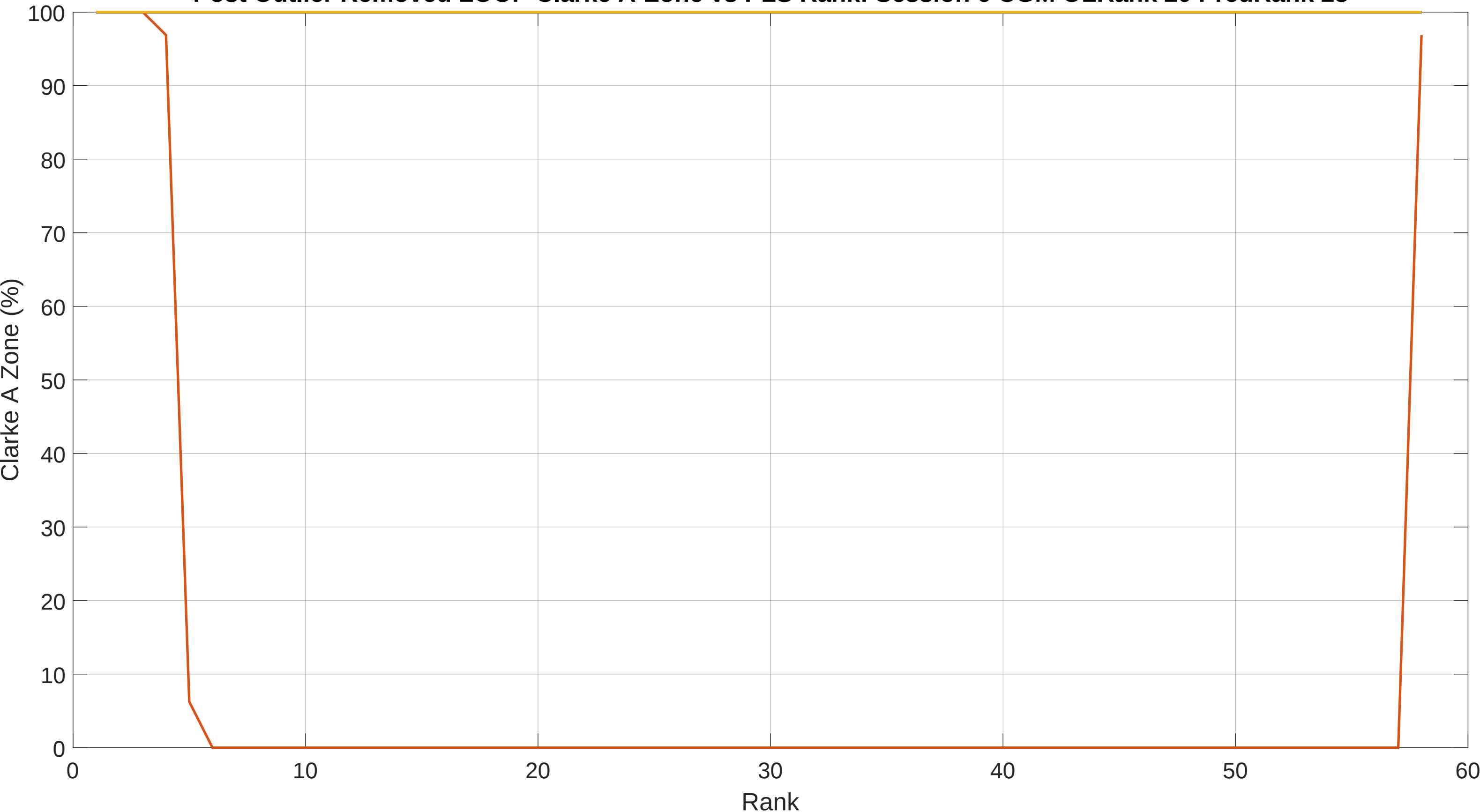
Post Outlier Removed LOOP Clarke A-Zone vs PLS Rank: Session 6 CGM OLRank 20 PredRank 28
