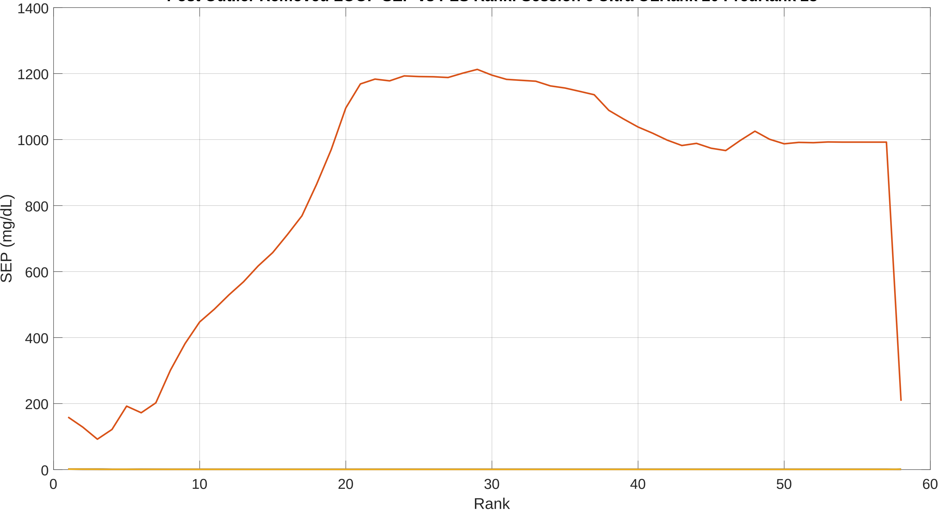
Post Outlier Removed LOOP SEP vs PLS Rank: Session 6 Ultra OLRank 20 PredRank 28
