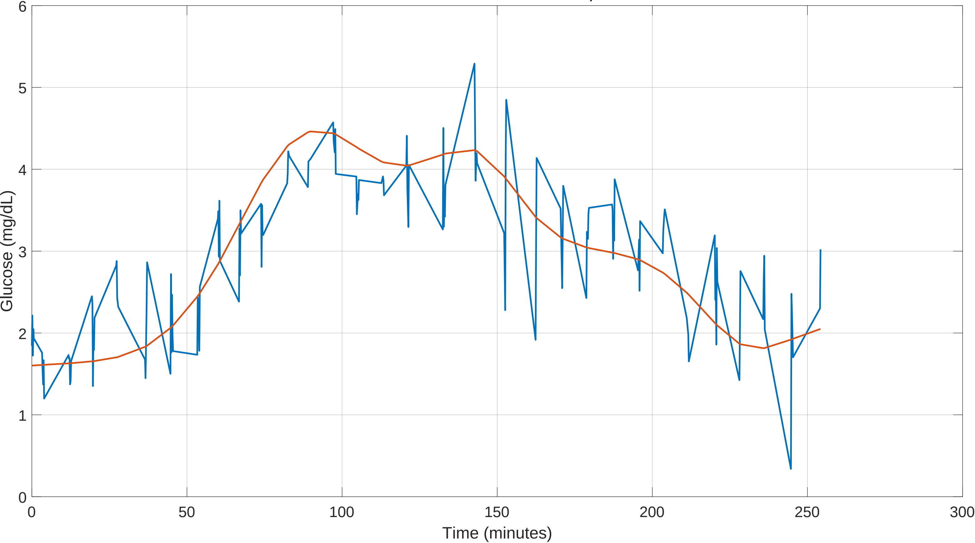
Post Outlier Removed LOOP vs Time: Outliers not in Predictions, Session 6 Ultra OLRank 20 PredRank 28
