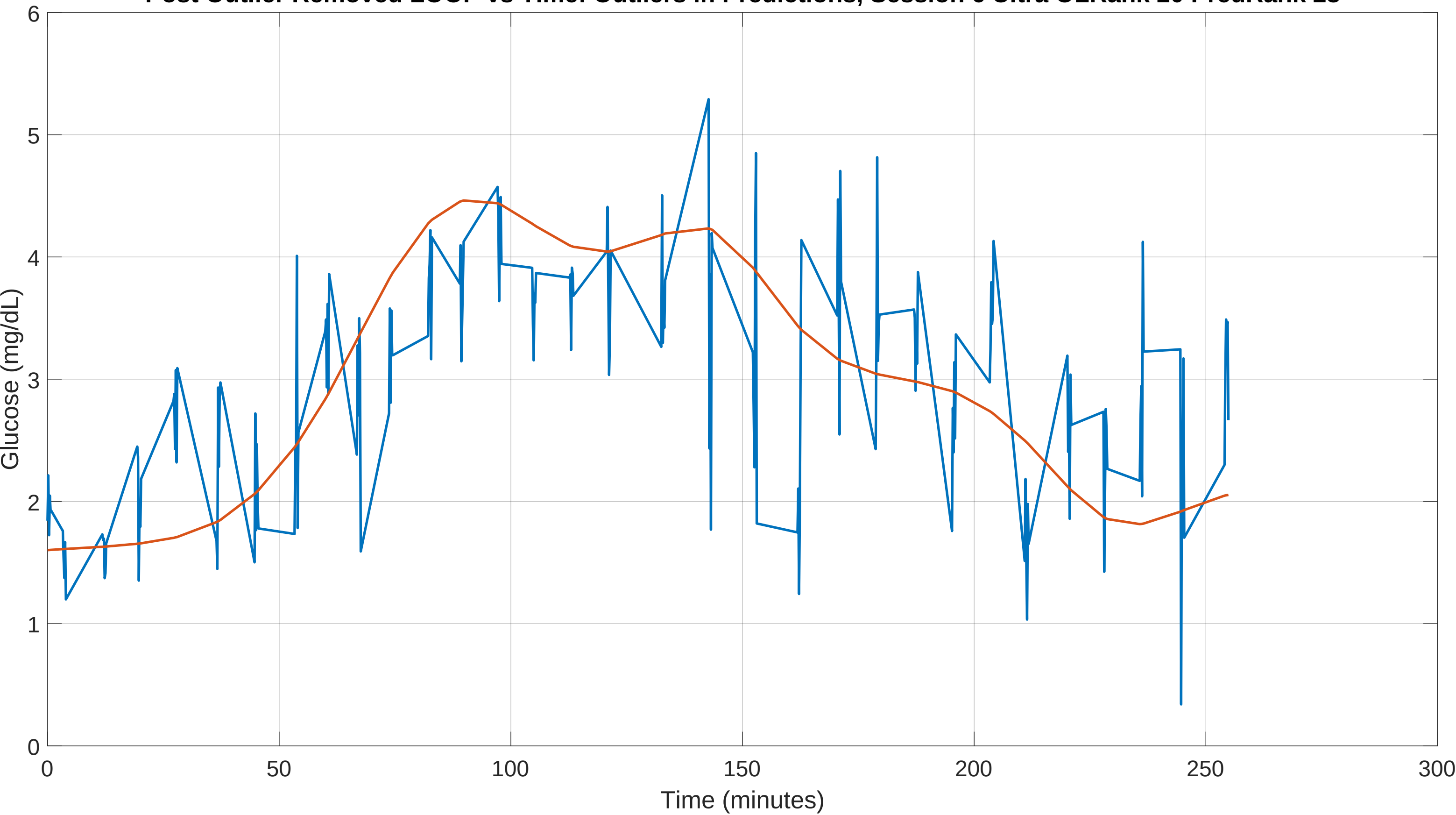
Post Outlier Removed LOOP vs Time: Outliers in Predictions, Session 6 Ultra OLRank 20 PredRank 28
