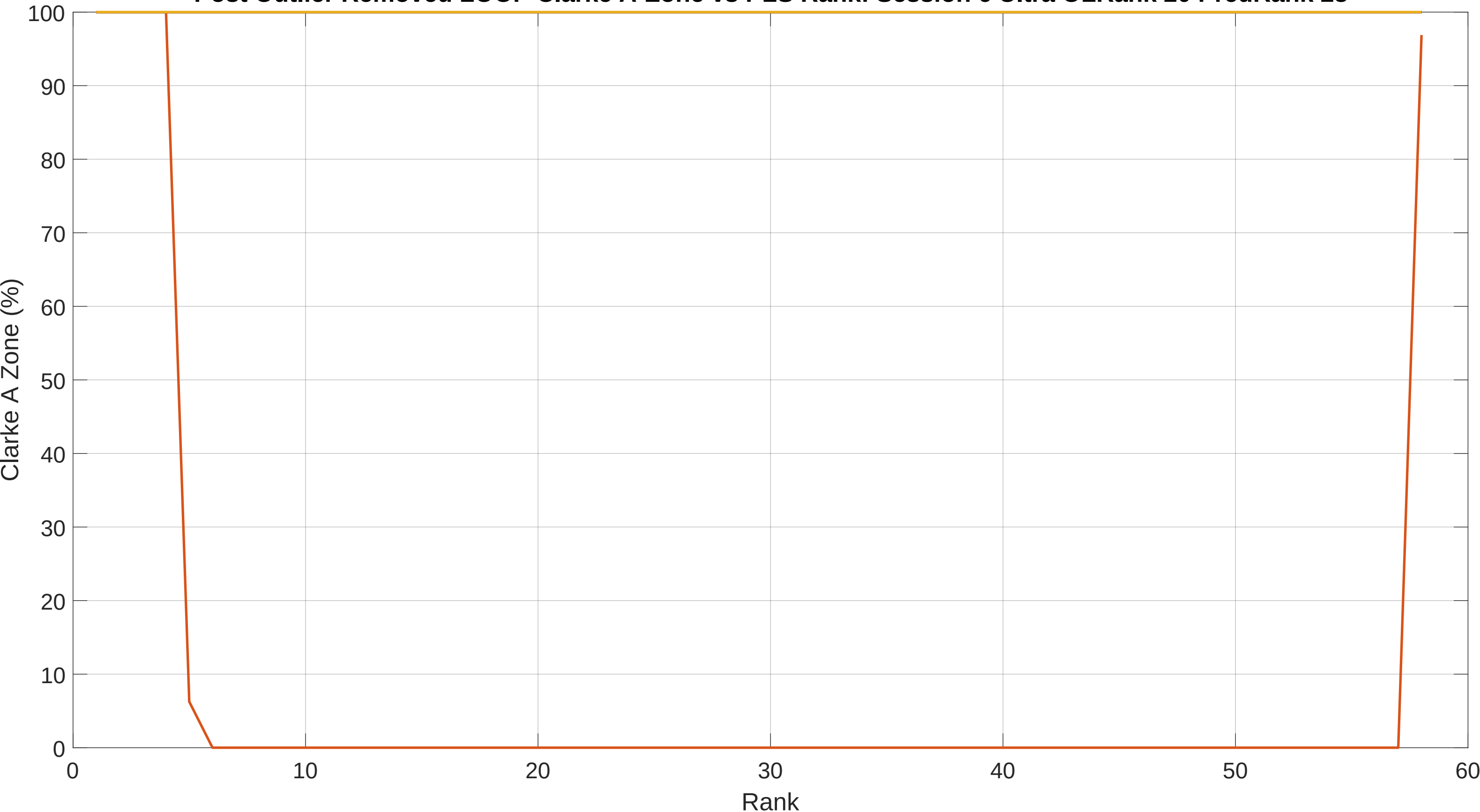
Post Outlier Removed LOOP Clarke A-Zone vs PLS Rank: Session 6 Ultra OLRank 20 PredRank 28
