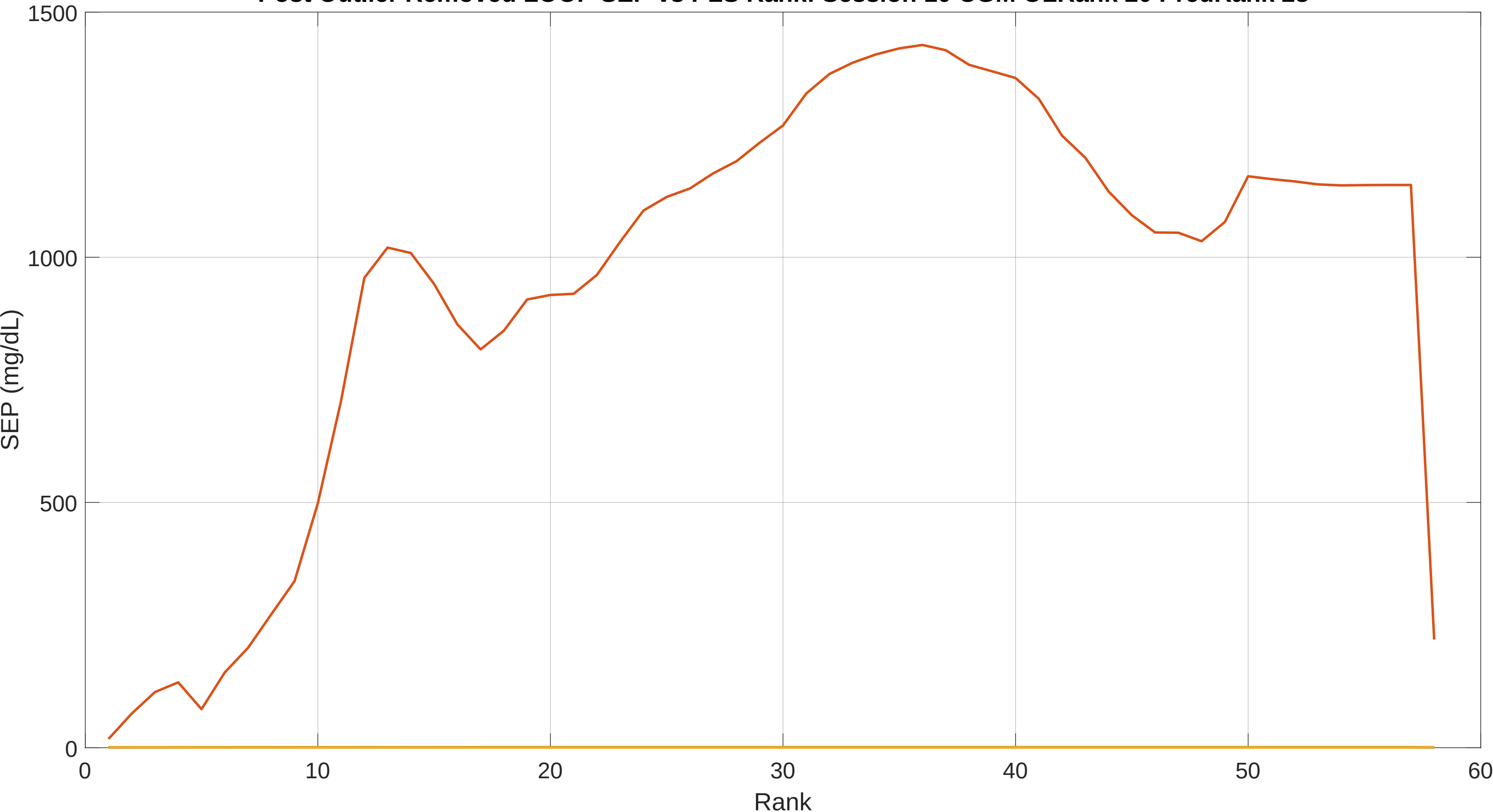
Post Outlier Removed LOOP SEP vs PLS Rank: Session 10 CGM OLRank 20 PredRank 28
