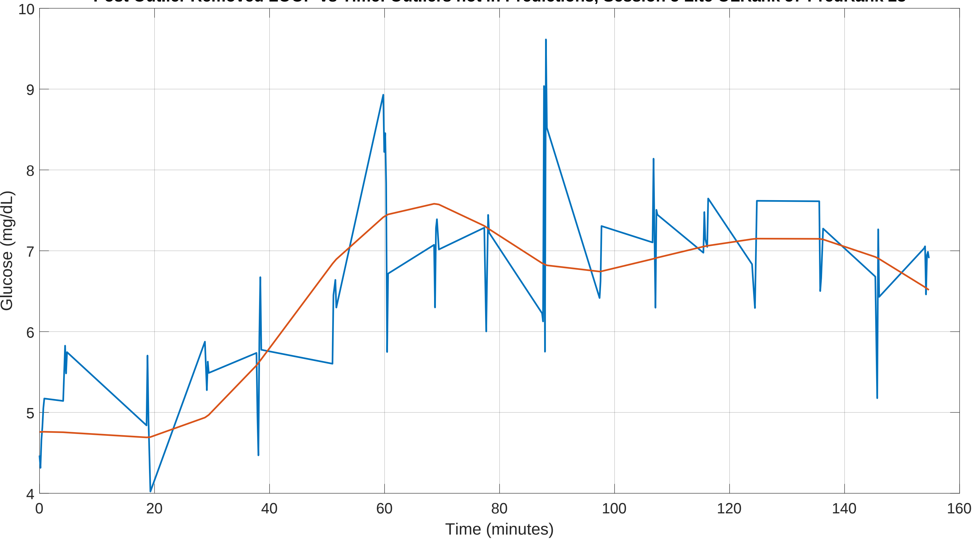
Post Outlier Removed LOOP vs Time: Outliers not in Predictions, Session 5 Lite OLRank 57 PredRank 28
