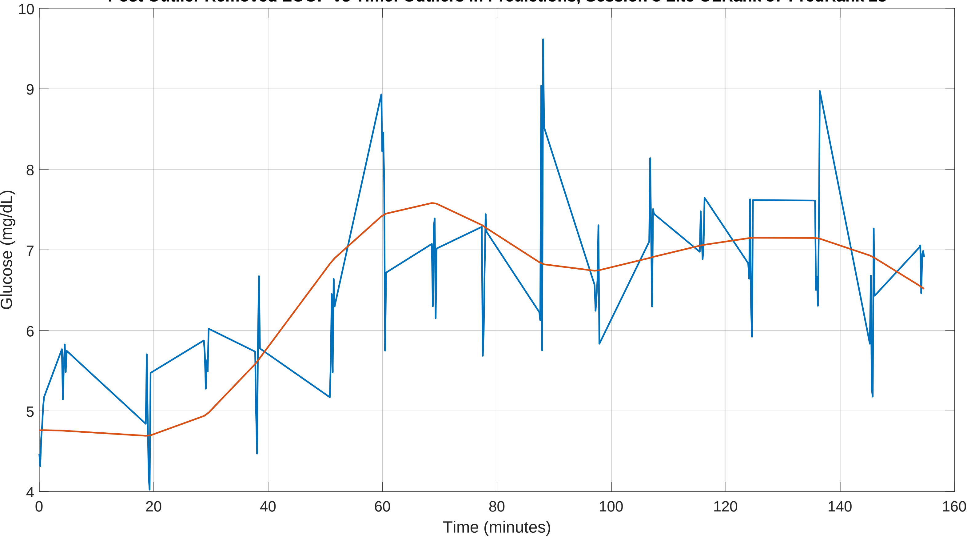
Post Outlier Removed LOOP vs Time: Outliers in Predictions, Session 5 Lite OLRank 57 PredRank 28
