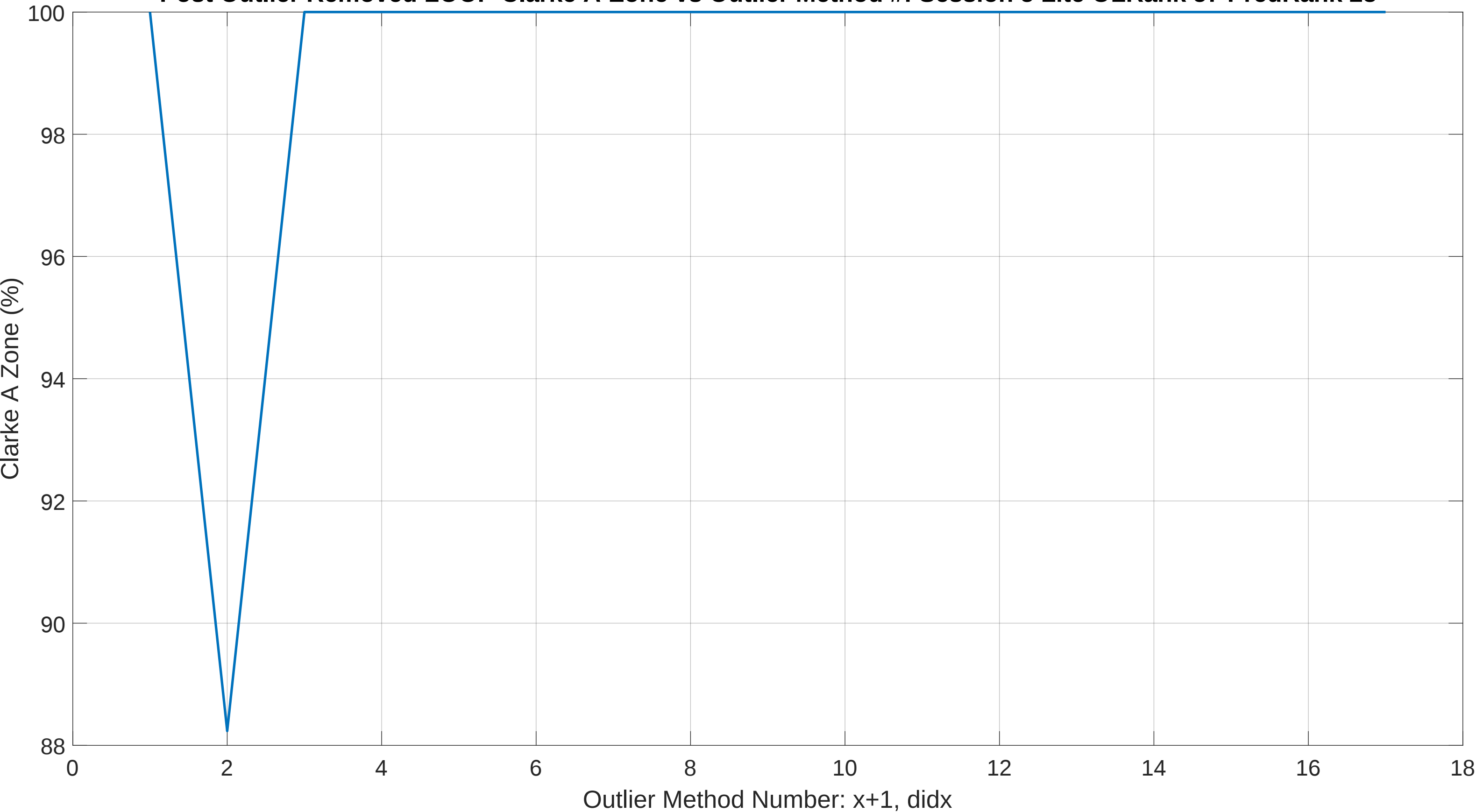
Post Outlier Removed LOOP Clarke A-Zone vs Outlier Method #: Session 5 Lite OLRank 57 PredRank 28
