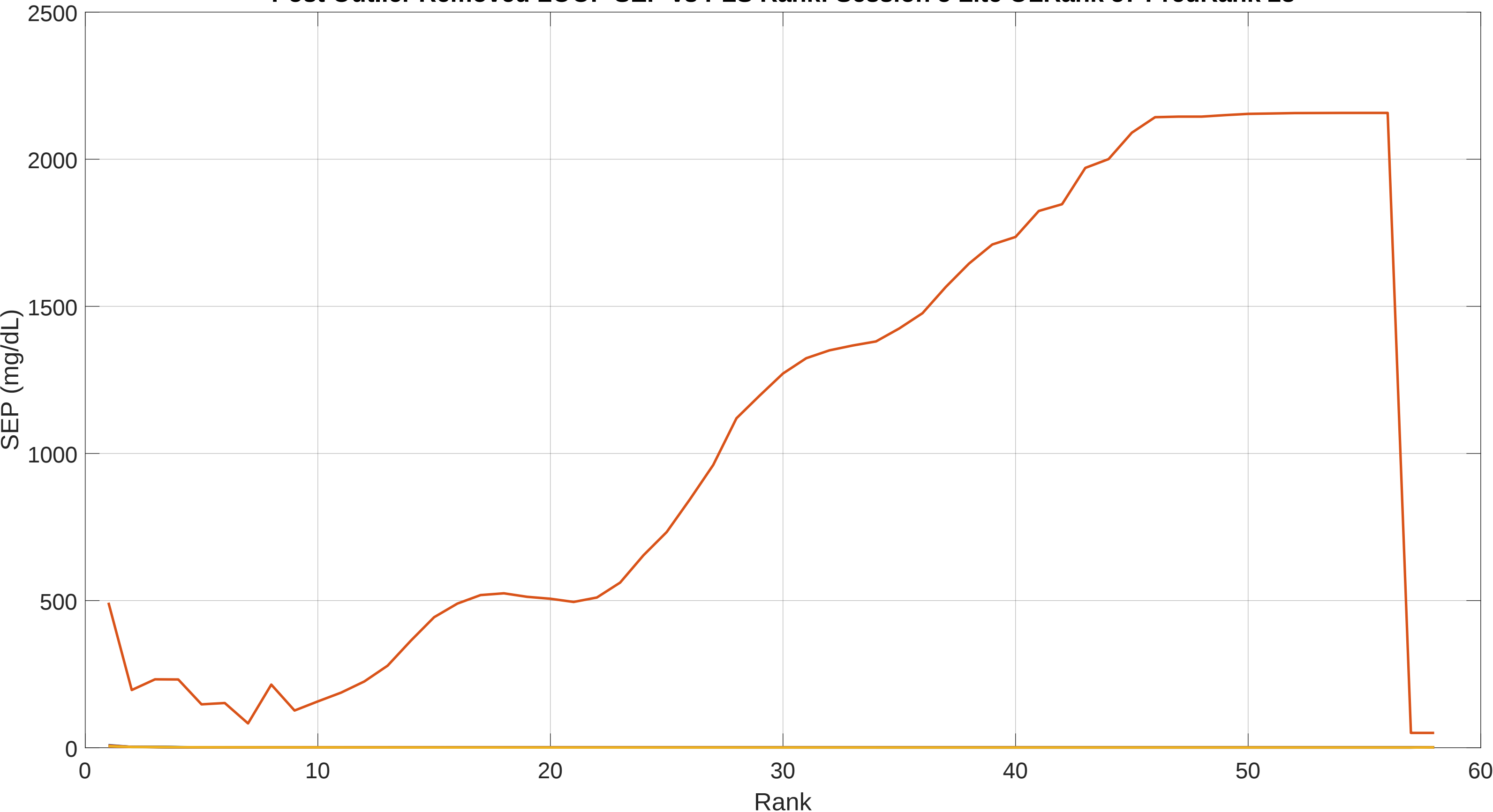
Post Outlier Removed LOOP SEP vs PLS Rank: Session 5 Lite OLRank 57 PredRank 28
