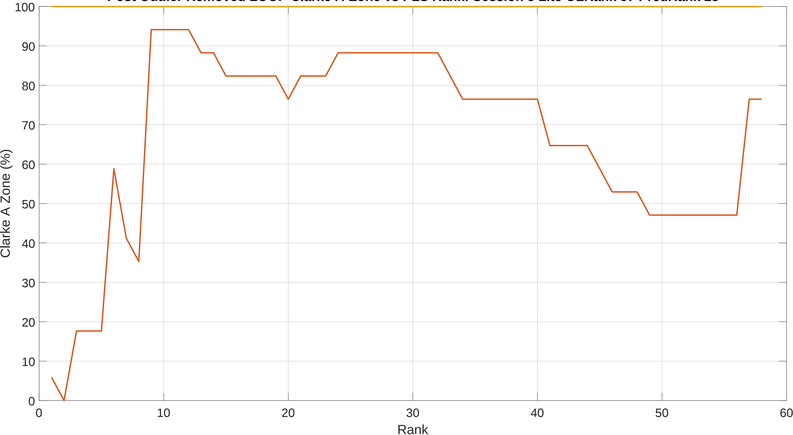
Post Outlier Removed LOOP Clarke A-Zone vs PLS Rank: Session 5 Lite OLRank 57 PredRank 28
