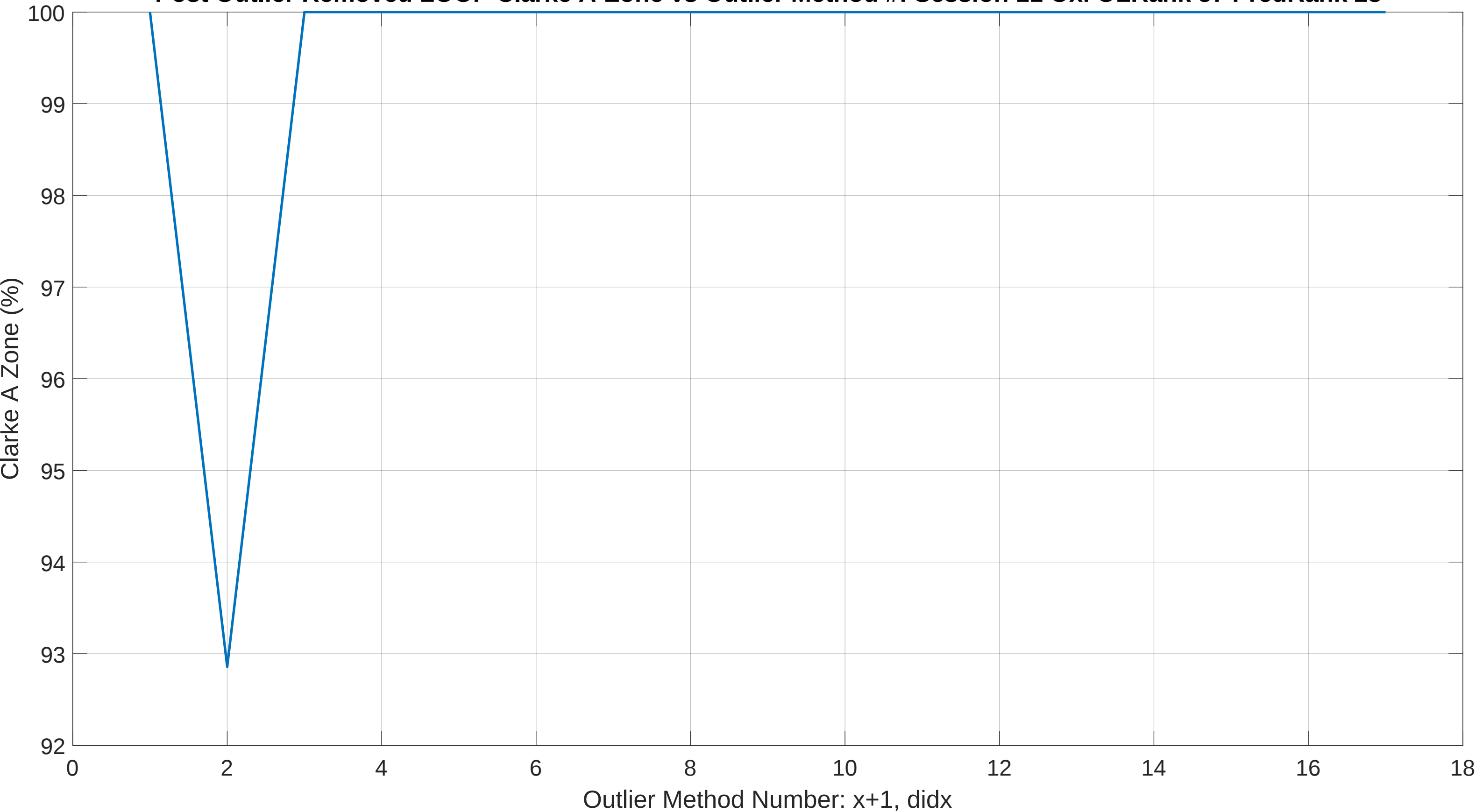
Post Outlier Removed LOOP Clarke A-Zone vs Outlier Method #: Session 11 Oxi OLRank 57 PredRank 28
