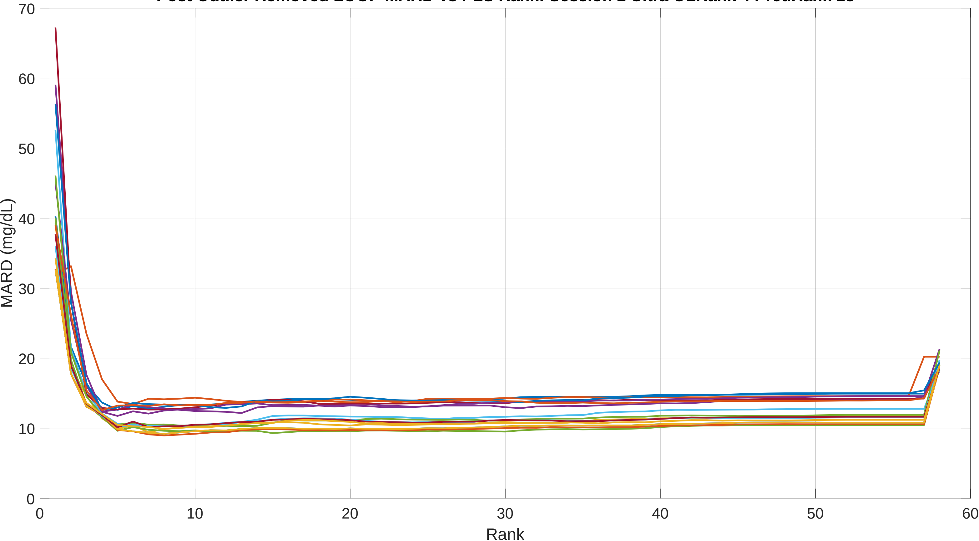
Post Outlier Removed LOOP MARD vs PLS Rank: Session 2 Ultra OLRank 4 PredRank 28
