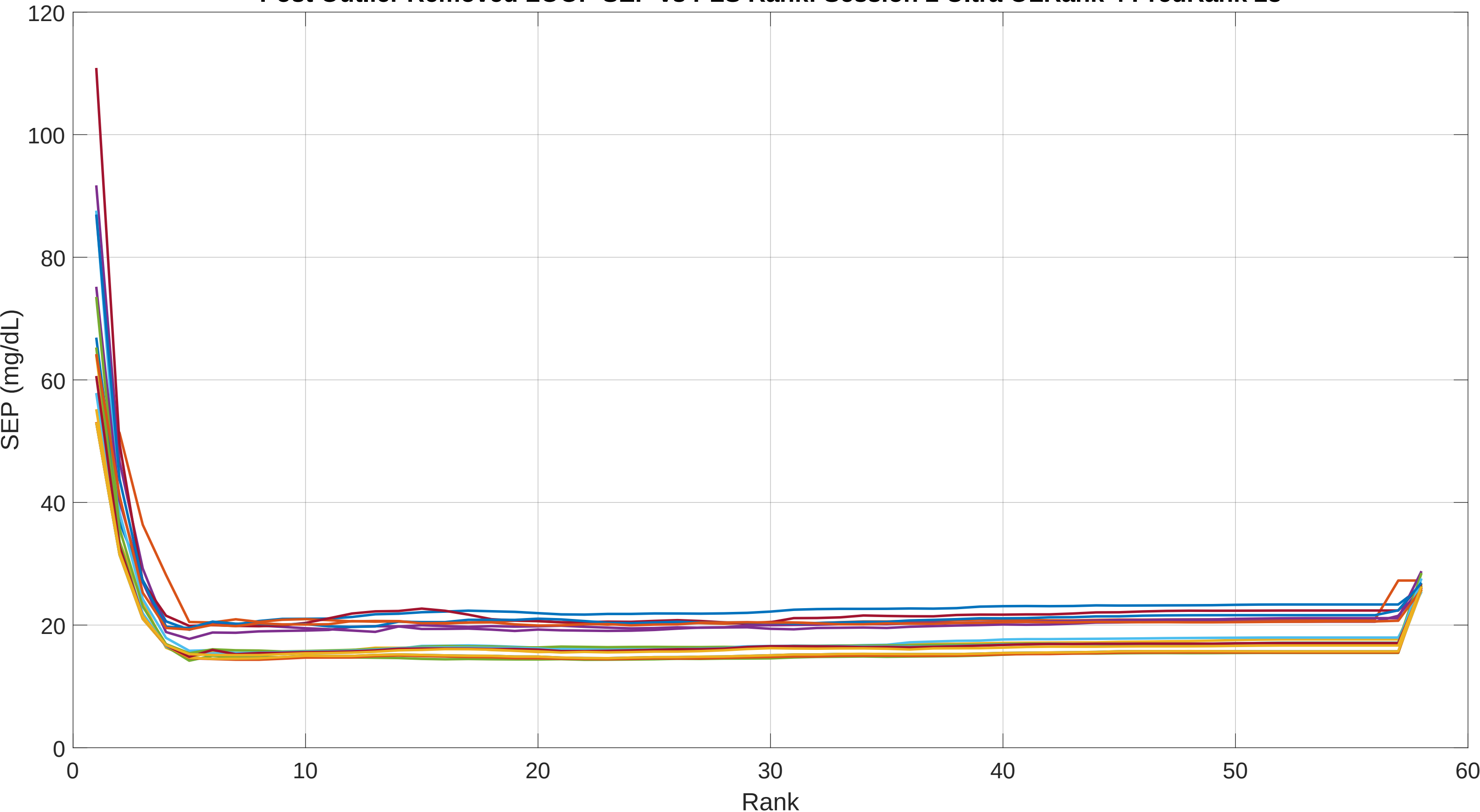
Post Outlier Removed LOOP SEP vs PLS Rank: Session 2 Ultra OLRank 4 PredRank 28
