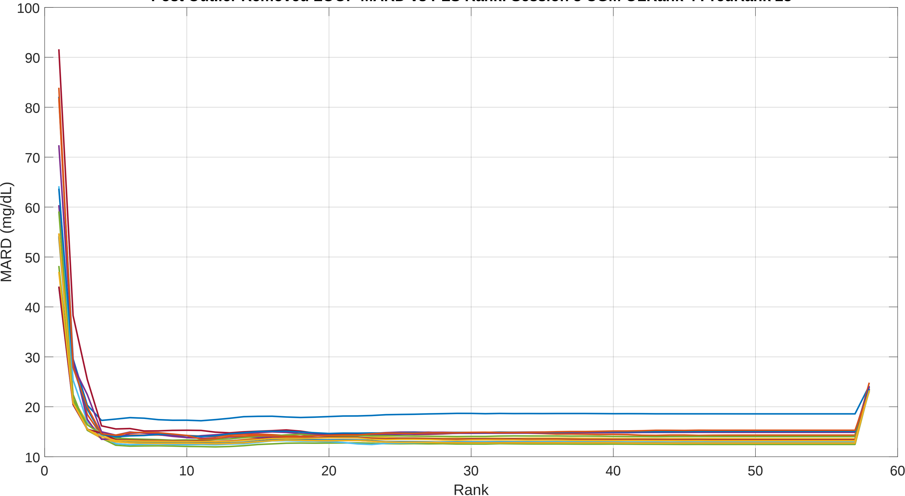
Post Outlier Removed LOOP MARD vs PLS Rank: Session 3 CGM OLRank 4 PredRank 28
