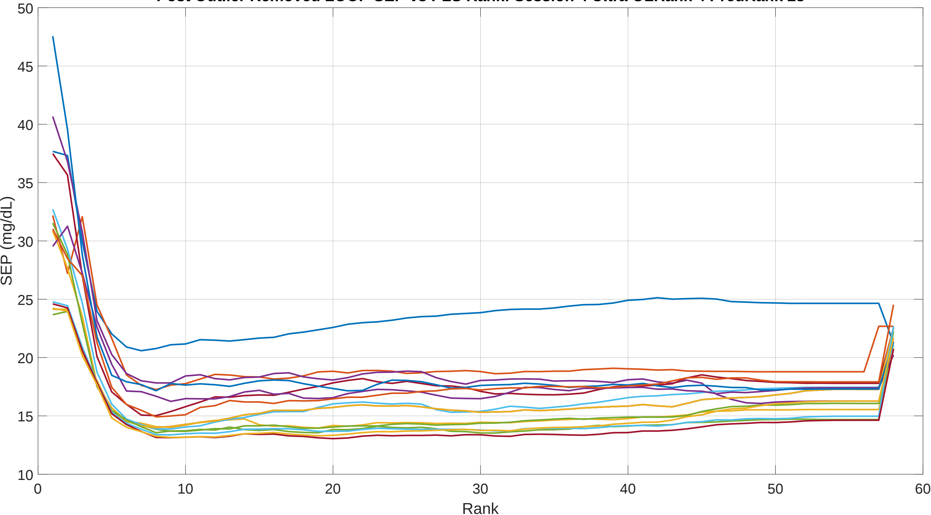
Post Outlier Removed LOOP SEP vs PLS Rank: Session 4 Ultra OLRank 4 PredRank 28
