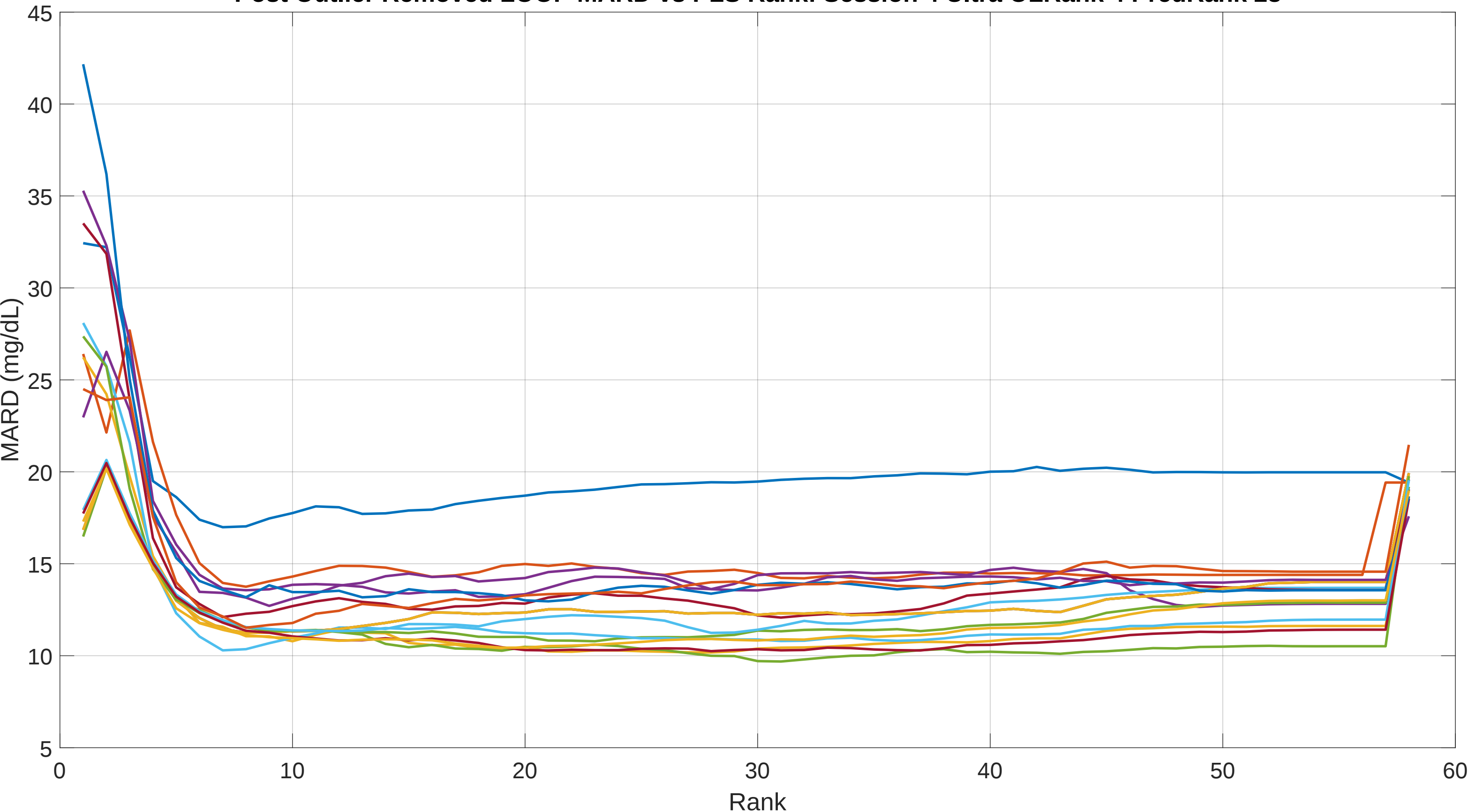
Post Outlier Removed LOOP MARD vs PLS Rank: Session 4 Ultra OLRank 4 PredRank 28
