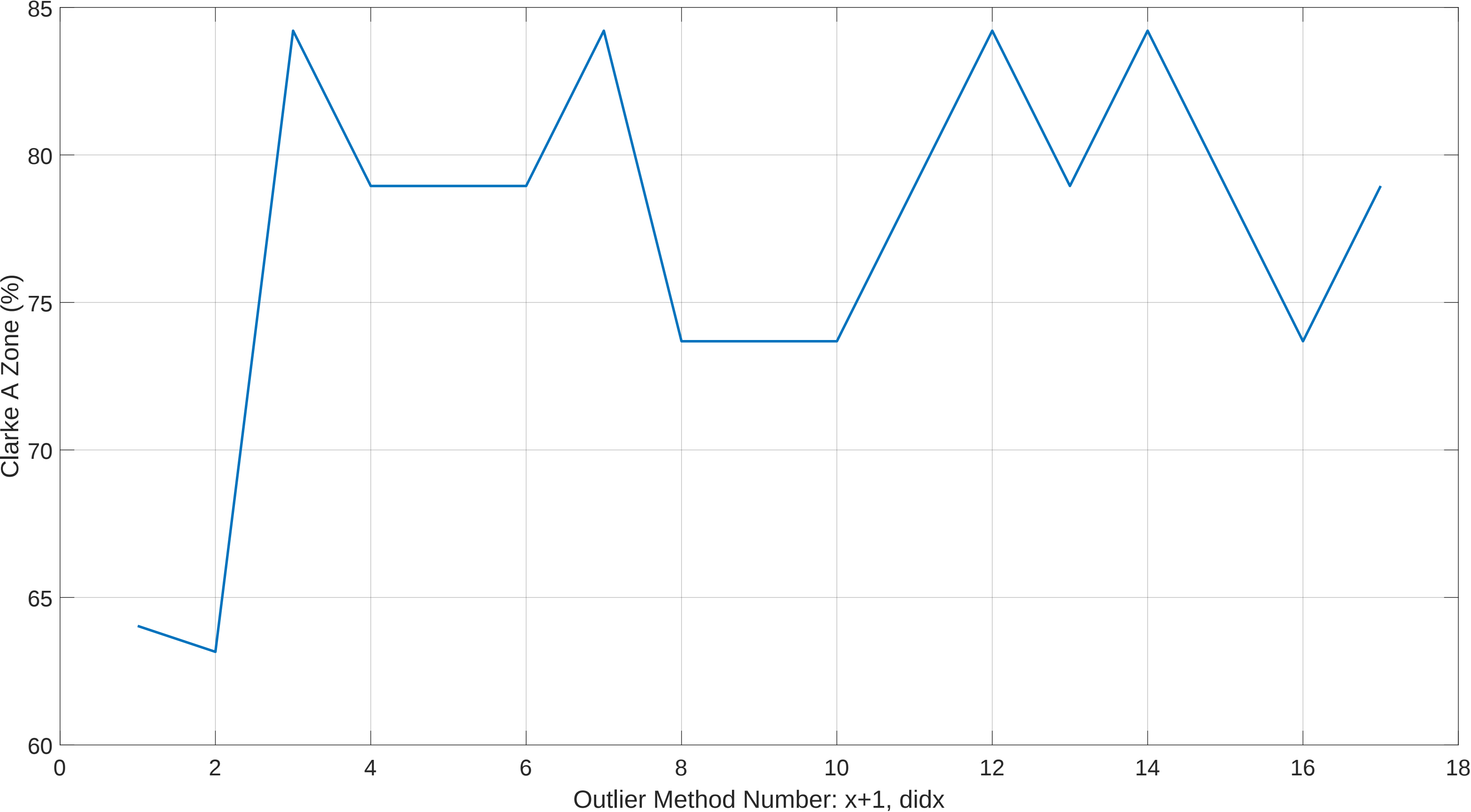
Post Outlier Removed LOOP Clarke A-Zone vs Outlier Method #: Session 4 Ultra OLRank 4 PredRank 28
