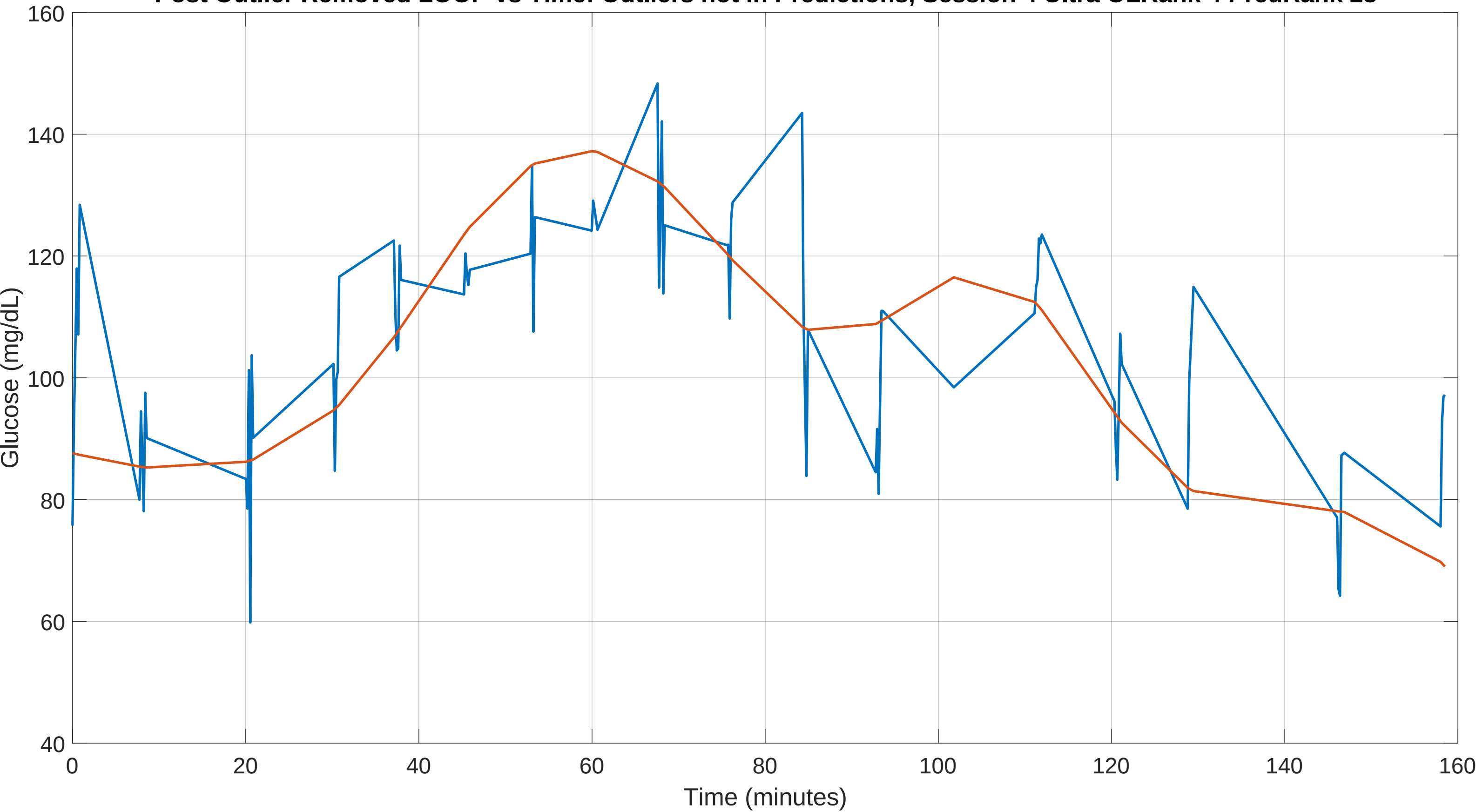
Post Outlier Removed LOOP vs Time: Outliers not in Predictions, Session 4 Ultra OLRank 4 PredRank 28
