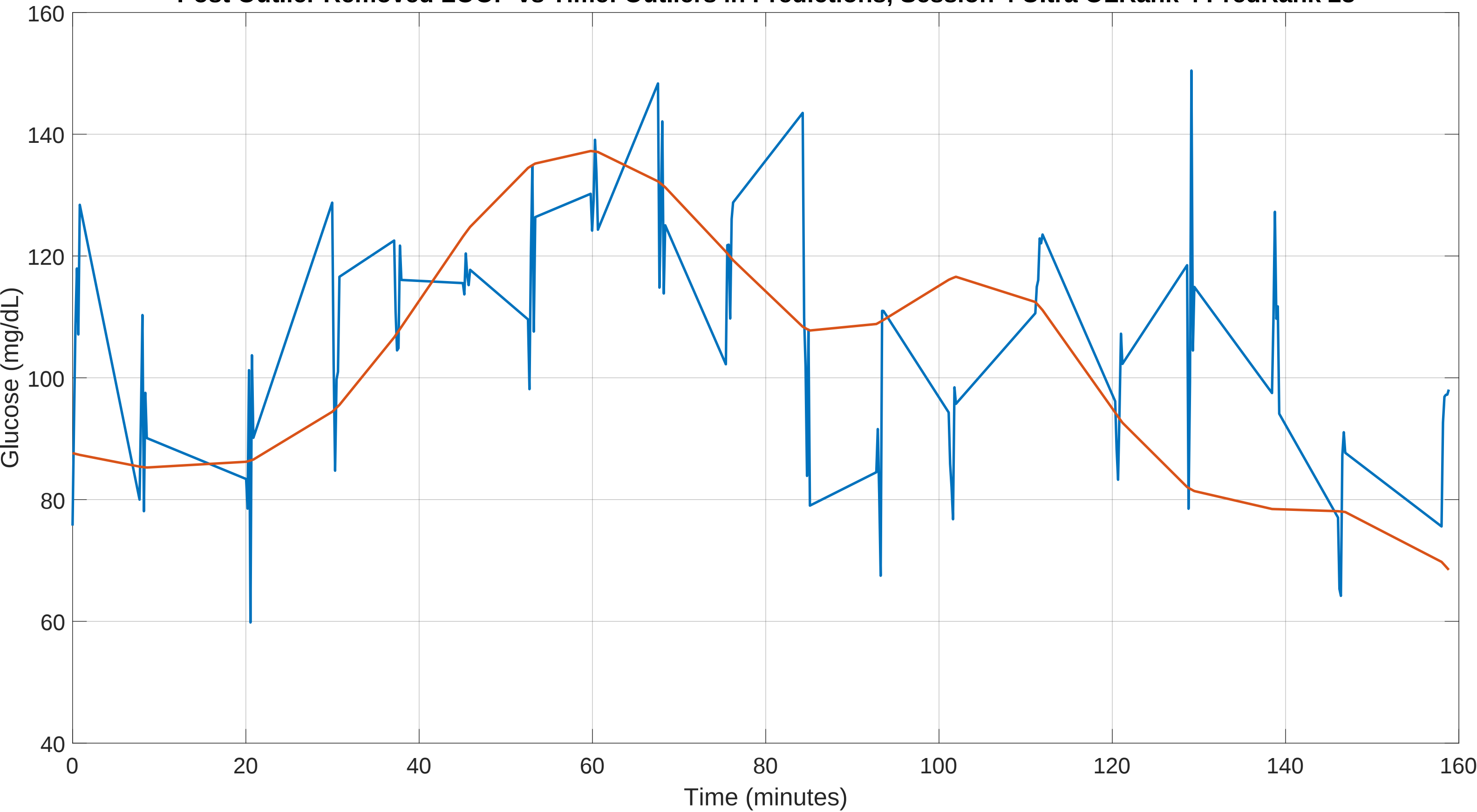
Post Outlier Removed LOOP vs Time: Outliers in Predictions, Session 4 Ultra OLRank 4 PredRank 28
