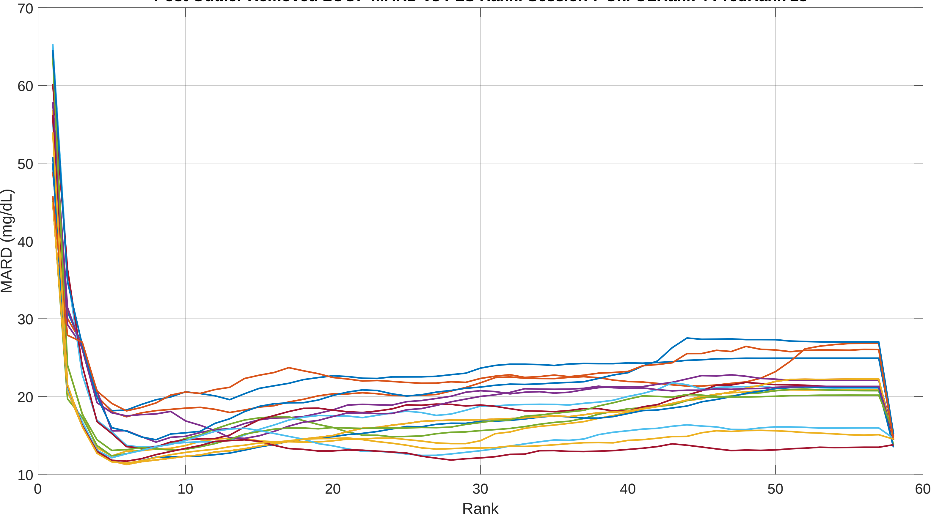
Post Outlier Removed LOOP MARD vs PLSRank: Session 7 Oxi OLRank 4 PredRank 28
