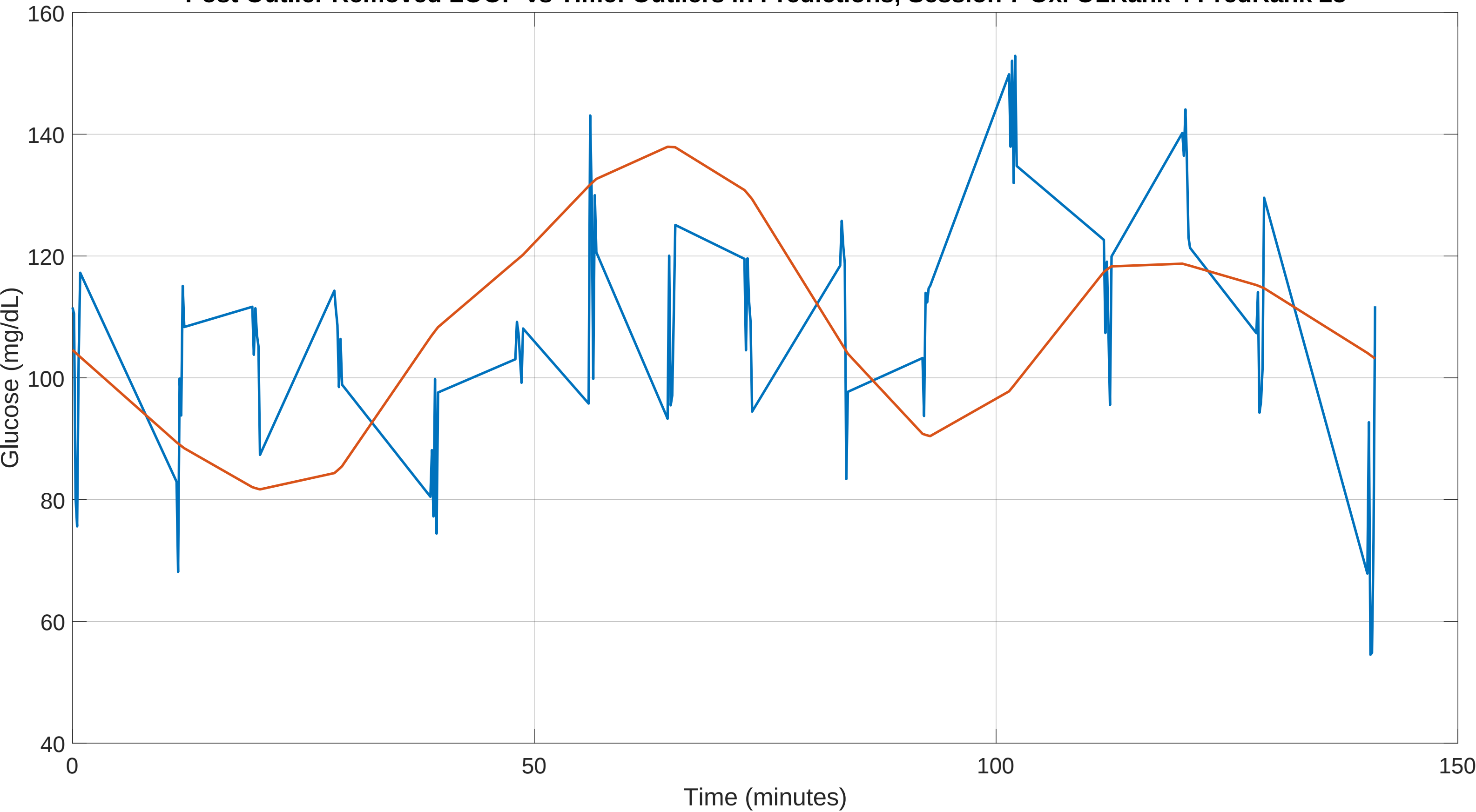
Post Outlier Removed LOOP vs Time: Outliers in Predictions, Session 7 Oxi OLRank 4 PredRank 28
