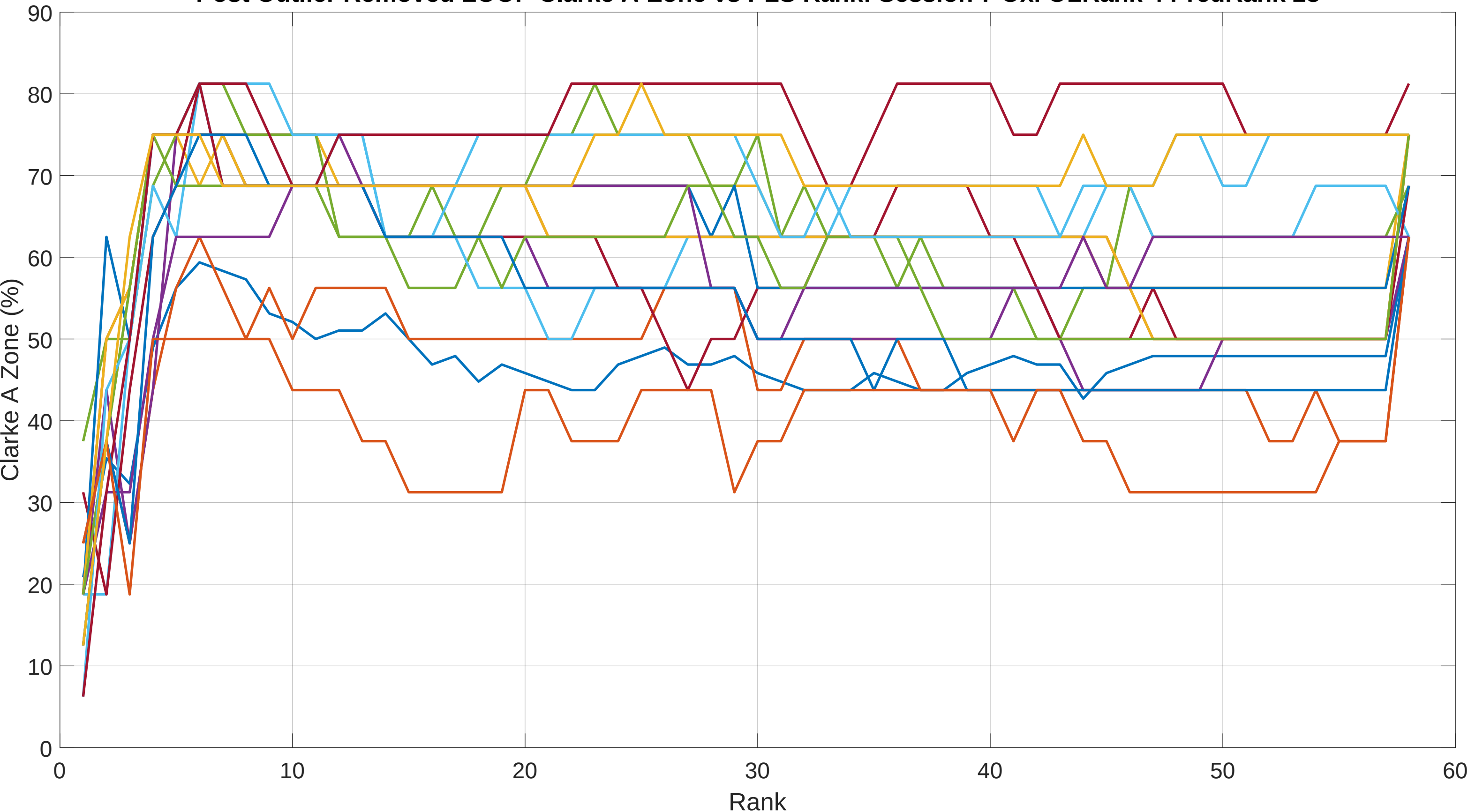
Post Outlier Removed LOOP Clarke A-Zone vs PLS Rank: Session 7 Oxi OLRank 4 PredRank 28
