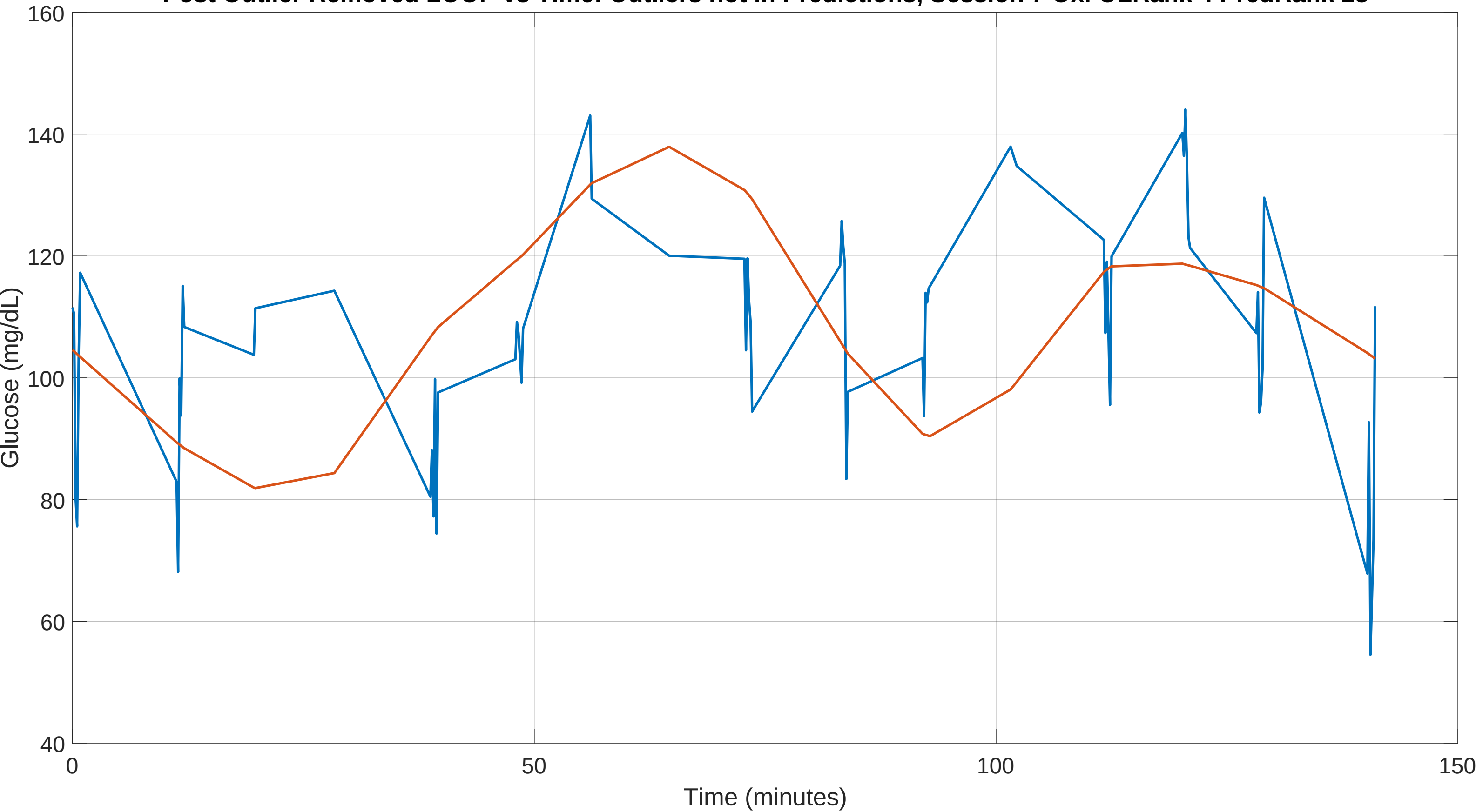
Post Outlier Removed LOOP vs Time: Outliers not in Predictions, Session 7 Oxi OLRank 4 PredRank 28
