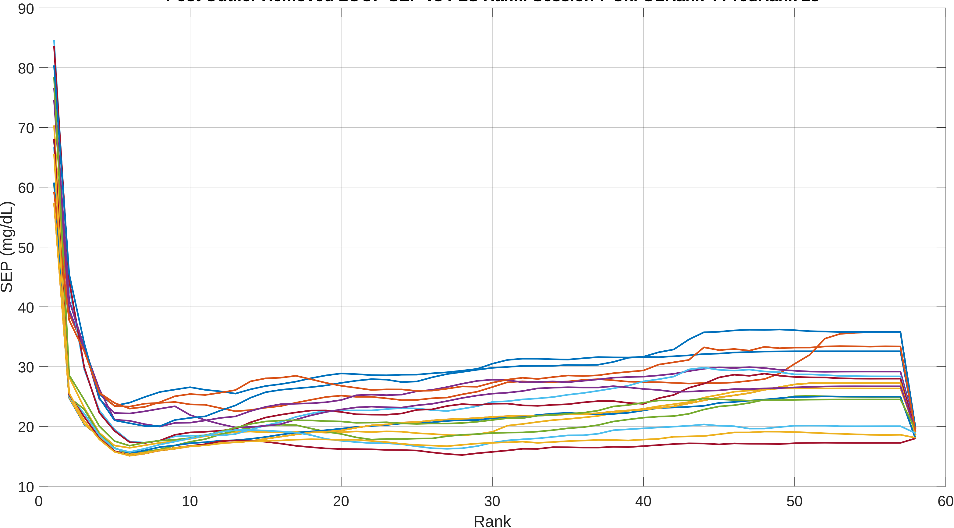
Post Outlier Removed LOOP SEP vs PLS Rank: Session 7 Oxi OLRank 4 PredRank 28
