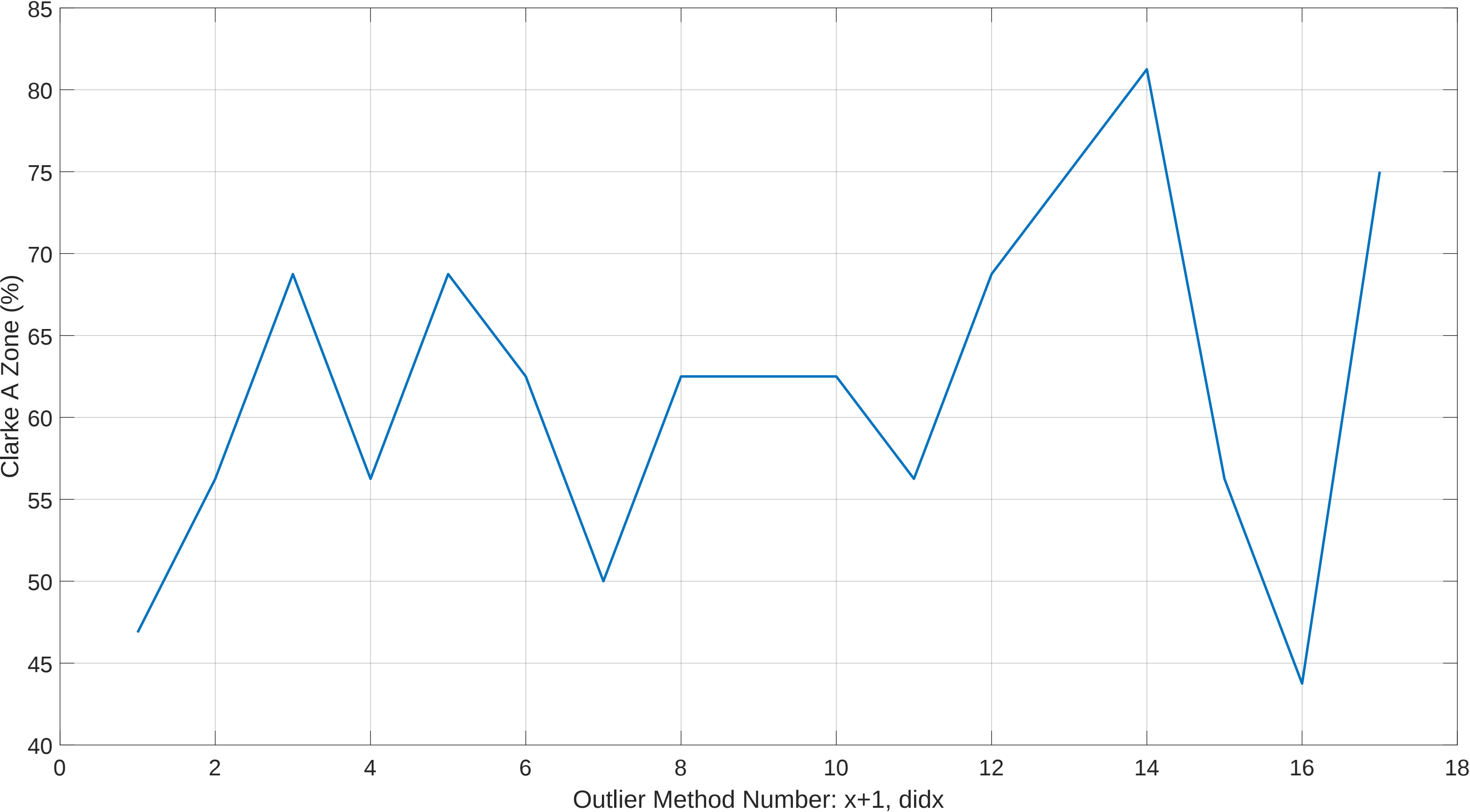
Post Outlier Removed LOOP Clarke A-Zone vs Outlier Method #: Session 7 Oxi OLRank 4 PredRank 28
