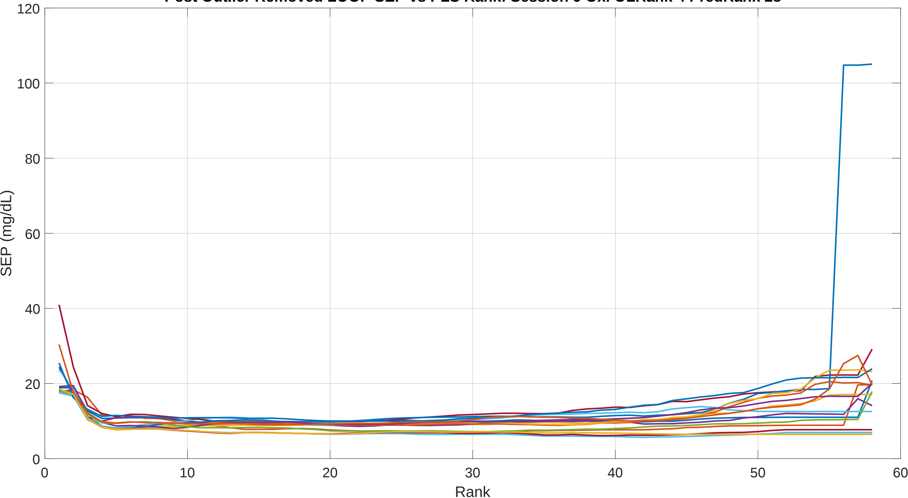
Post Outlier Removed LOOP SEP vs PLS Rank: Session 9 Oxi OLRank 4 PredRank 28
