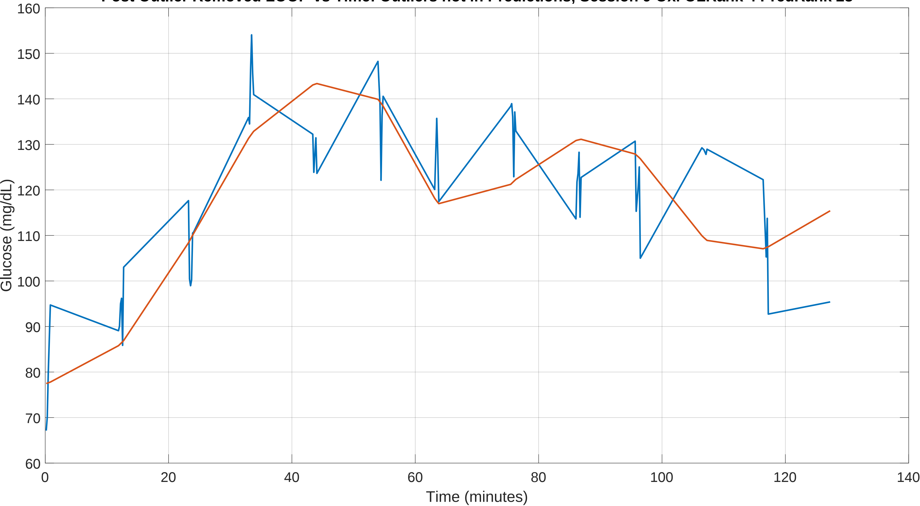
Post Outlier Removed LOOP vs Time: Outliers not in Predictions, Session 9 Oxi OLRank 4 PredRank 28
