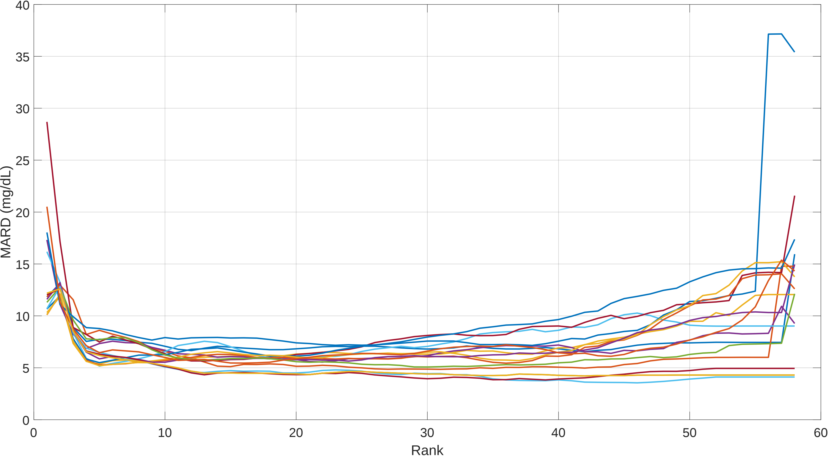
Post Outlier Removed LOOP MARD vs PLSRank: Session 9 Oxi OLRank 4 PredRank 28
