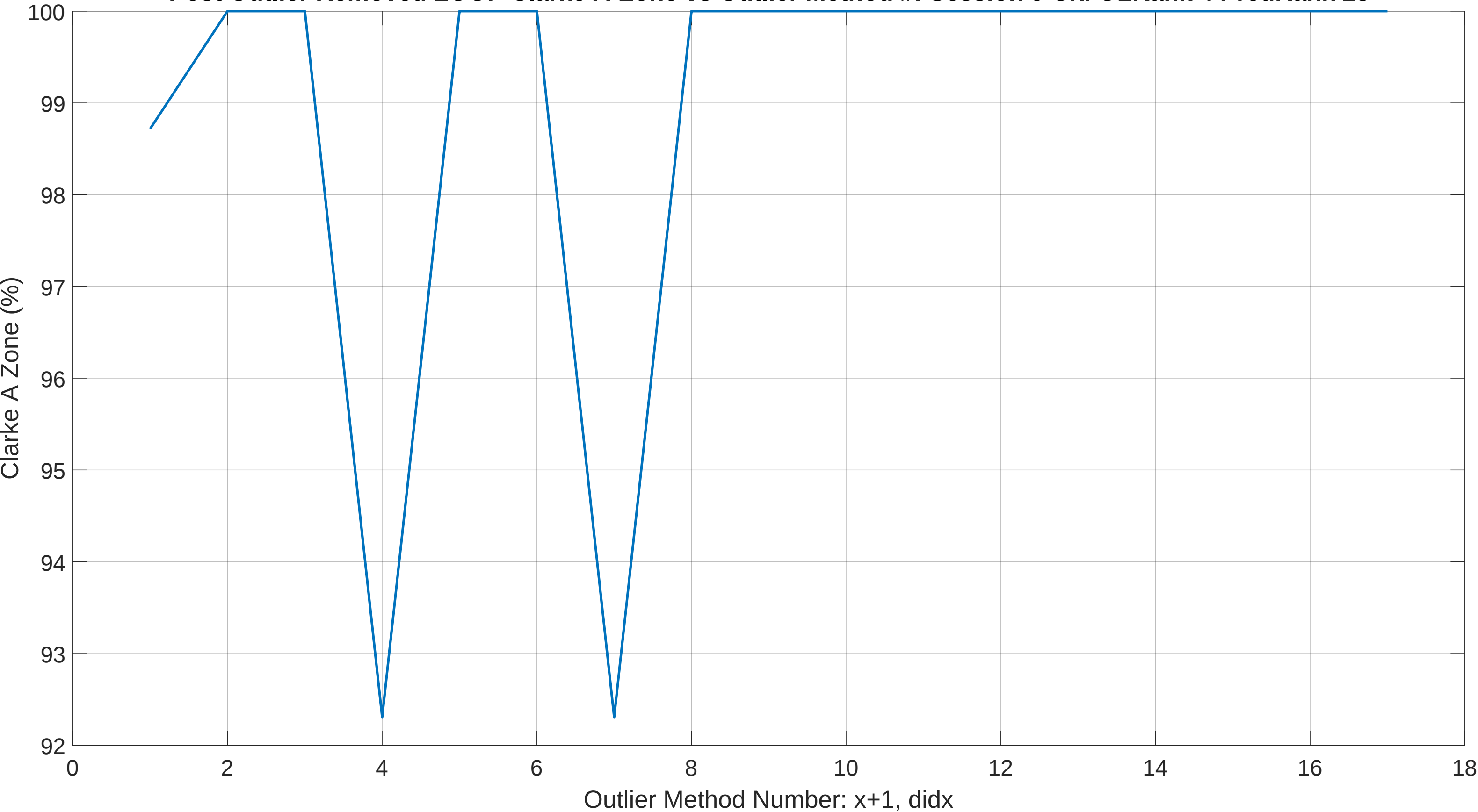
Post Outlier Removed LOOP Clarke A-Zone vs Outlier Method #: Session 9 Oxi OLRank 4 PredRank 28
