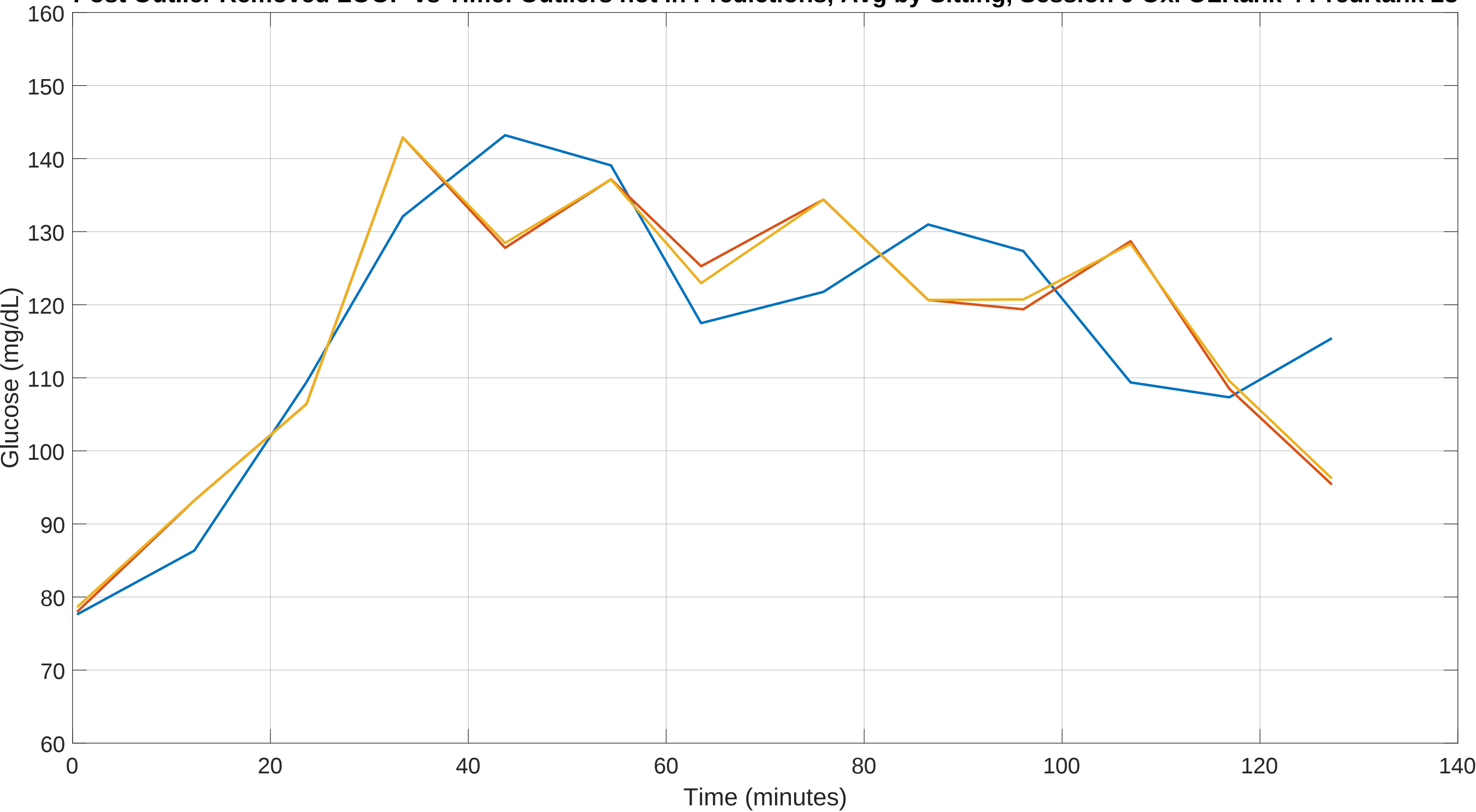
Post Outlier Removed LOOP vs Time: Outliers not in Predictions, Avg by Sitting, Session 9 Oxi OLRank 4 PredRank 28
