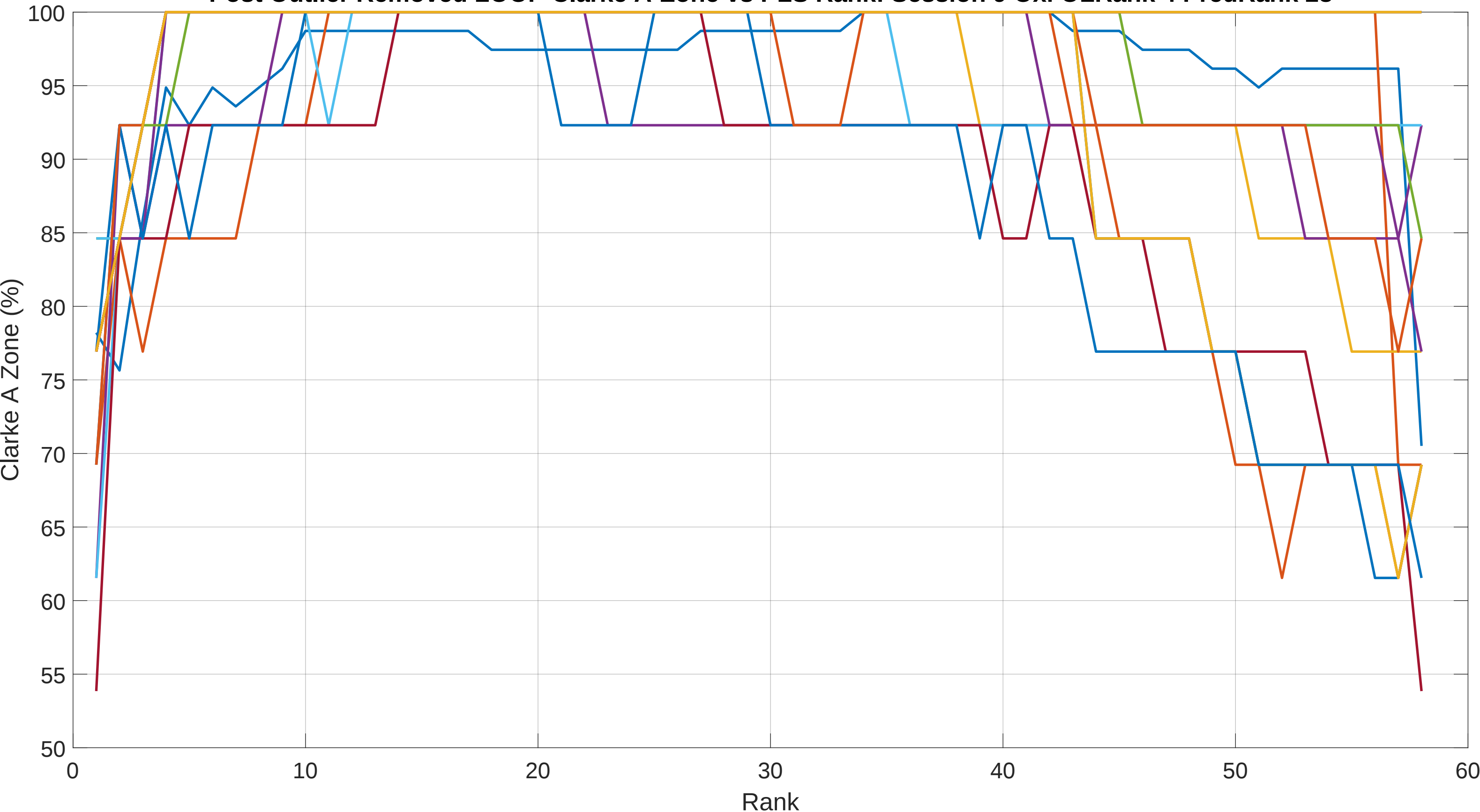
Post Outlier Removed LOOP Clarke A-Zone vs PLS Rank: Session 9 Oxi OLRank 4 PredRank 28
