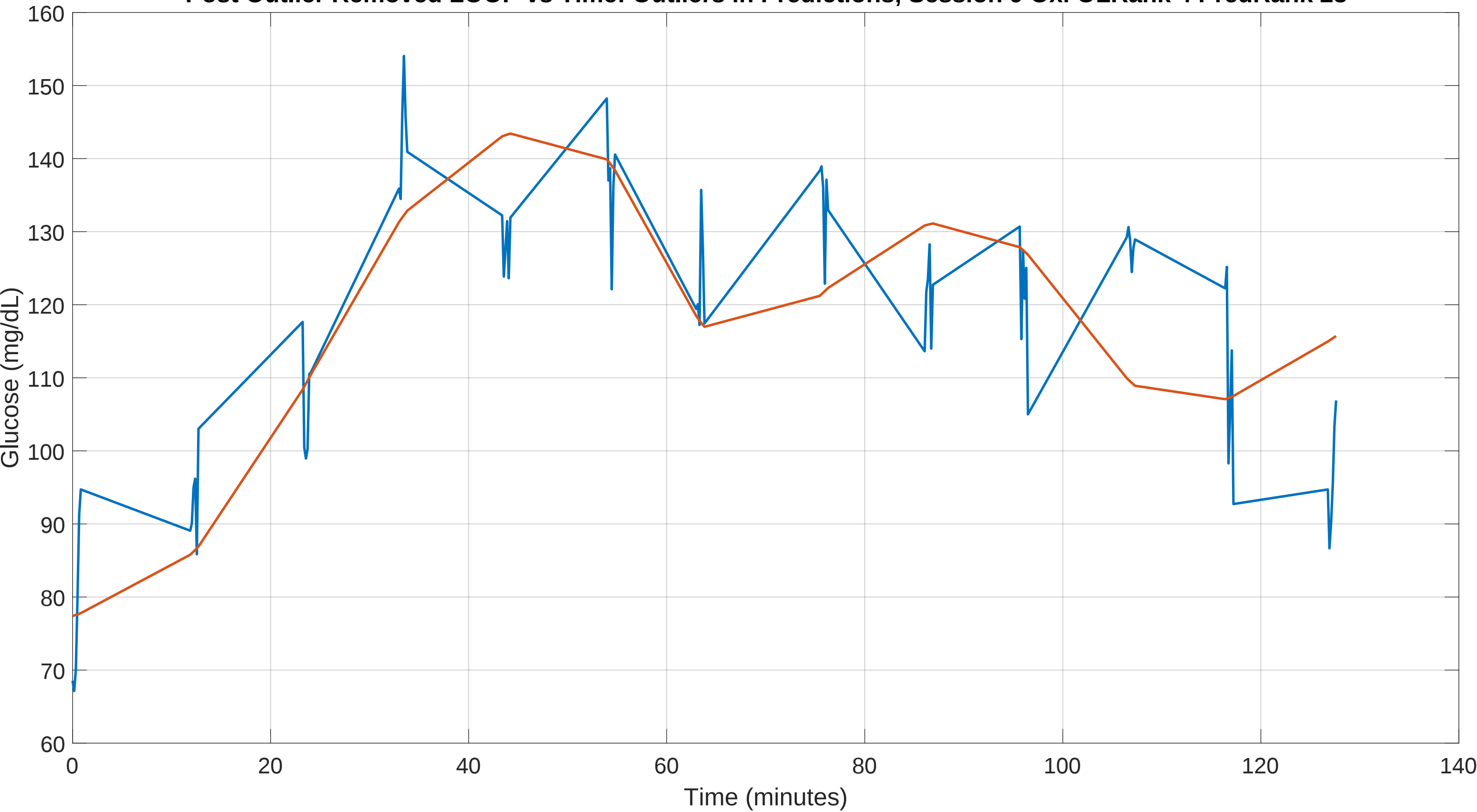
Post Outlier Removed LOOP vs Time: Outliers in Predictions, Session 9 Oxi OLRank 4 PredRank 28
