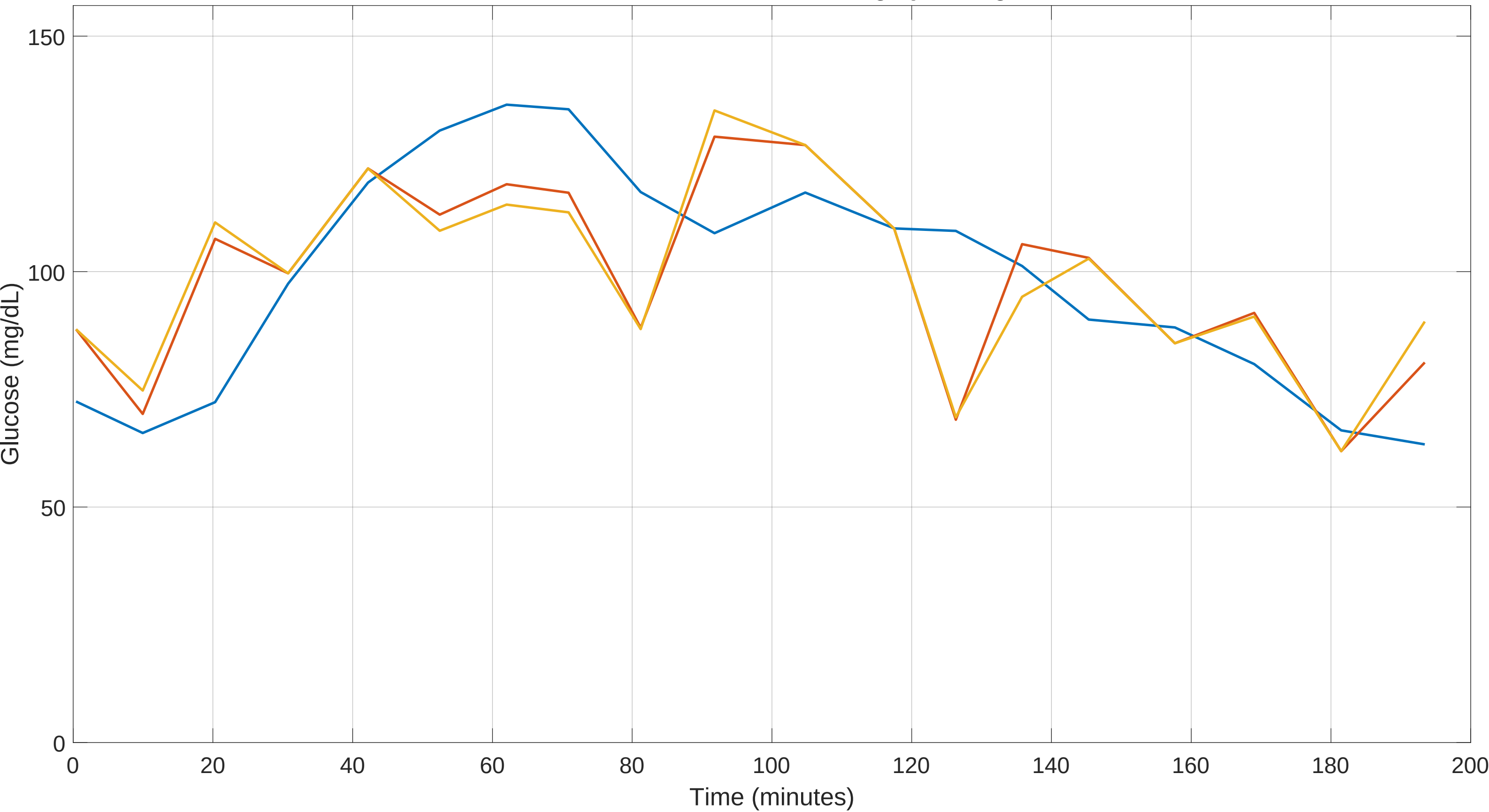
Post Outlier Removed LOOP vs Time: Outliers not in Predictions, Avg by Sitting, Session 12 Oxi OLRank 4 PredRank 28
