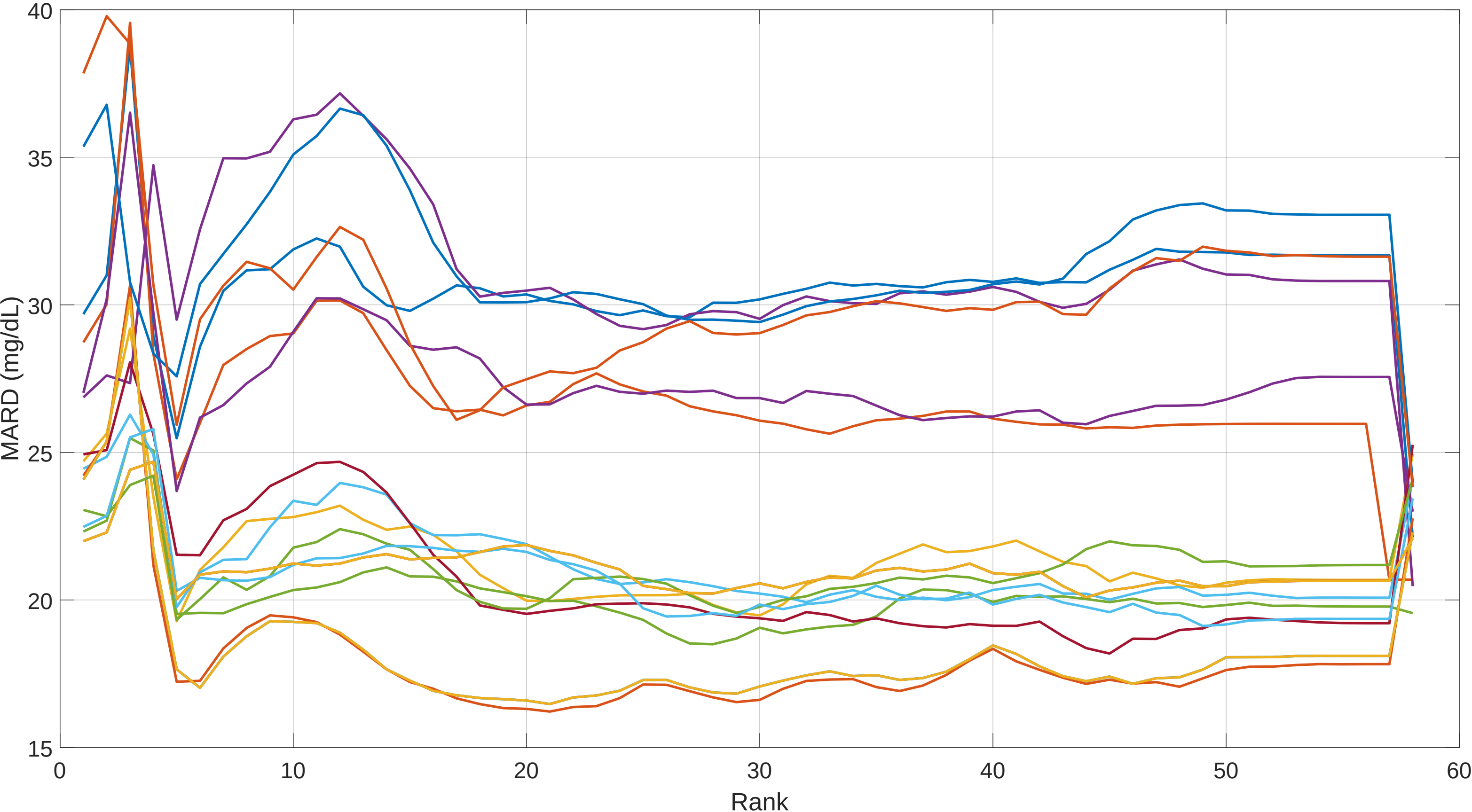
Post Outlier Removed LOOP MARD vs PLSRank: Session 12 Oxi OLRank 4 PredRank 28
