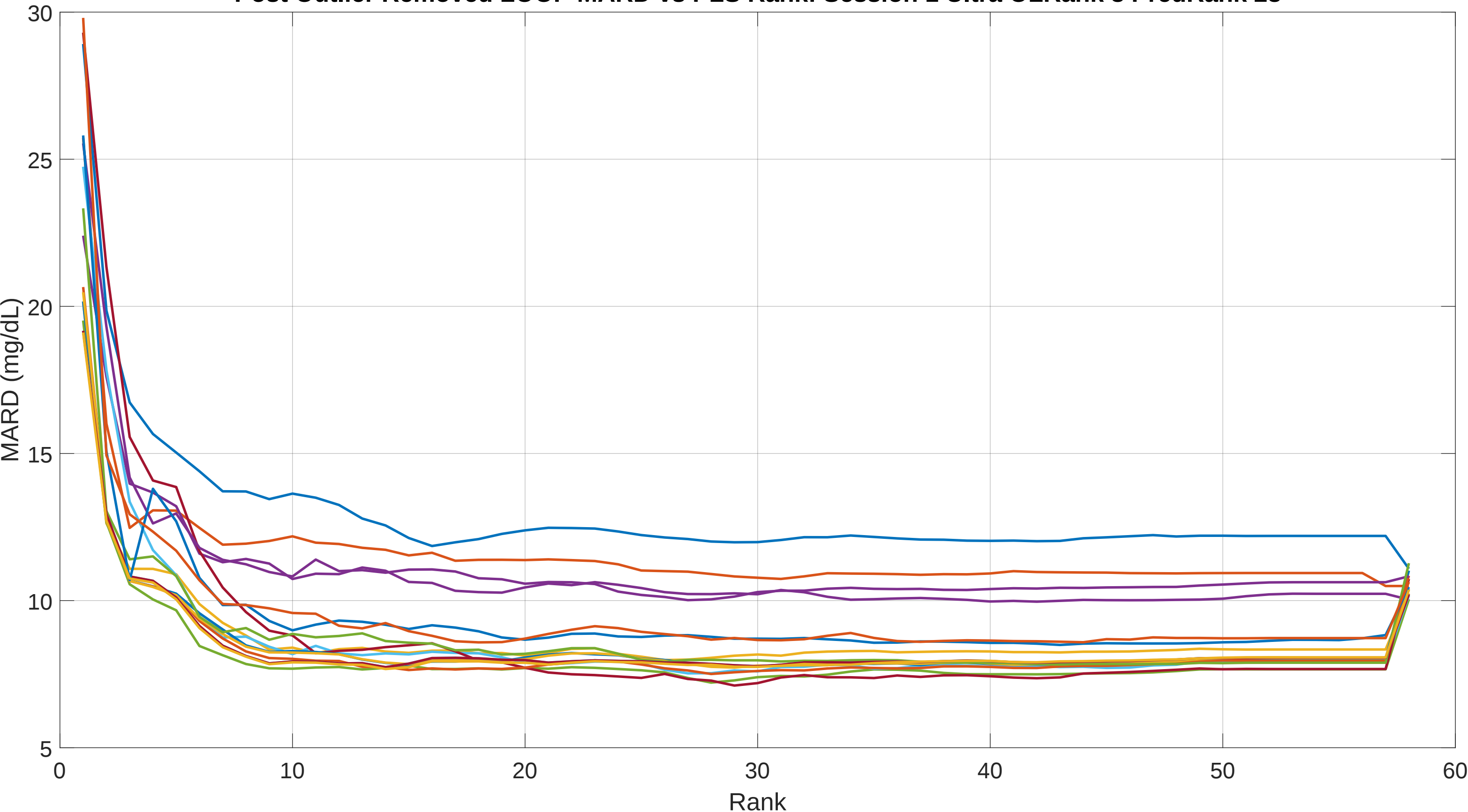
Post Outlier Removed LOOP MARD vs PLS Rank: Session 1 Ultra OLRank 8 PredRank 28
