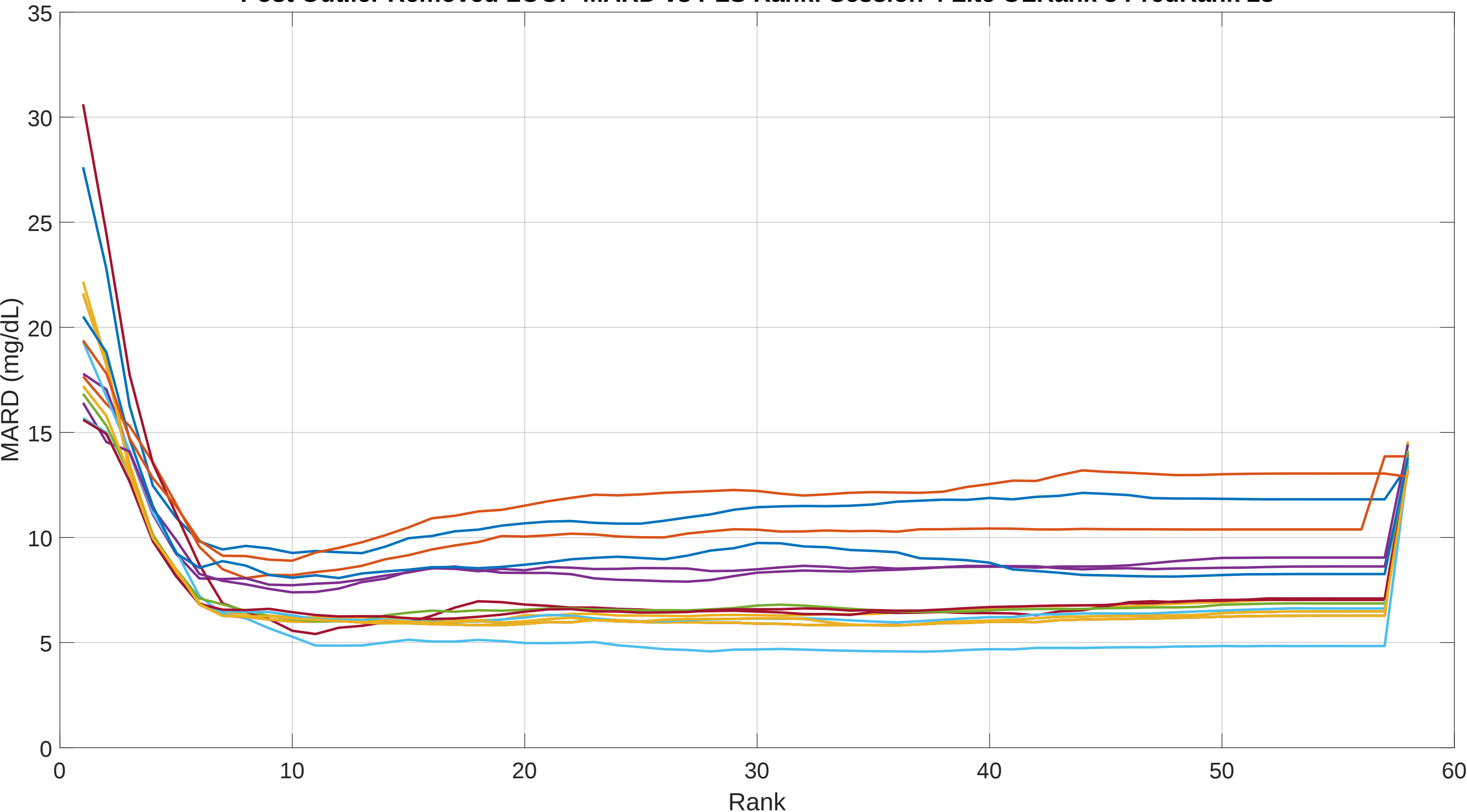
Post Outlier Removed LOOP MARD vs PLS Rank: Session 4 Lite OLRank 8 PredRank 28
