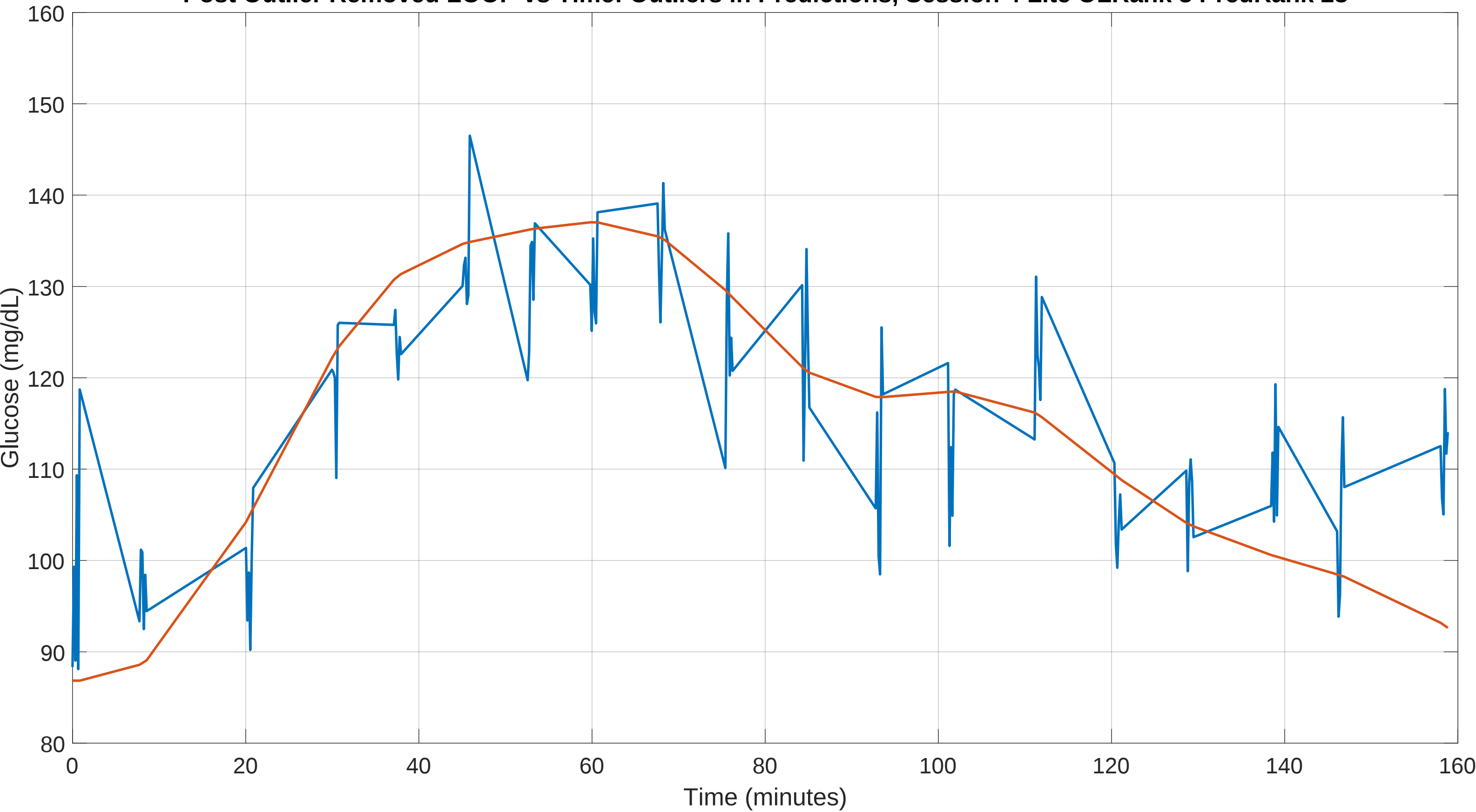
Post Outlier Removed LOOP vs Time: Outliers in Predictions, Session 4 Lite OLRank 8 PredRank 28
