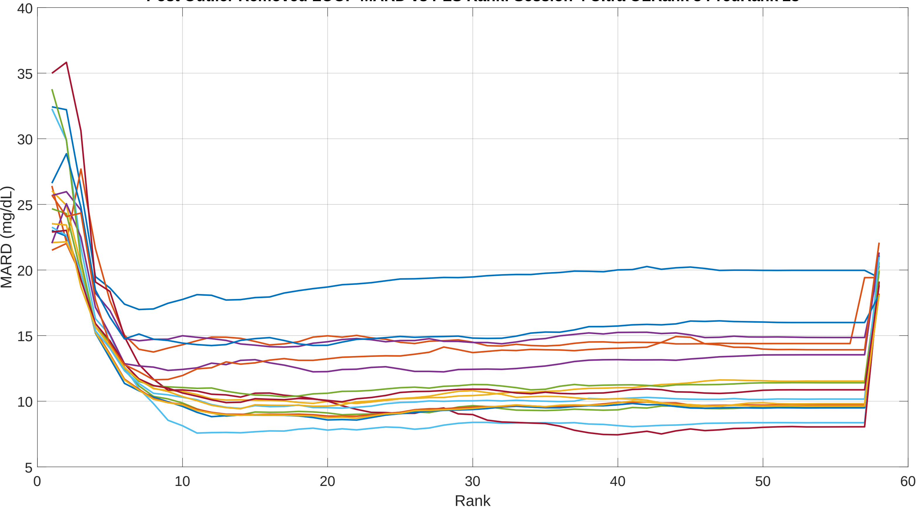
Post Outlier Removed LOOP MARD vs PLS Rank: Session 4 Ultra OLRank 8 PredRank 28
