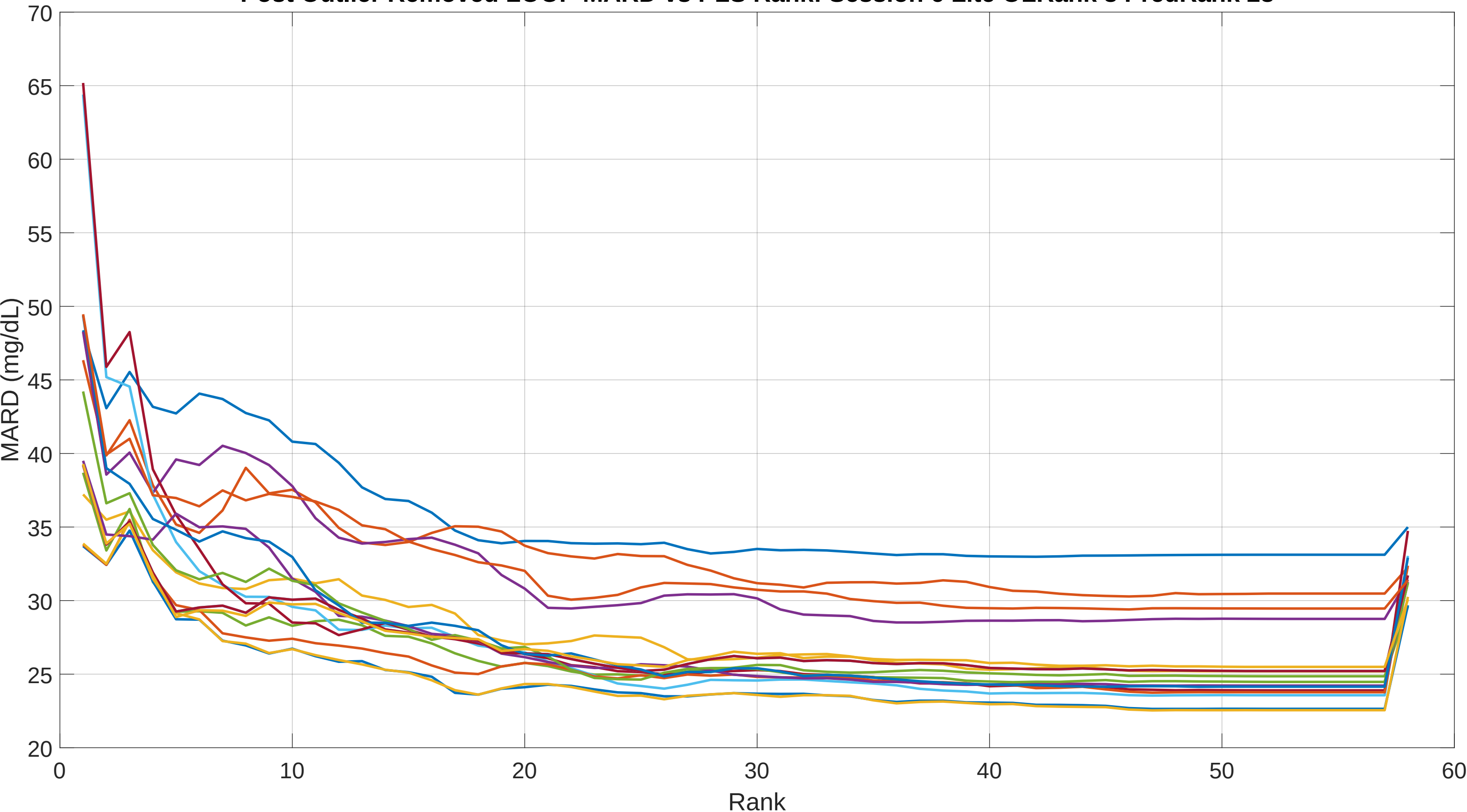
Post Outlier Removed LOOP MARD vs PLS Rank: Session 6 Lite OLRank 8 PredRank 28
