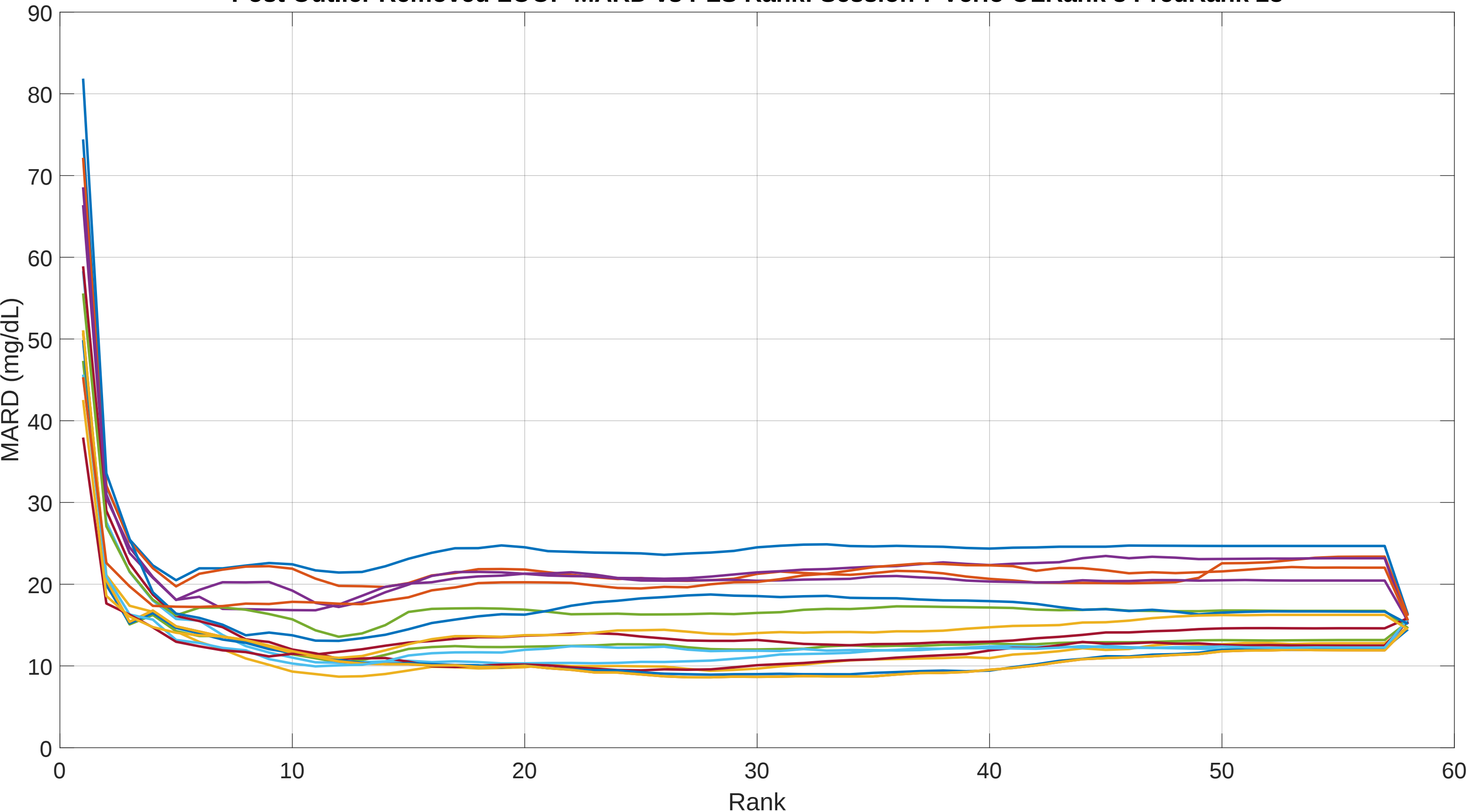
Post Outlier Removed LOOP MARD vs PLS Rank: Session 7 Verio OLRank 8 PredRank 28
