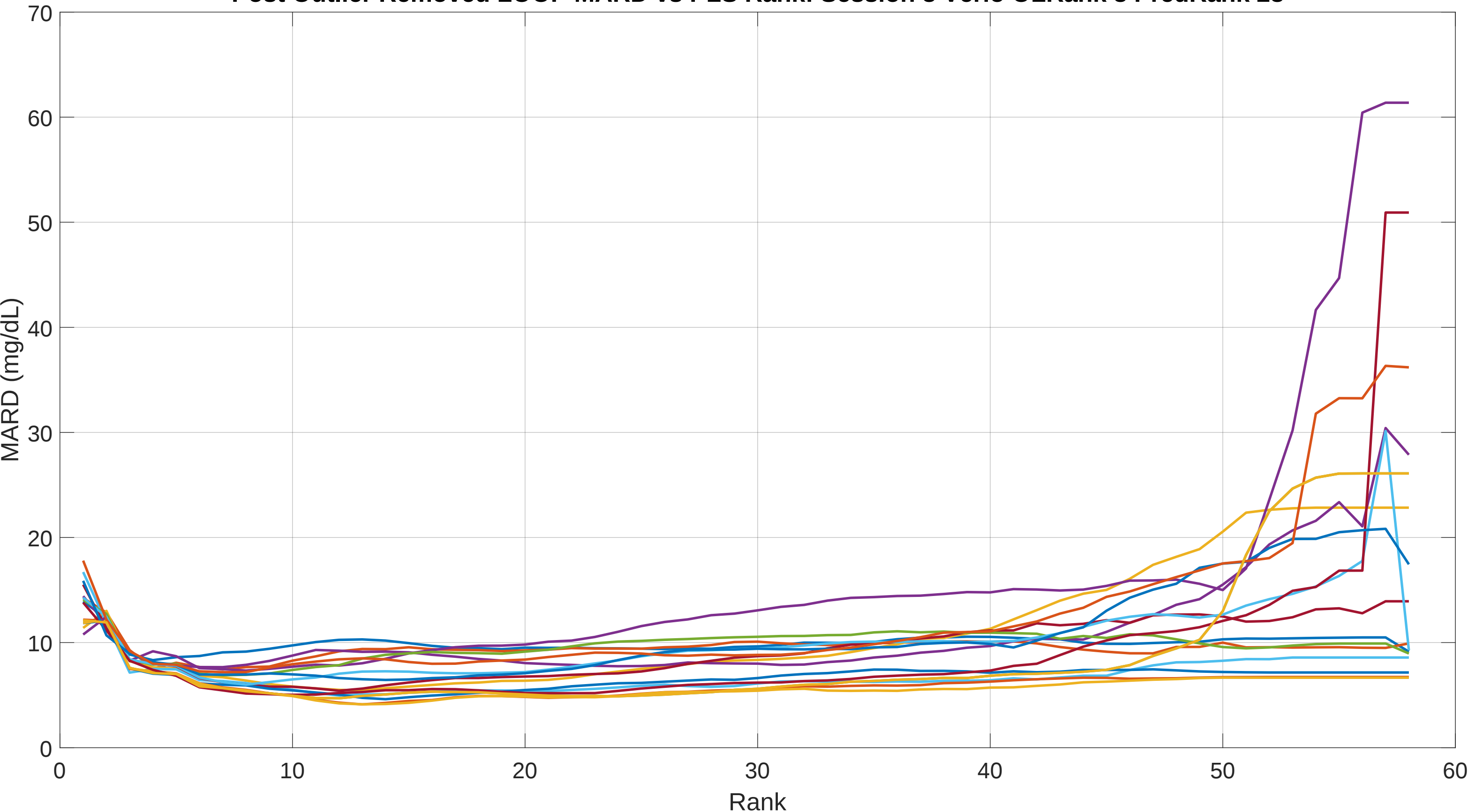
Post Outlier Removed LOOP MARD vs PLS Rank: Session 8 Verio OLRank 8 PredRank 28
