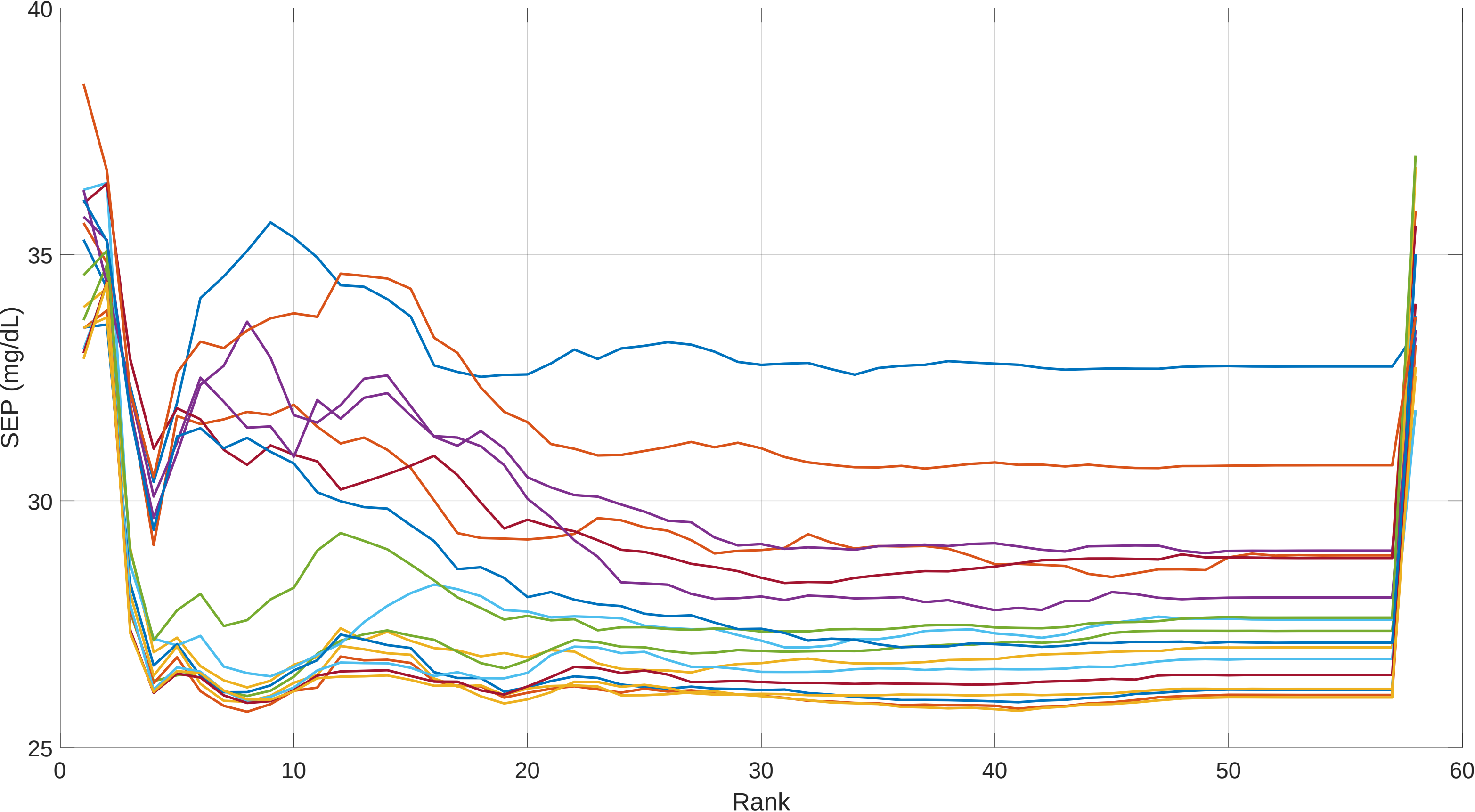
Post Outlier Removed LOOP SEP vs PLS Rank: Session 10 CGM OLRank 8 PredRank 28
