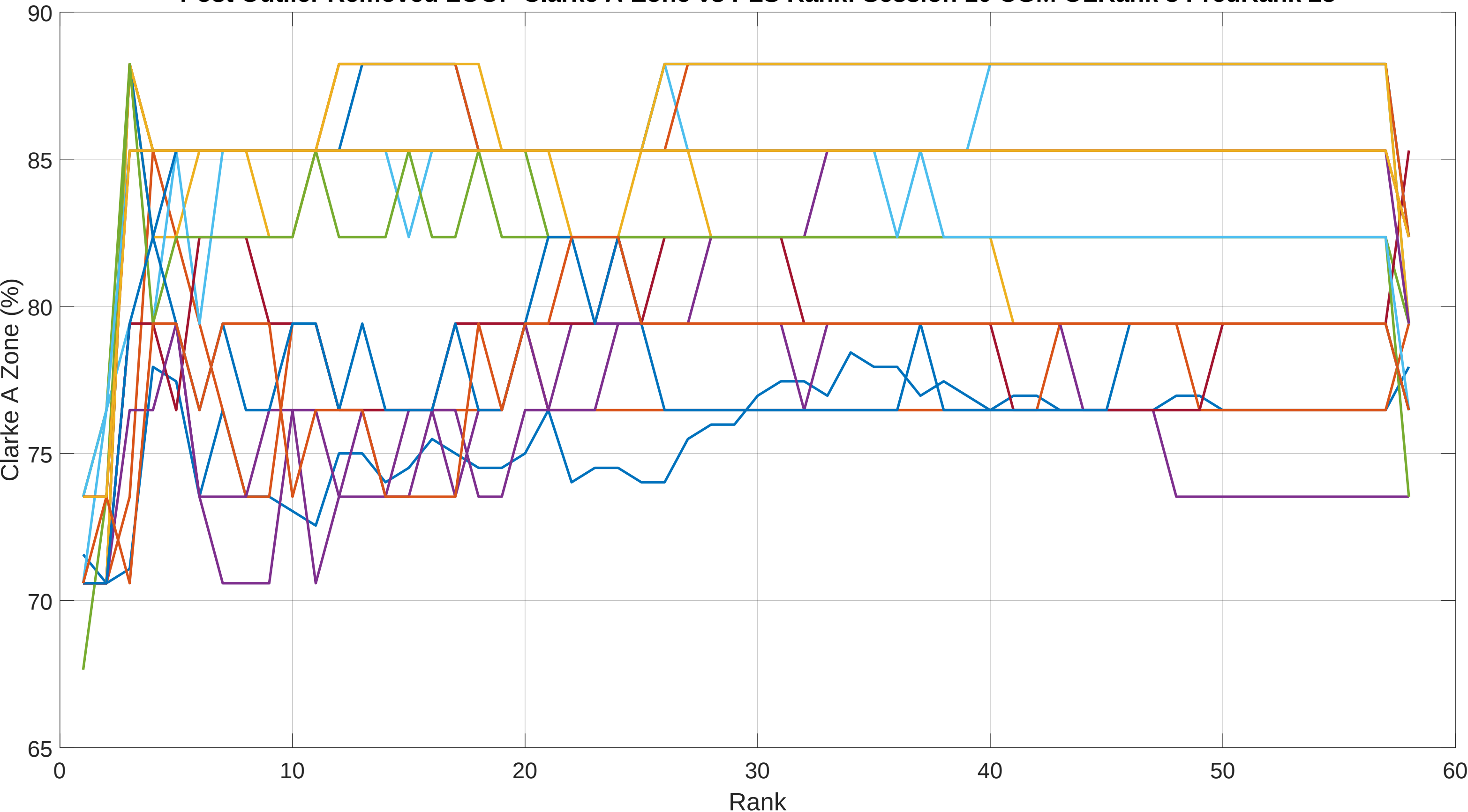
Post Outlier Removed LOOP Clarke A-Zone vs PLS Rank: Session 10 CGM OLRank 8 PredRank 28
