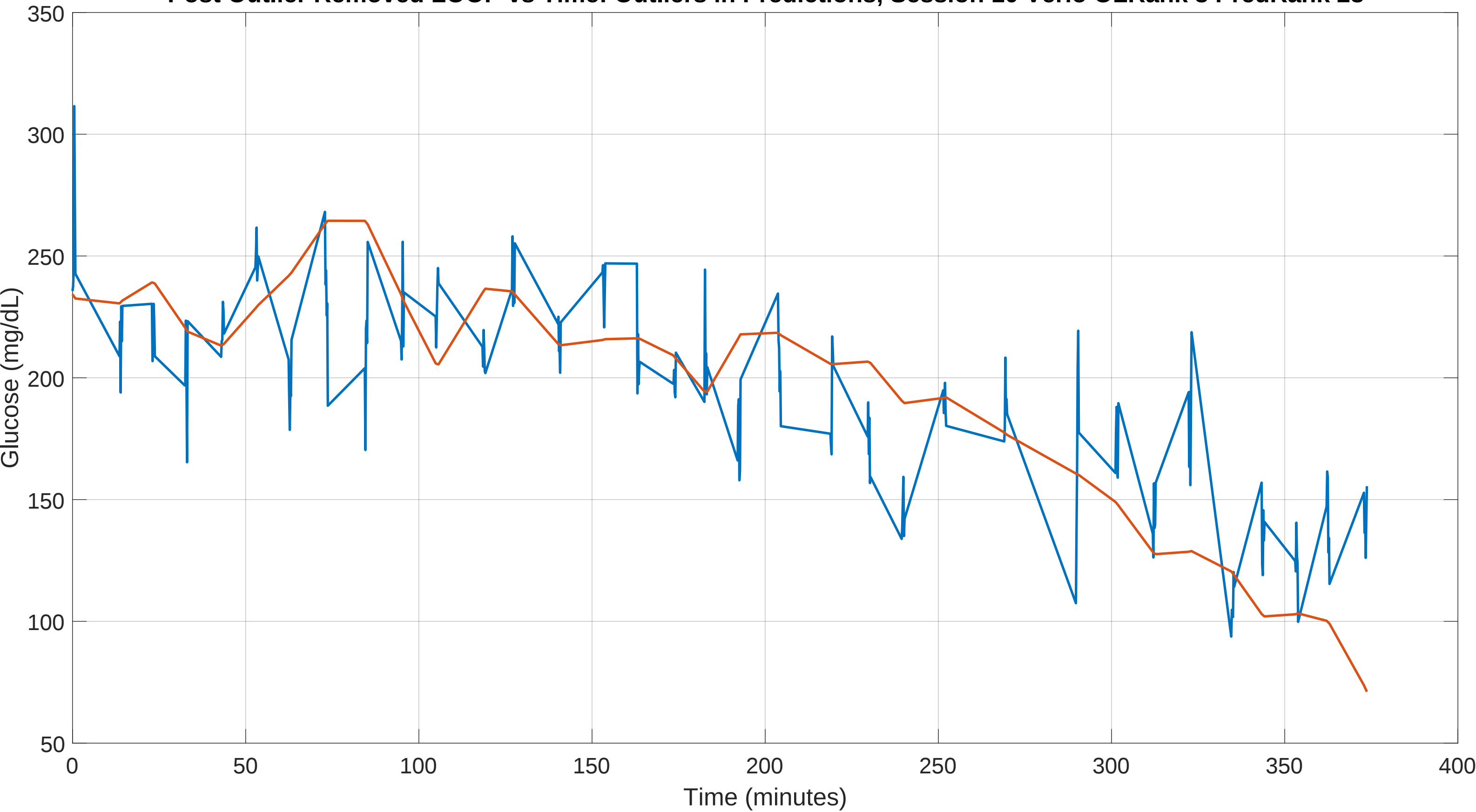
Post Outlier Removed LOOP vs Time: Outliers in Predictions, Session 10 Verio OLRank 8 PredRank 28
