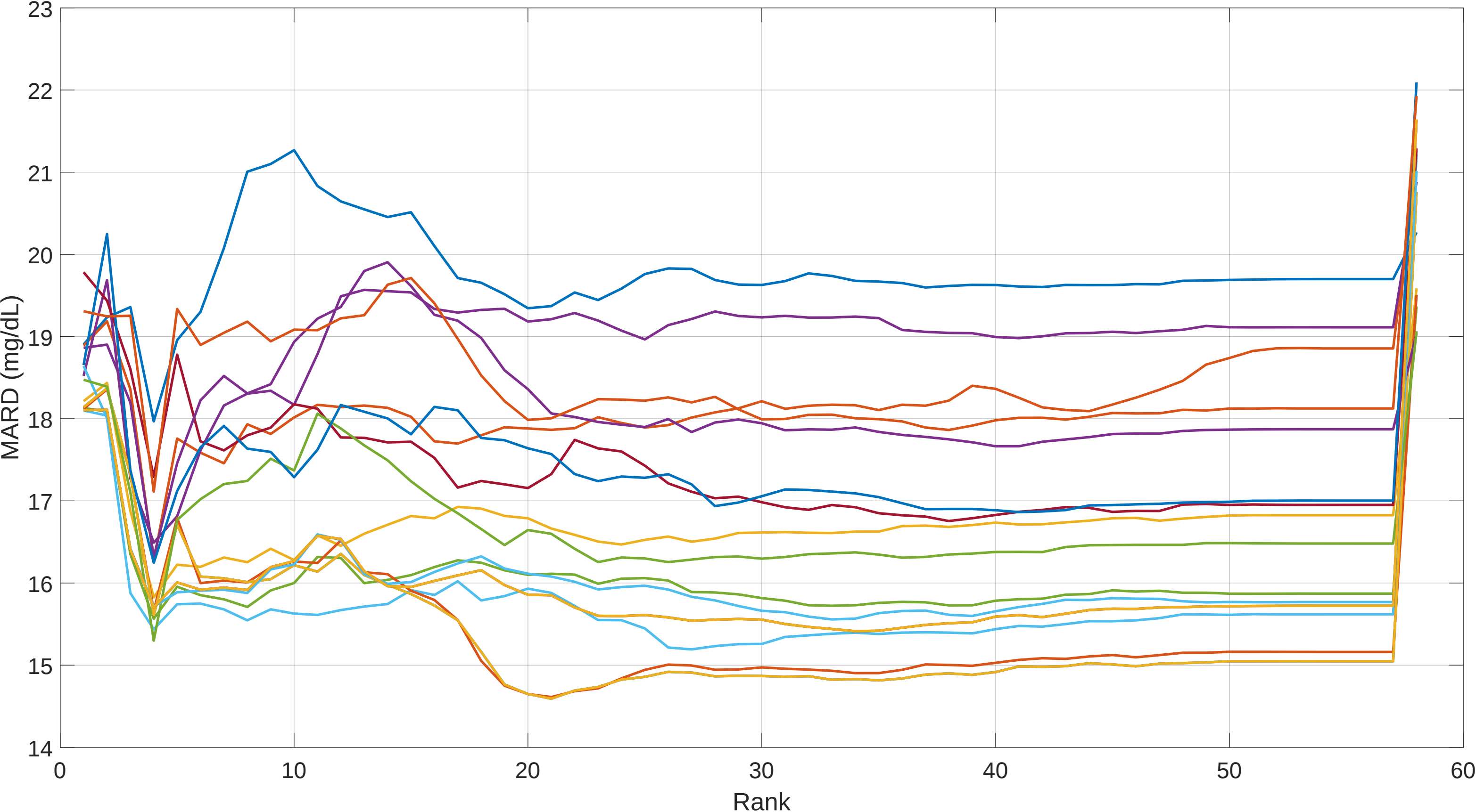
Post Outlier Removed LOOP MARD vs PLS Rank: Session 10 Verio OLRank 8 PredRank 28
