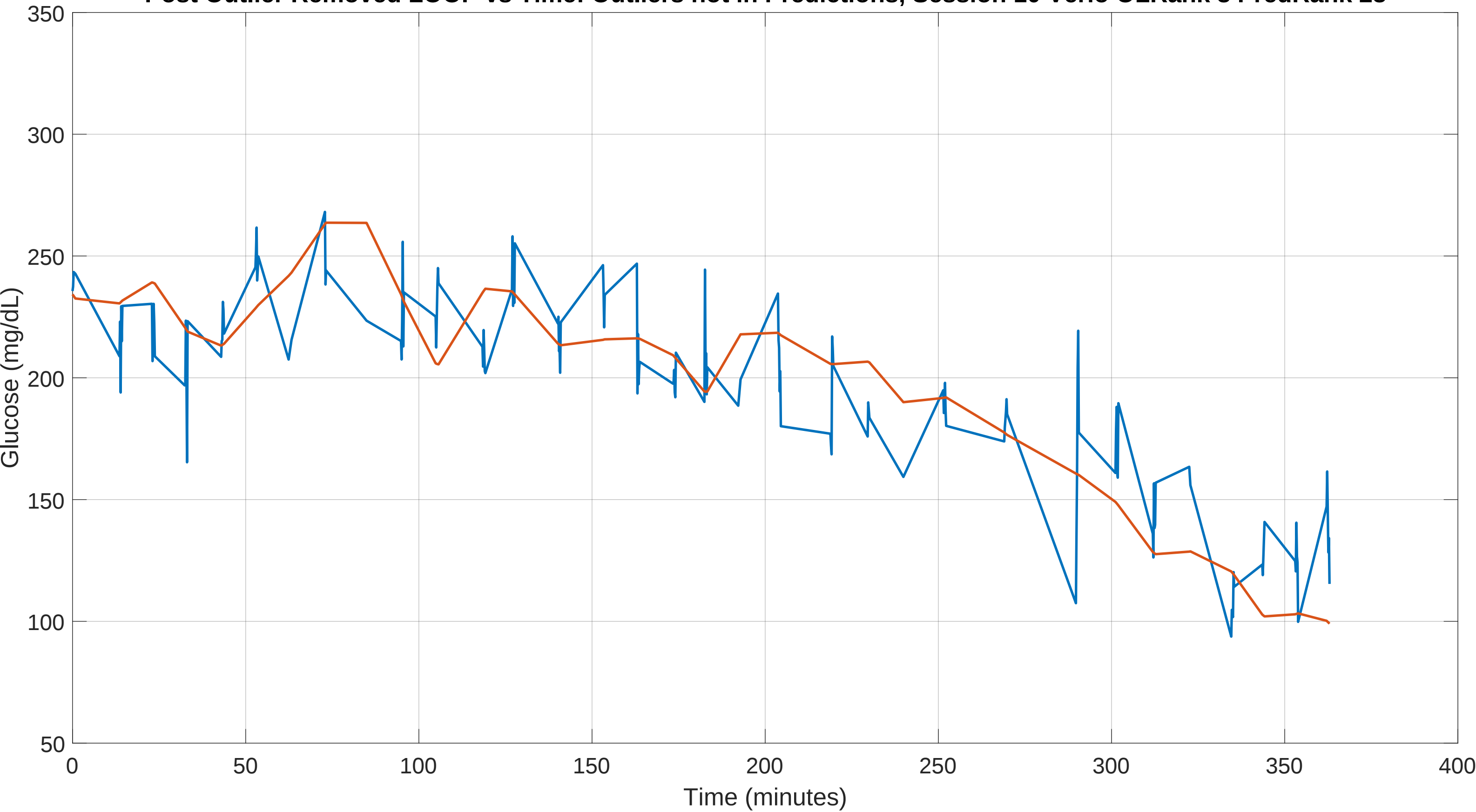
Post Outlier Removed LOOP vs Time: Outliers not in Predictions, Session 10 Verio OLRank 8PredRank 28
