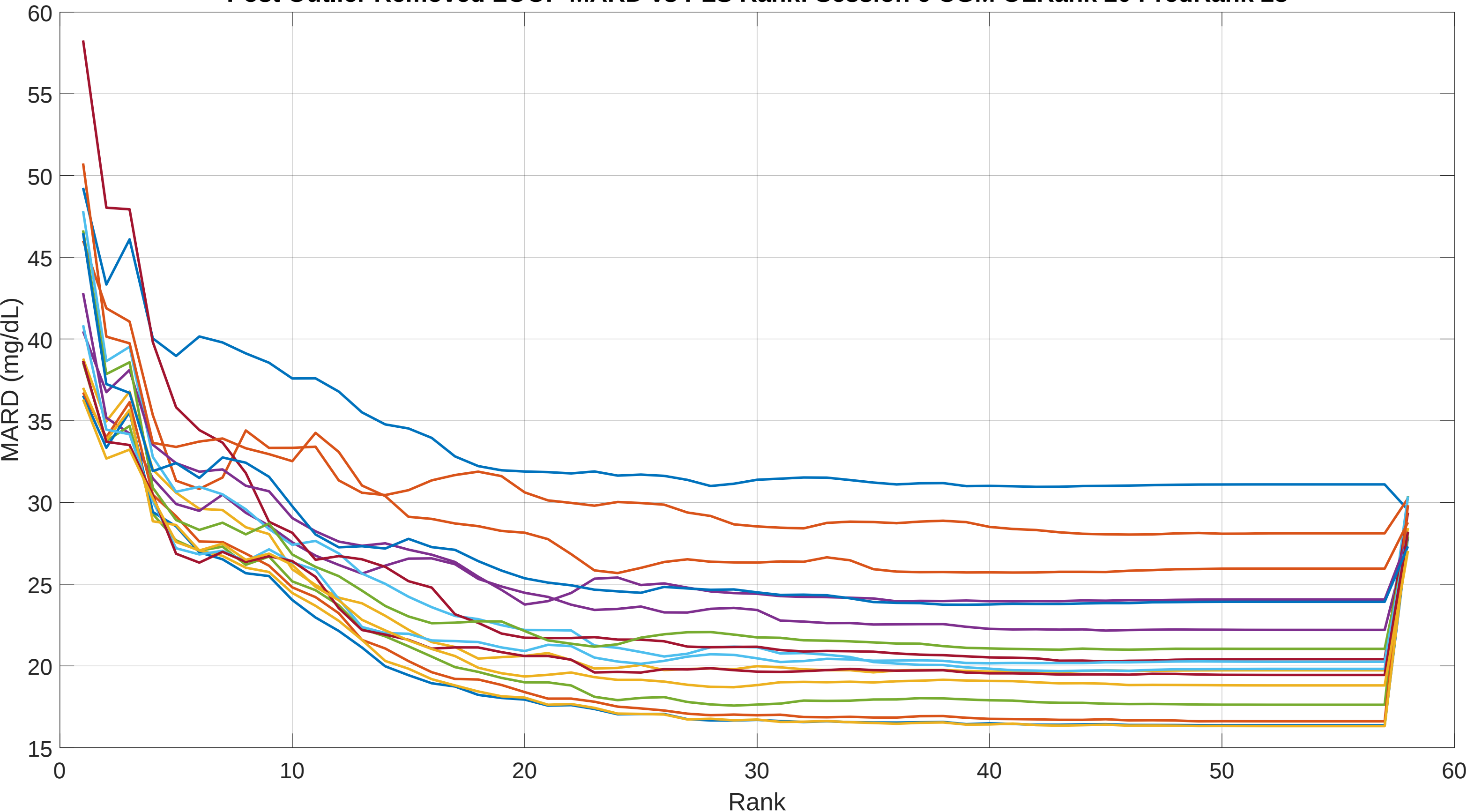
Post Outlier Removed LOOP MARD vs PLS Rank: Session 6 CGM OLRank 20 PredRank 28
