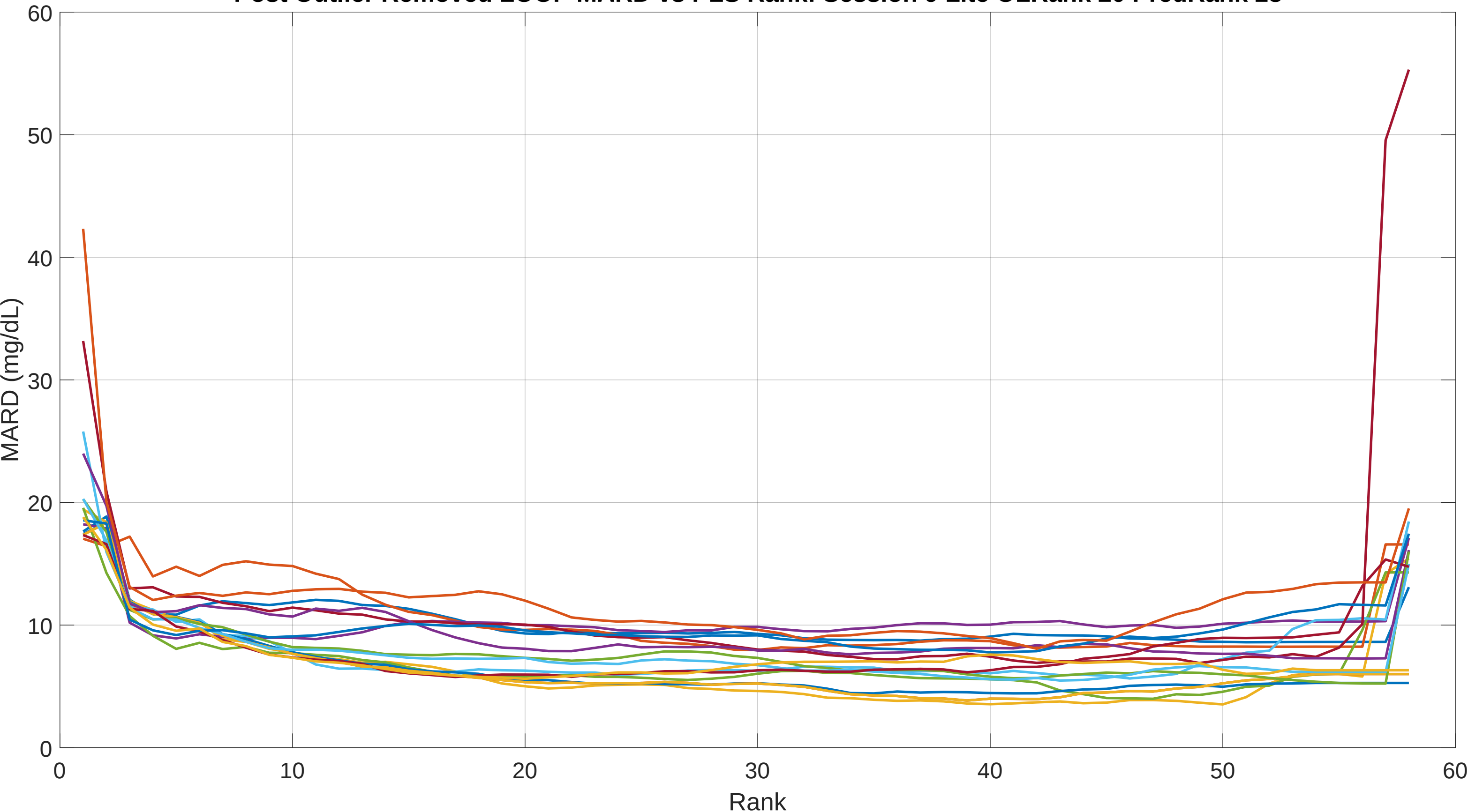
Post Outlier Removed LOOP MARD vs PLS Rank: Session 9 Lite OLRank 20 PredRank 28
