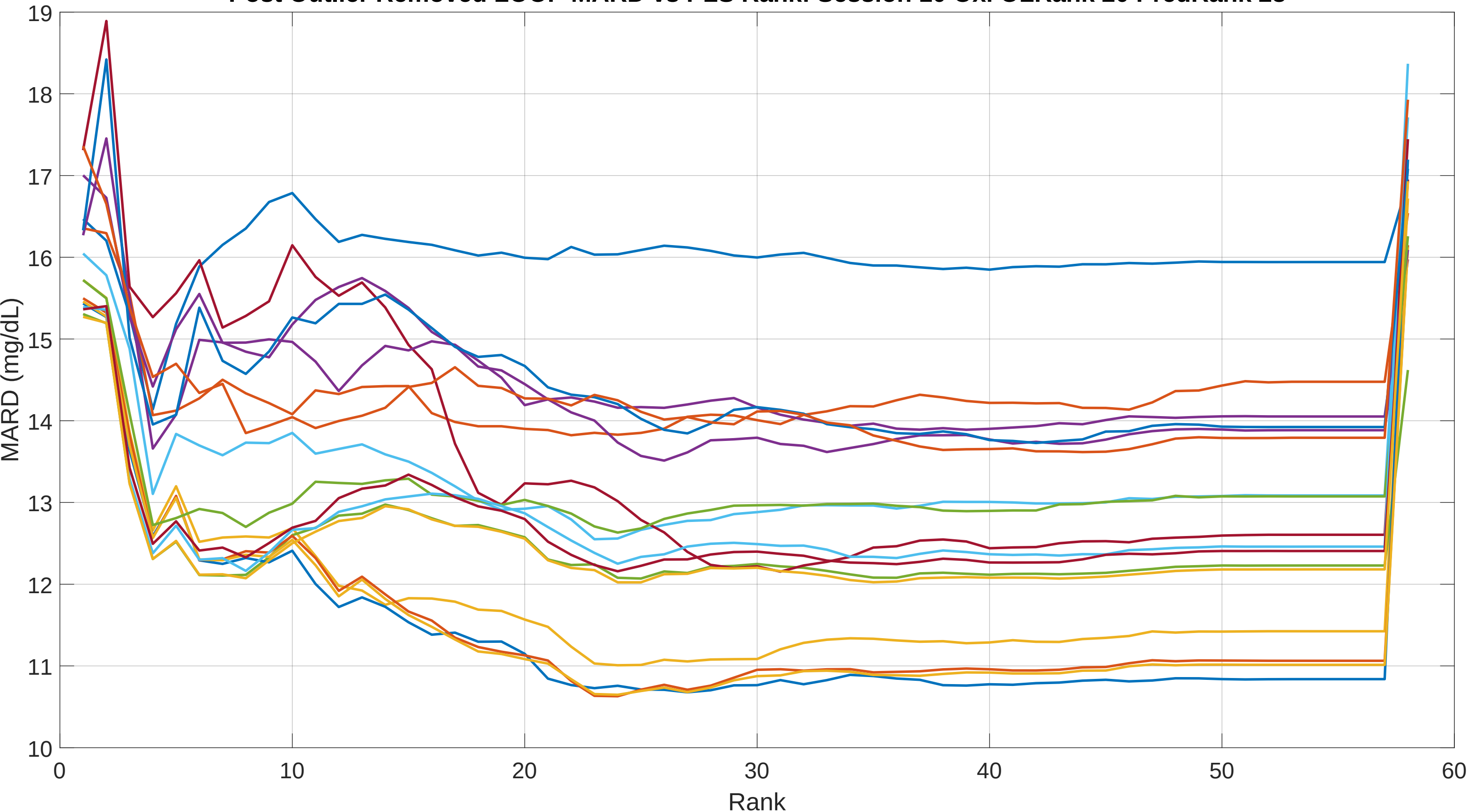
Post Outlier Removed LOOP MARD vs PLSRank: Session 10 Oxi OLRank 20 PredRank 28
