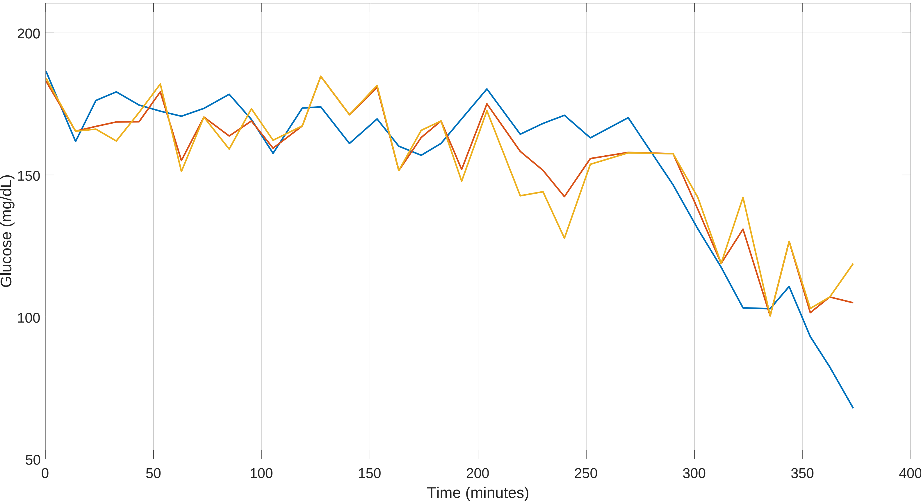
Post Outlier Removed LOOP vs Time: Outliers not in Predictions, Avg by Sitting, Session 10 Oxi OLRank 20 PredRank 28
