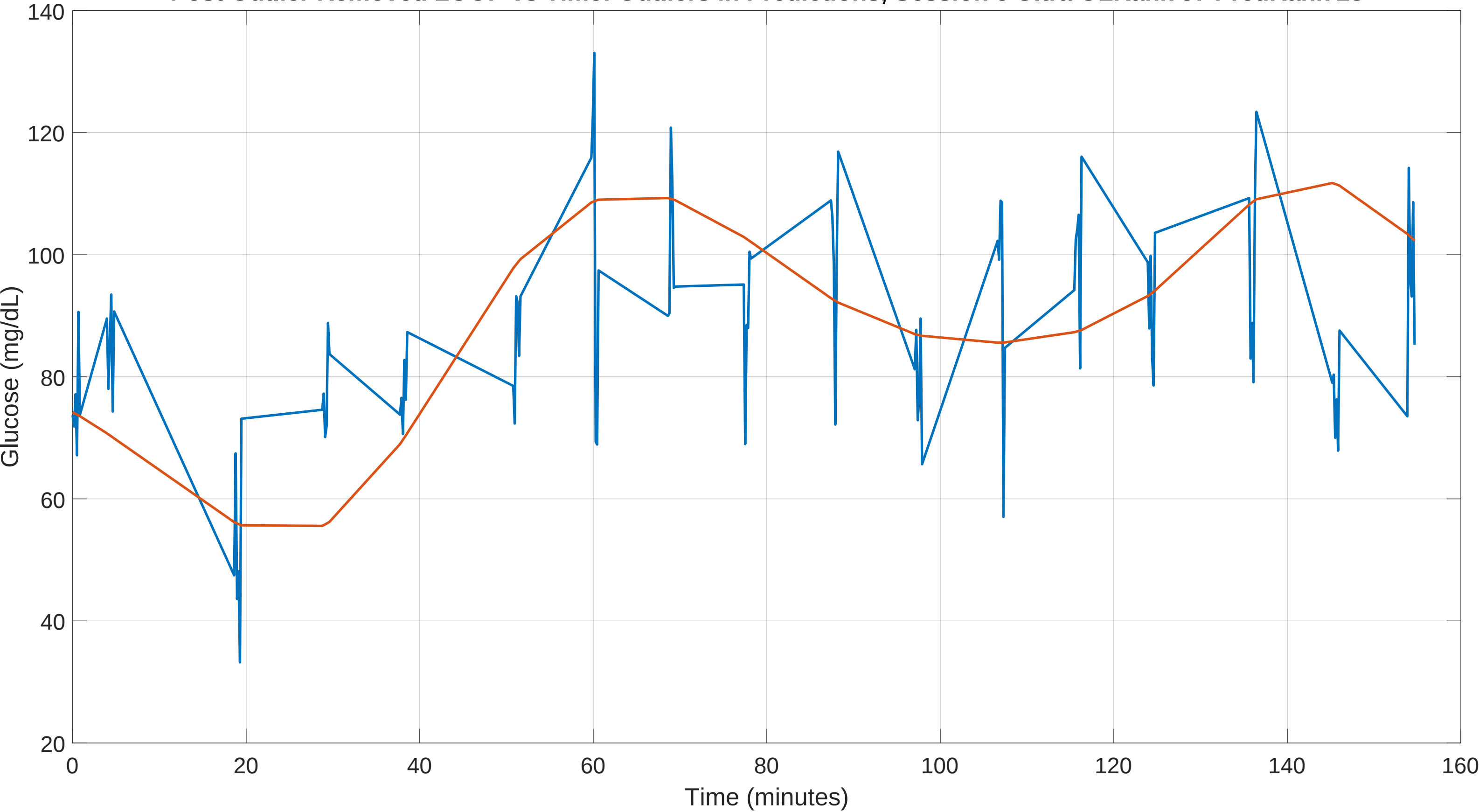
Post Outlier Removed LOOP vs Time: Outliers in Predictions, Session 5 Ultra OLRank 57 PredRank 28
