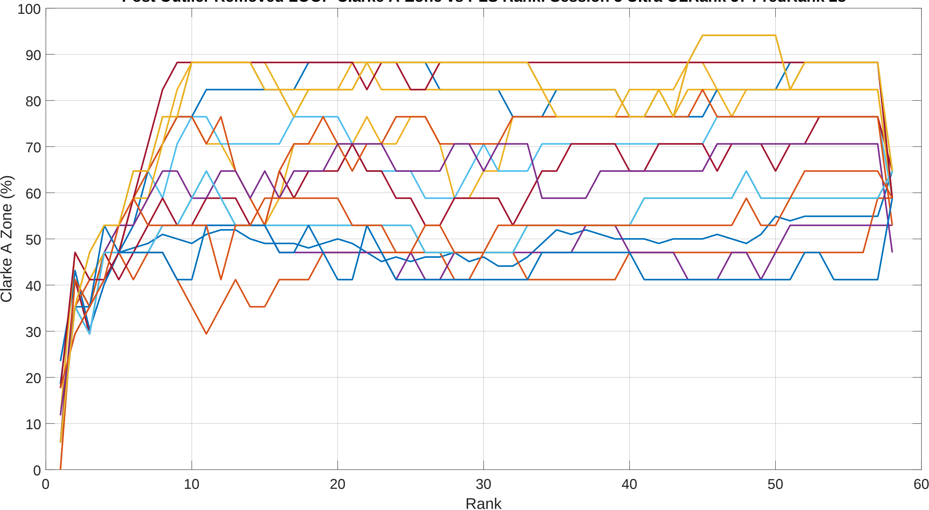
Post Outlier Removed LOOP Clarke A-Zone vs PLS Rank: Session 5 Ultra OLRank 57 PredRank 28
