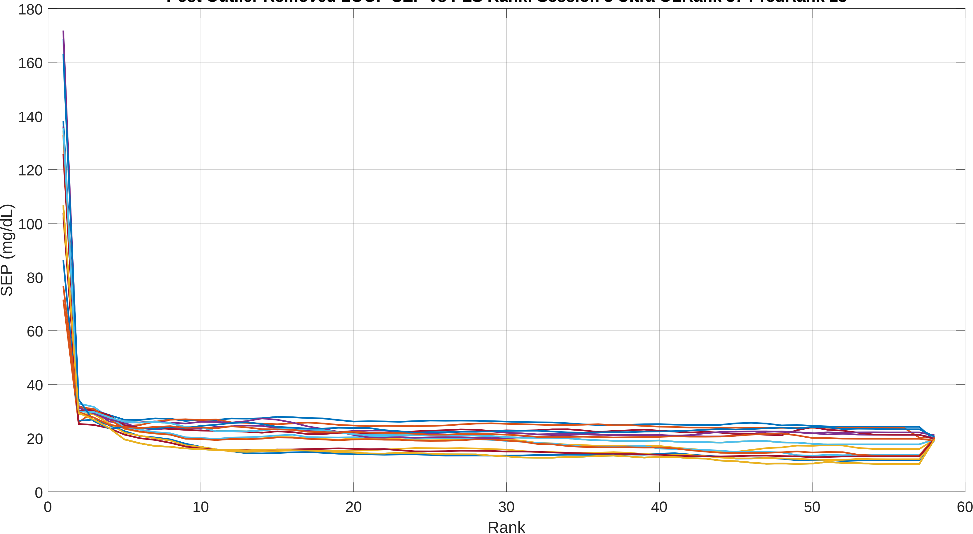
Post Outlier Removed LOOP SEP vs PLS Rank: Session 5 Ultra OLRank 57 PredRank 28
