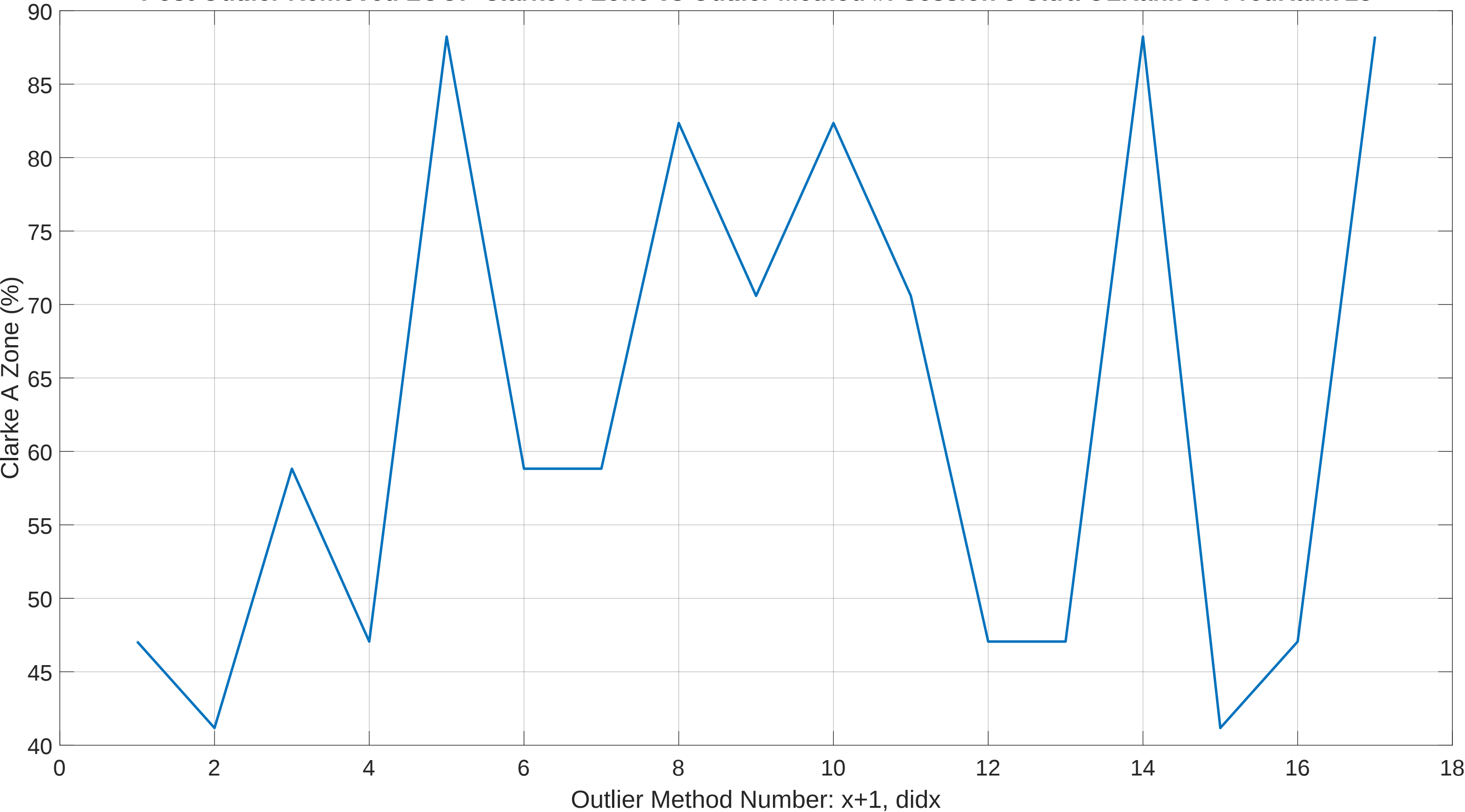
Post Outlier Removed LOOP Clarke A-Zone vs Outlier Method #: Session 5 Ultra OLRank 57 PredRank 28
