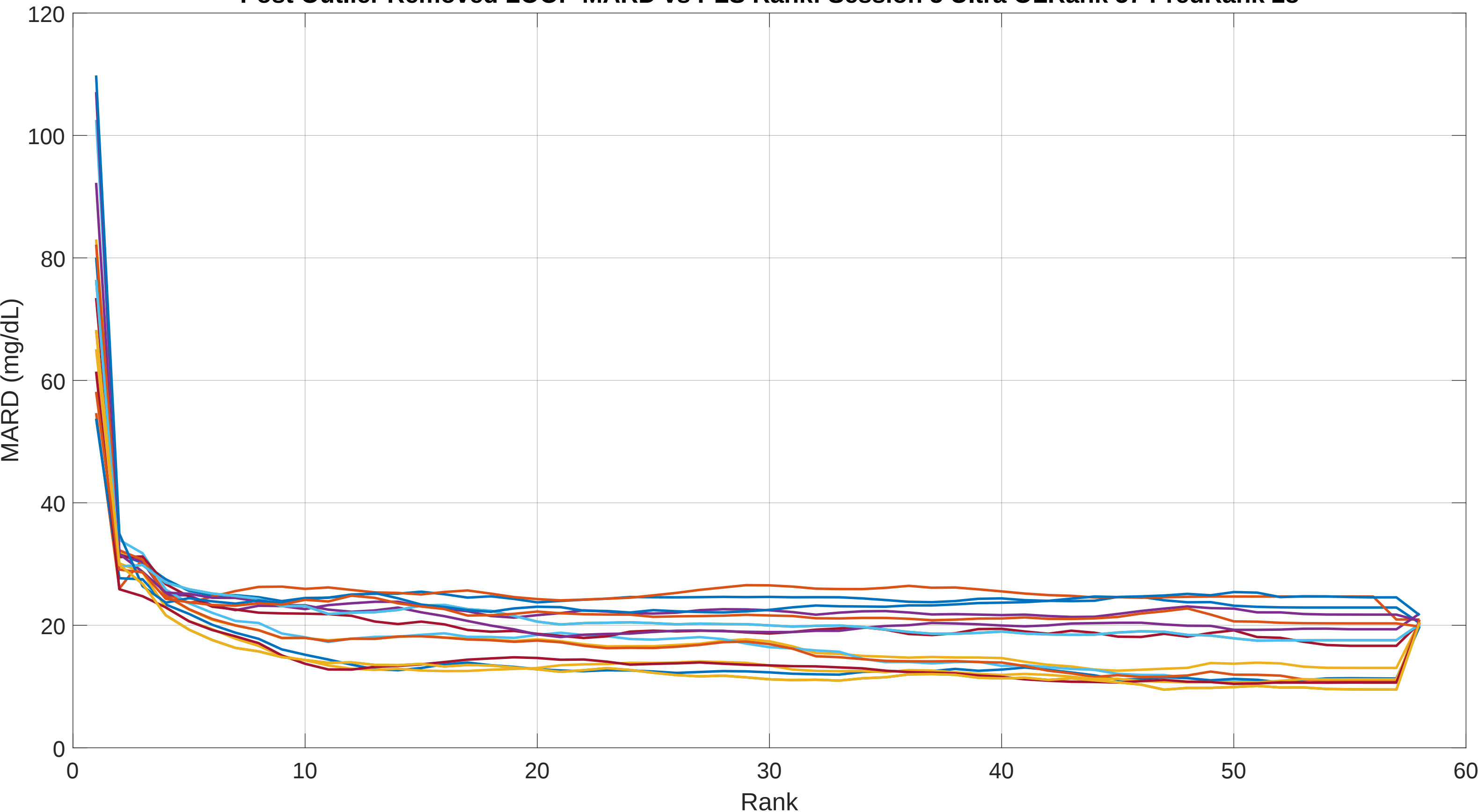
Post Outlier Removed LOOP MARD vs PLS Rank: Session 5 Ultra OLRank 57 PredRank 28
