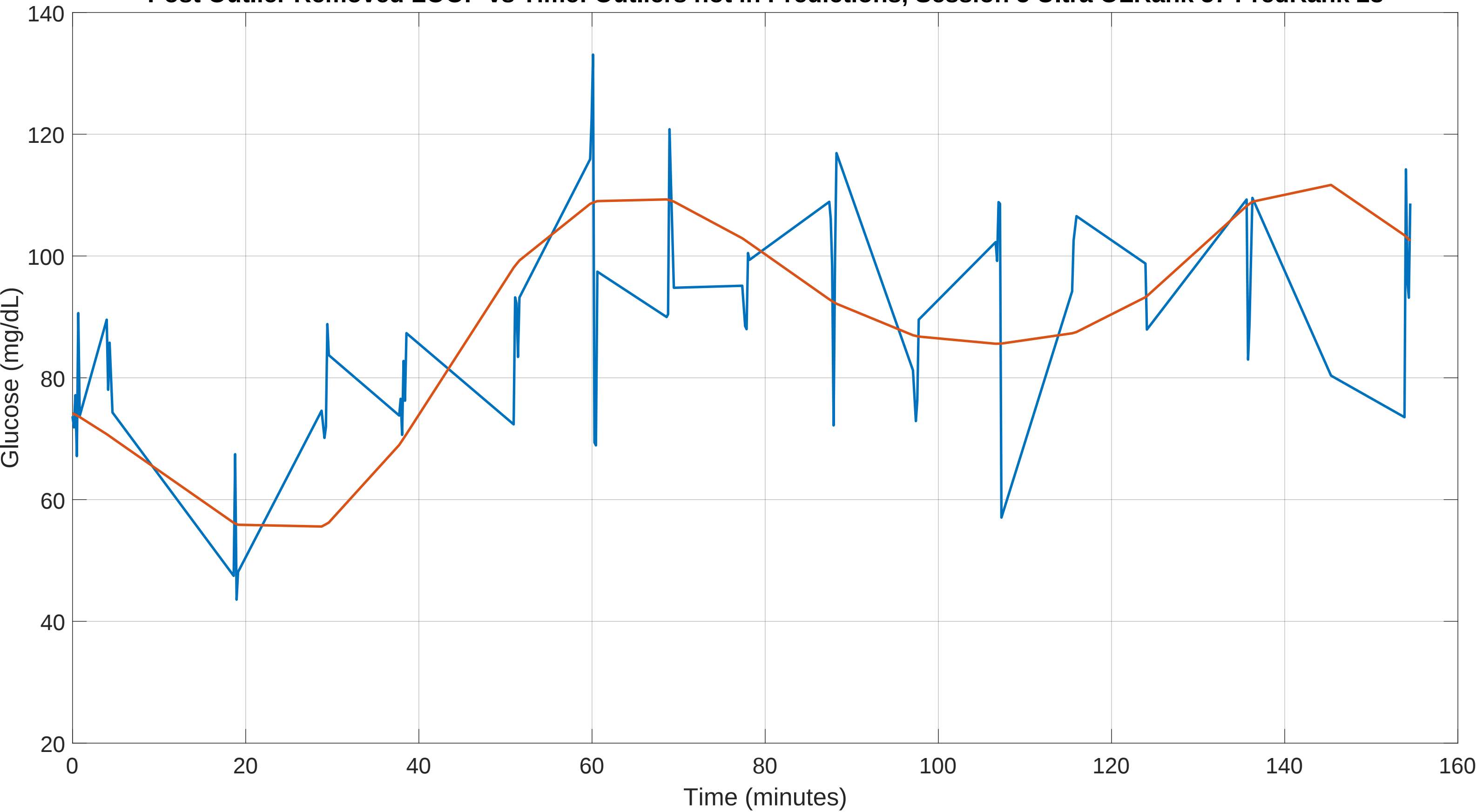
Post Outlier Removed LOOP vs Time: Outliers not in Predictions, Session 5 Ultra OLRank 57 PredRank 28
