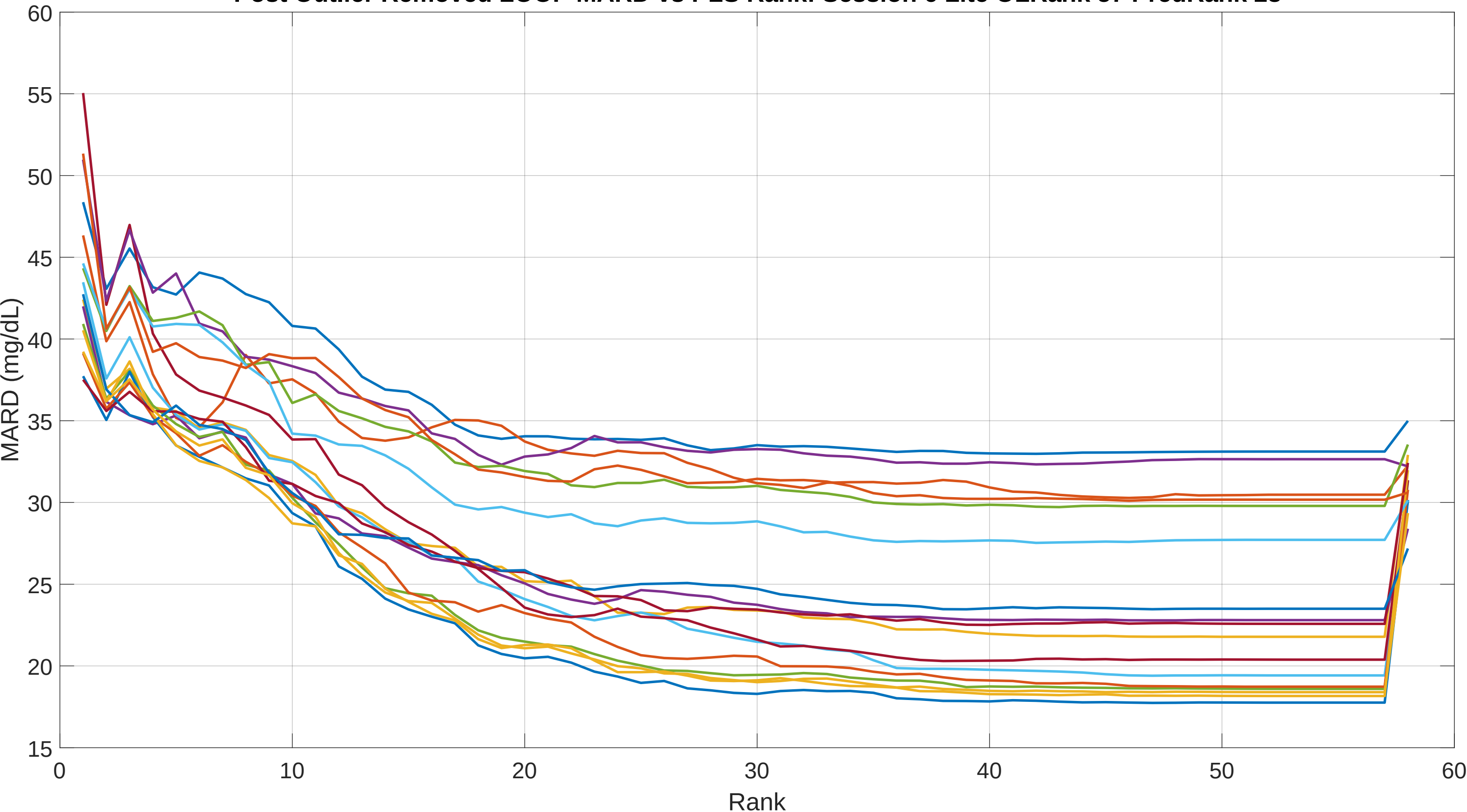
Post Outlier Removed LOOP MARD vs PLS Rank: Session 6 Lite OLRank 57 PredRank 28
