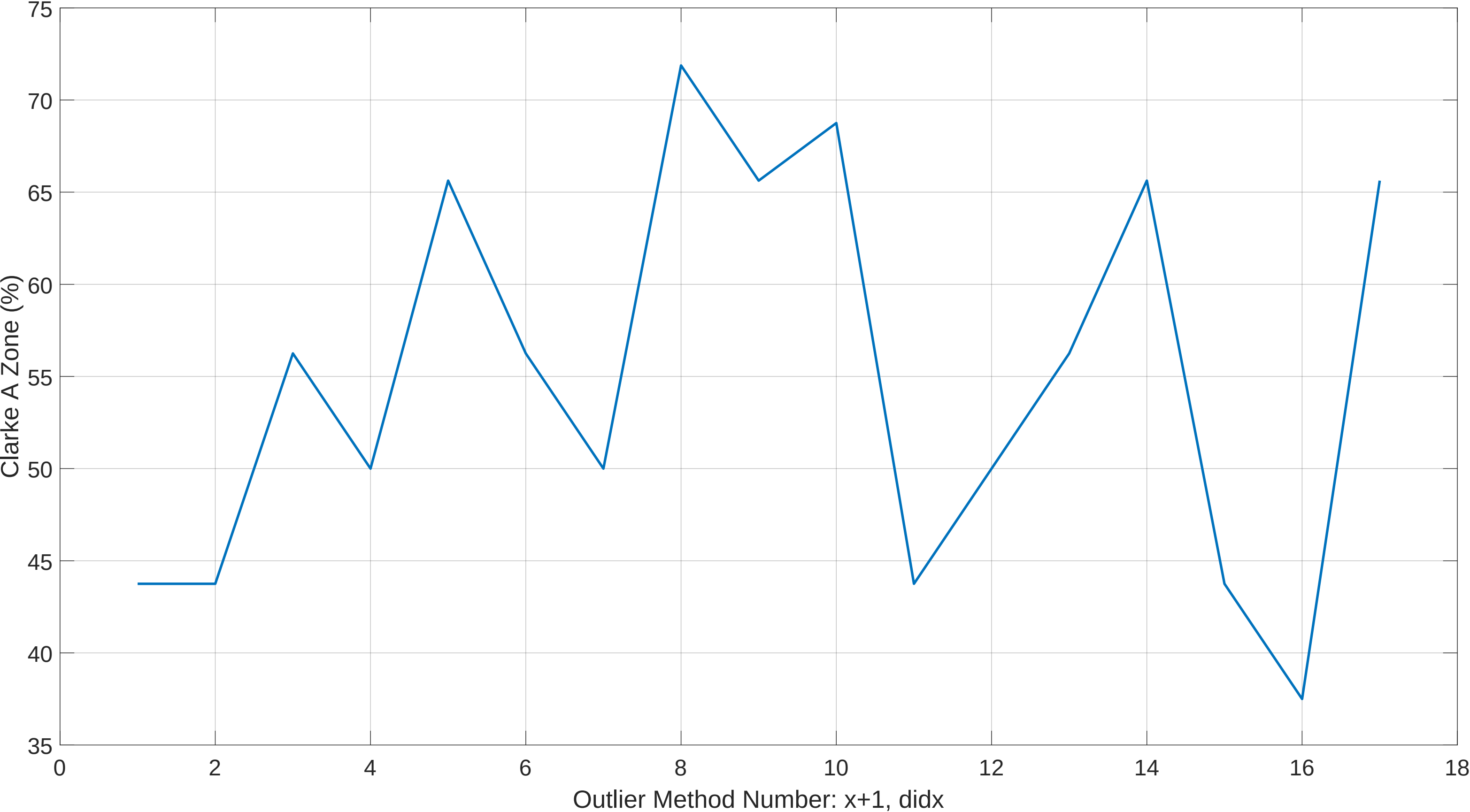
Post Outlier Removed LOOP Clarke A-Zone vs Outlier Method #: Session 6 Lite OLRank 57 PredRank 28
