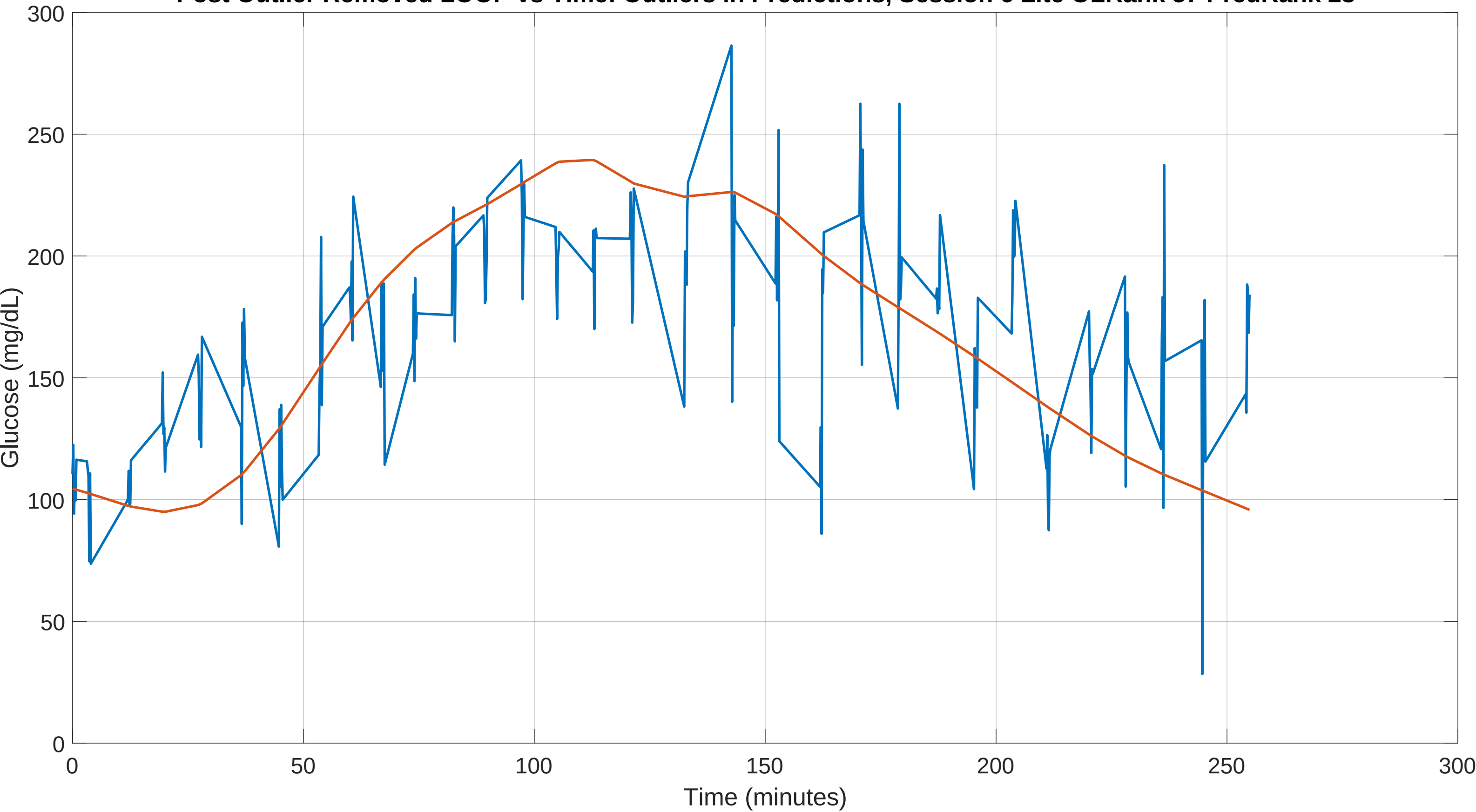
Post Outlier Removed LOOP vs Time: Outliers in Predictions, Session 6 Lite OLRank 57 PredRank 28
