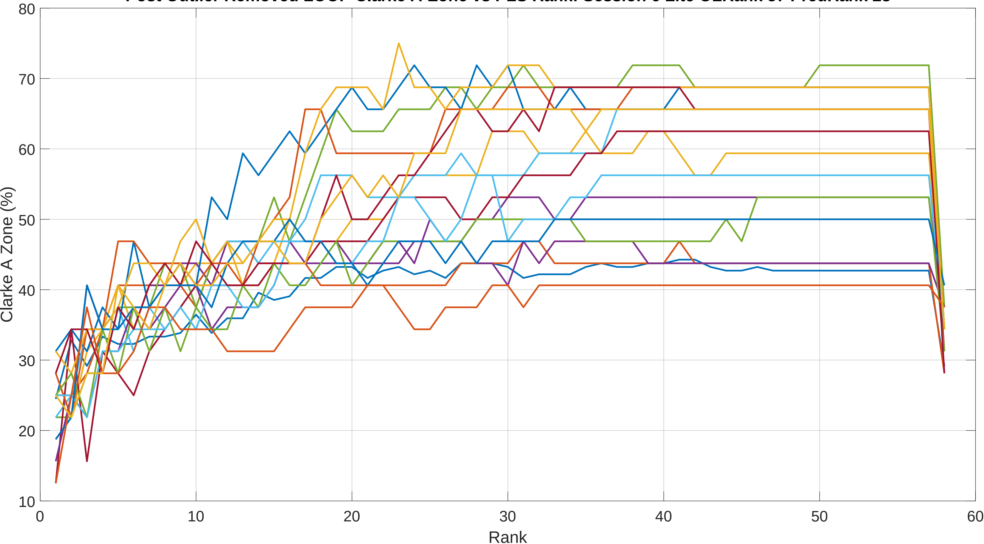
Post Outlier Removed LOOP Clarke A-Zone vs PLS Rank: Session 6 Lite OLRank 57 PredRank 28
