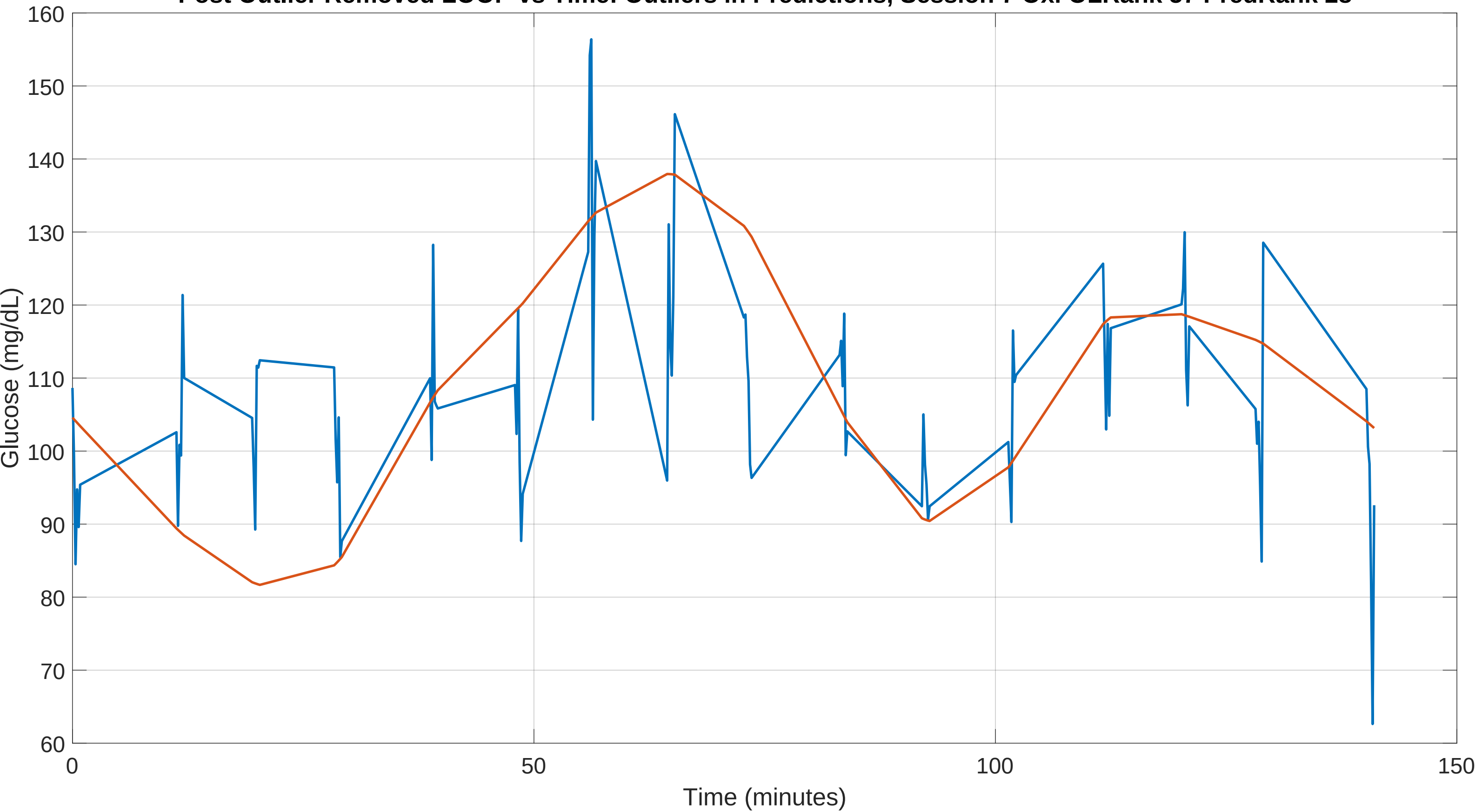
Post Outlier Removed LOOP vs Time: Outliers in Predictions, Session 7 Oxi OLRank 57 PredRank 28
