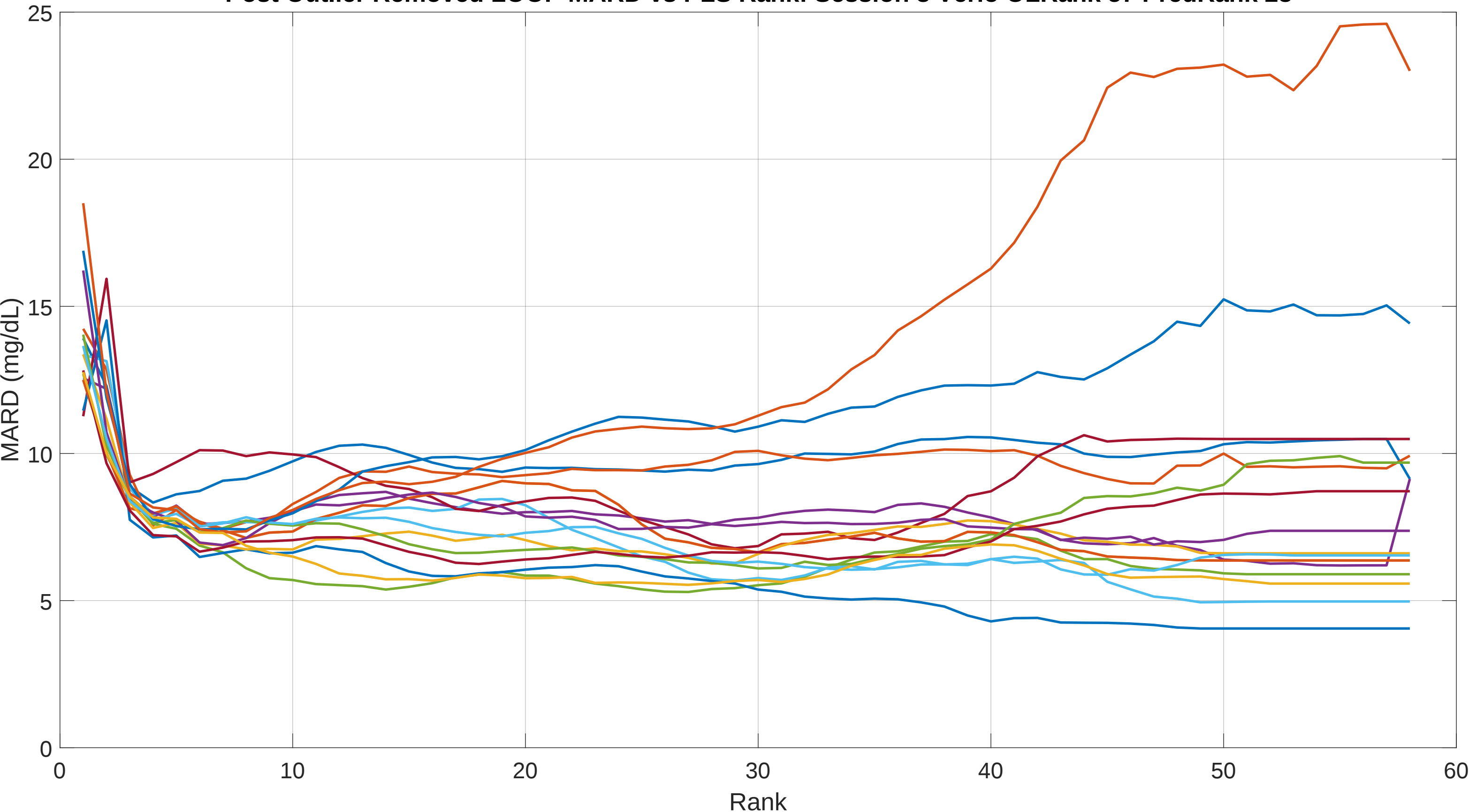
Post Outlier Removed LOOP MARD vs PLS Rank: Session 8 Verio OLRank 57 PredRank 28
