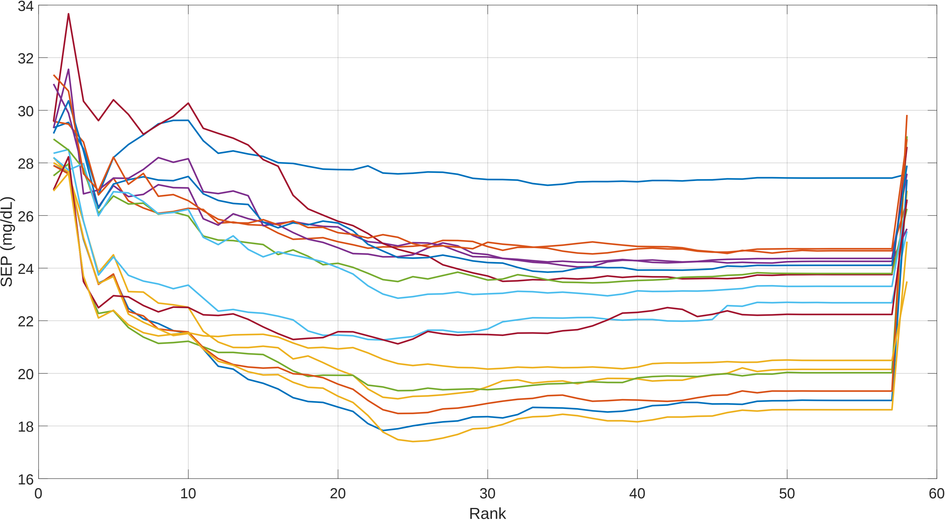
Post Outlier Removed LOOP SEP vs PLS Rank: Session 10 Oxi OLRank 57 PredRank 28
