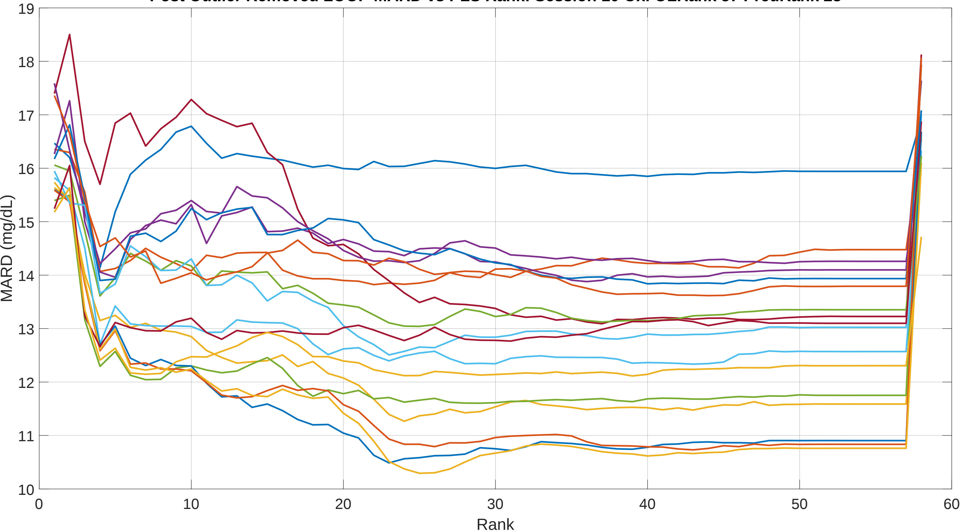
Post Outlier Removed LOOP MARD vs PLSRank: Session 10 Oxi OLRank 57 PredRank 28
