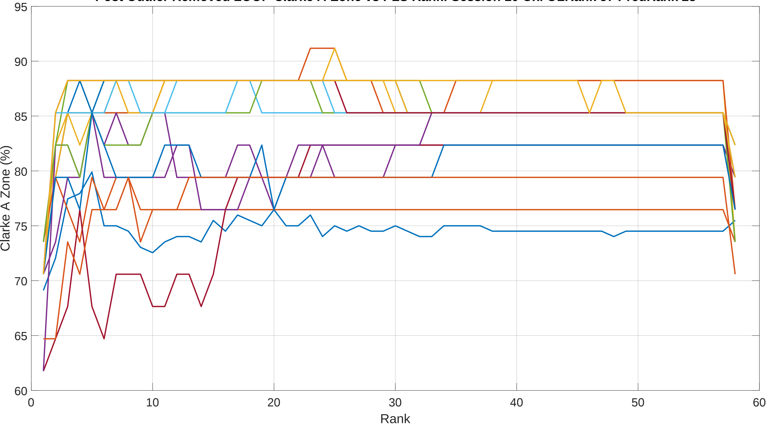
Post Outlier Removed LOOP Clarke A-Zone vs PLS Rank: Session 10 Oxi OLRank 57 PredRank 28
