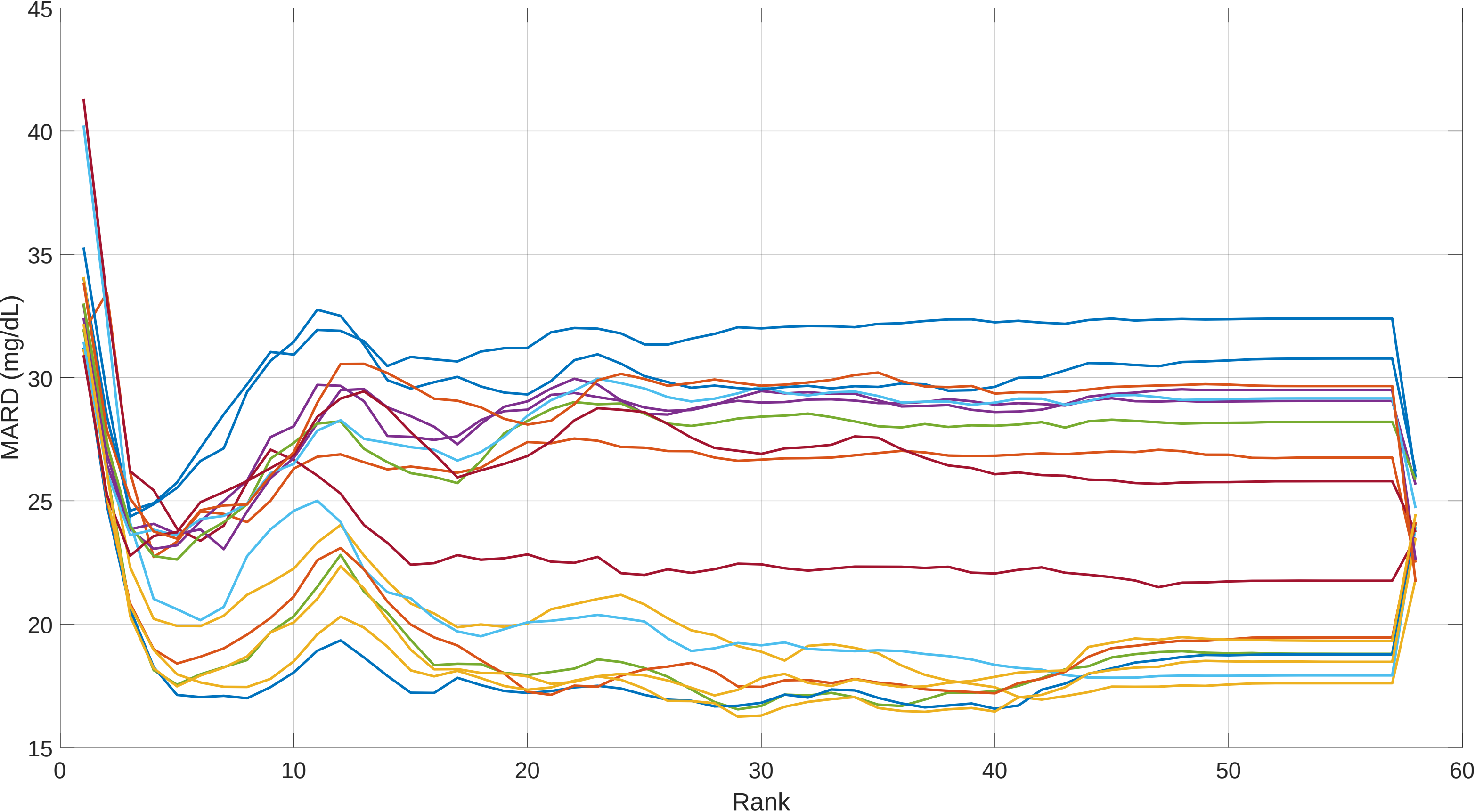
Post Outlier Removed LOOP MARD vs PLS Rank: Session 13 Verio OLRank 57 PredRank 28
