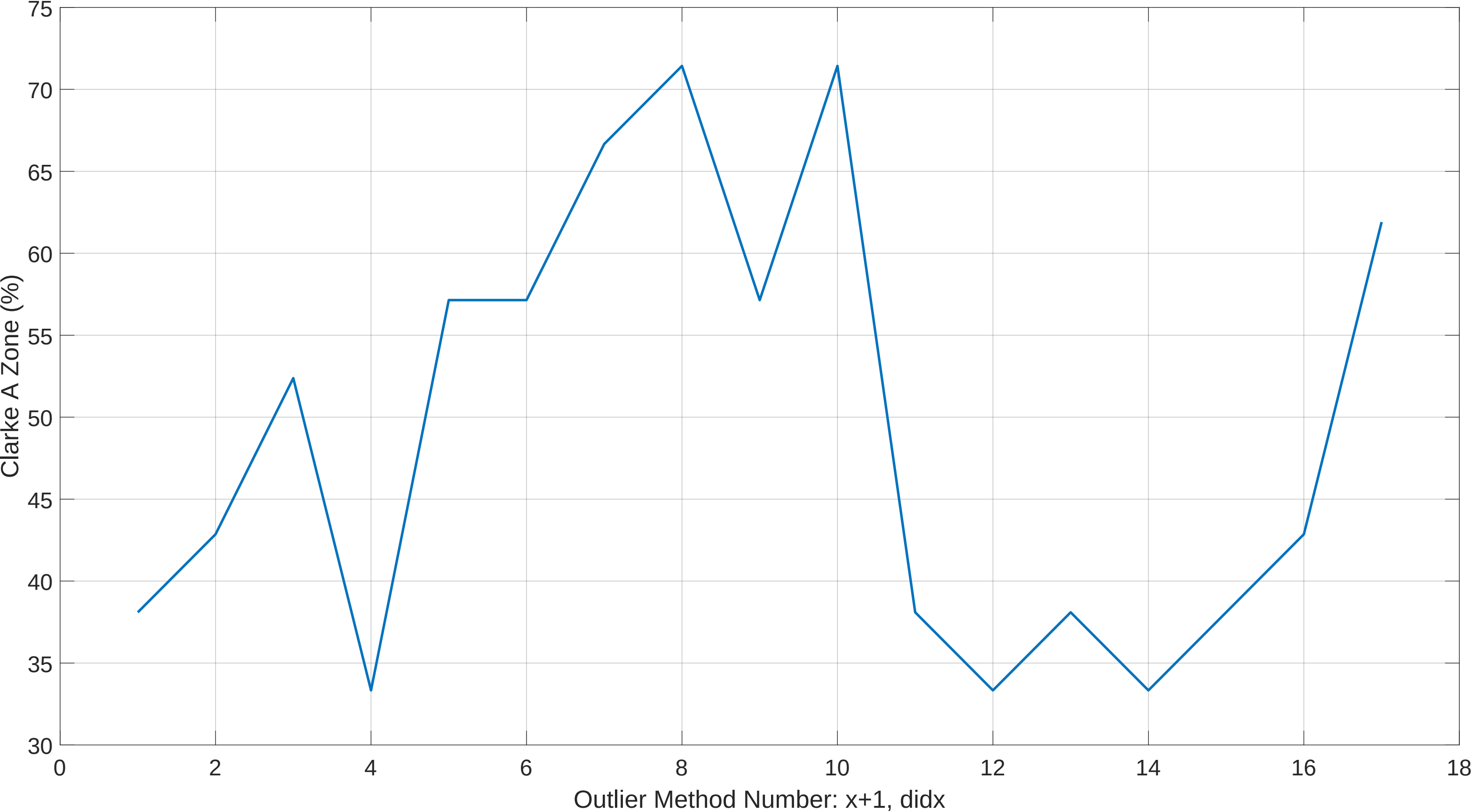
Post Outlier Removed LOOP Clarke A-Zone vs Outlier Method #: Session 13 Verio OLRank 57 PredRank 28
