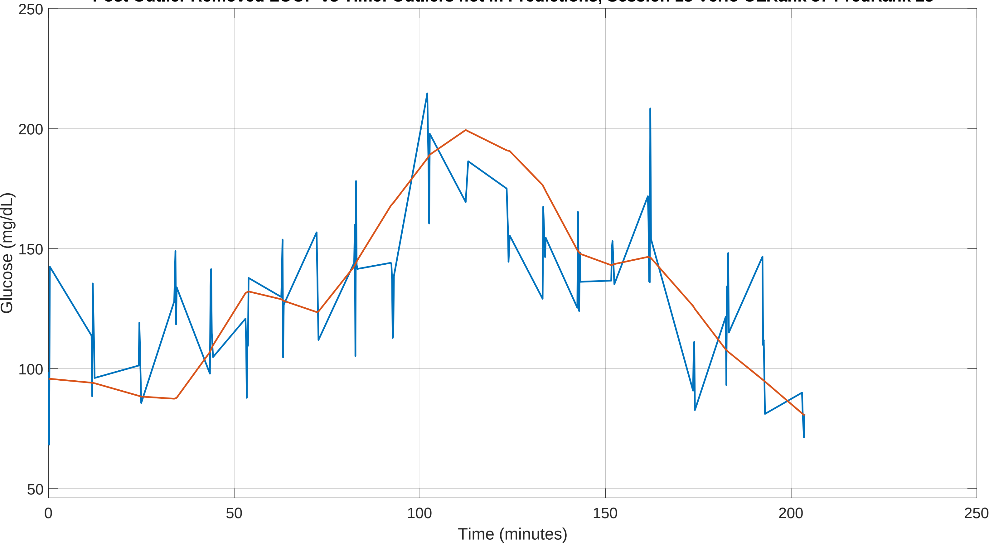
Post Outlier Removed LOOP vs Time: Outliers not in Predictions, Session 13 Verio OLRank 57 PredRank 28
